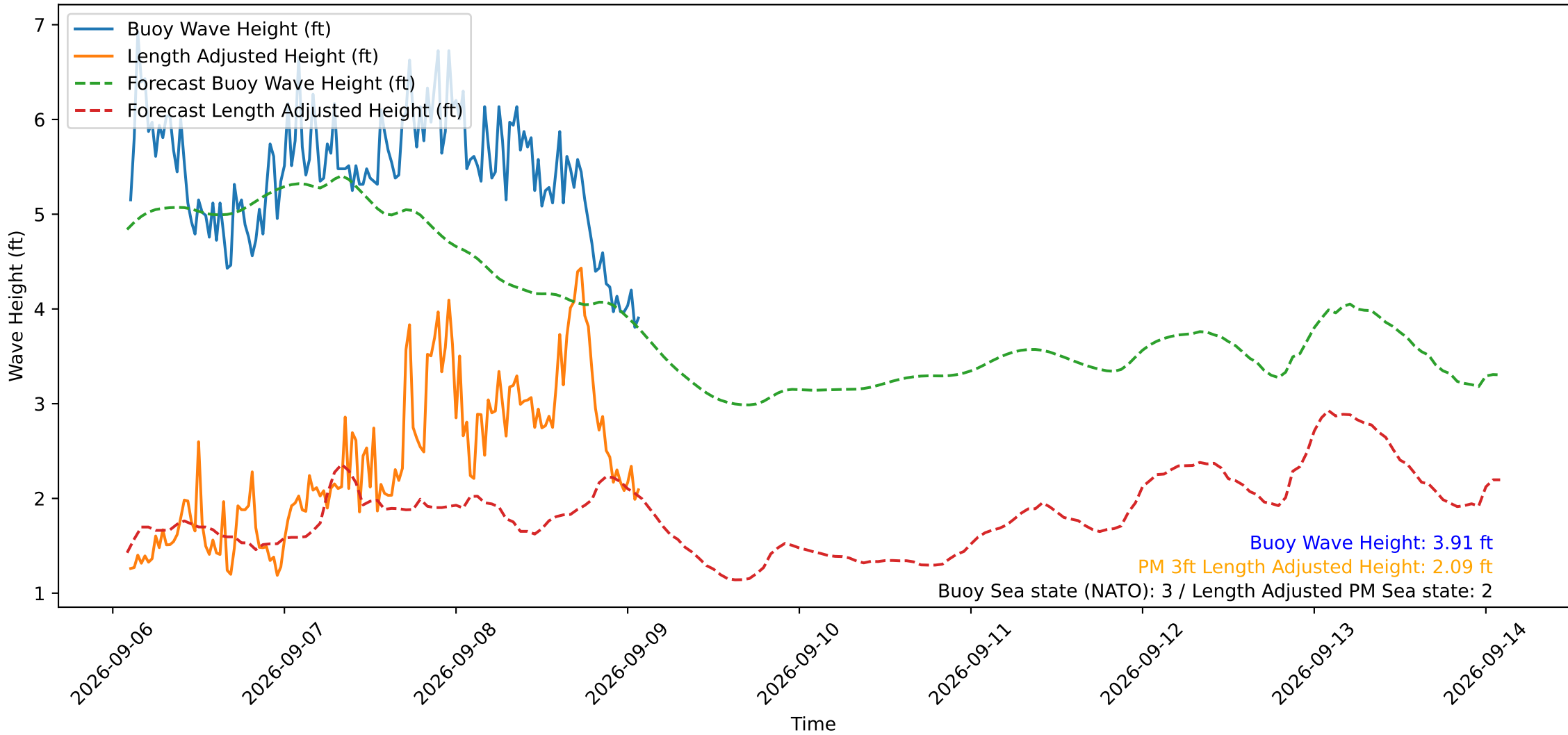
Wave Heights over Time for Red Beach at 2026-09-09 02:20:51
