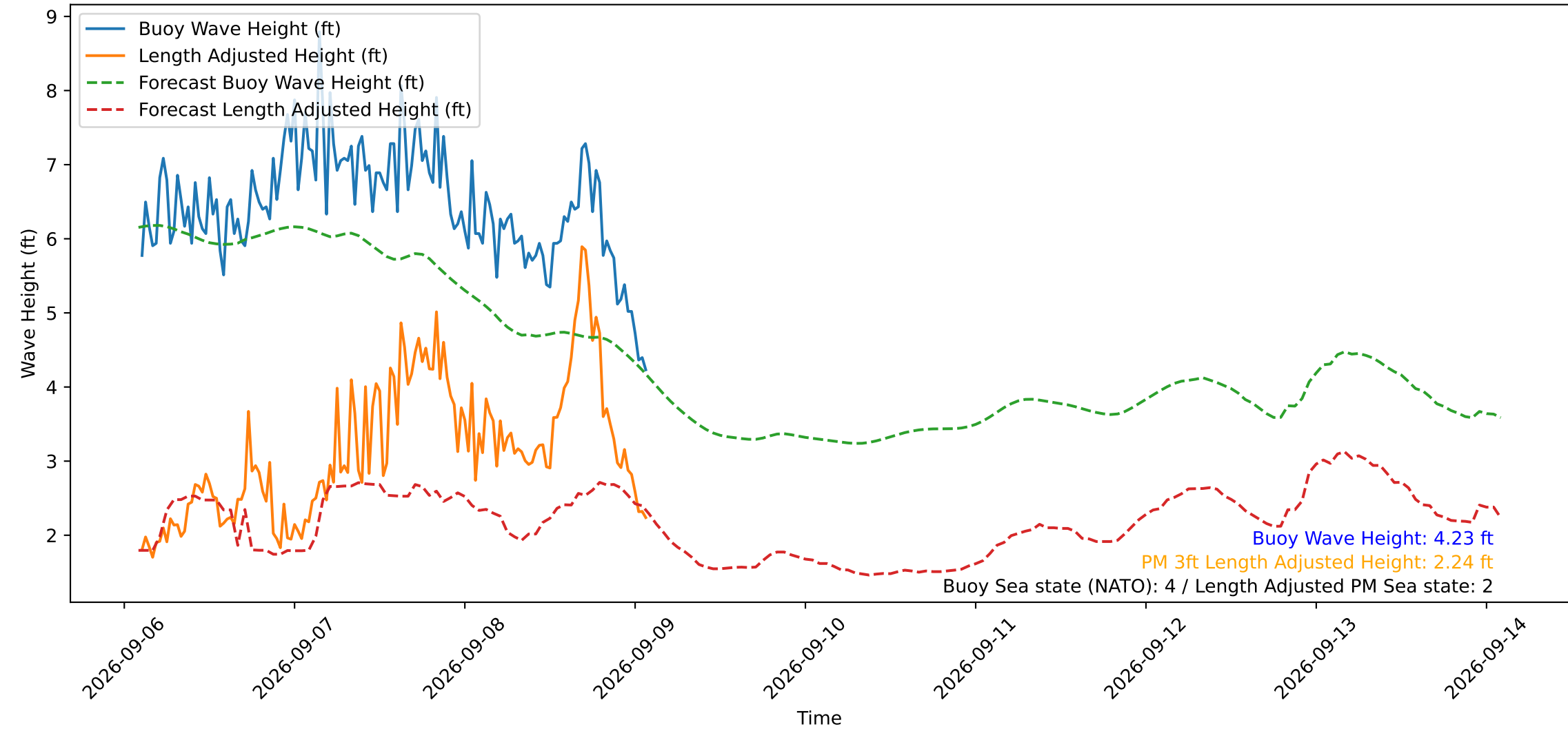
Wave Heights over Time for Green Beach at 2026-09-09 02:21:16
