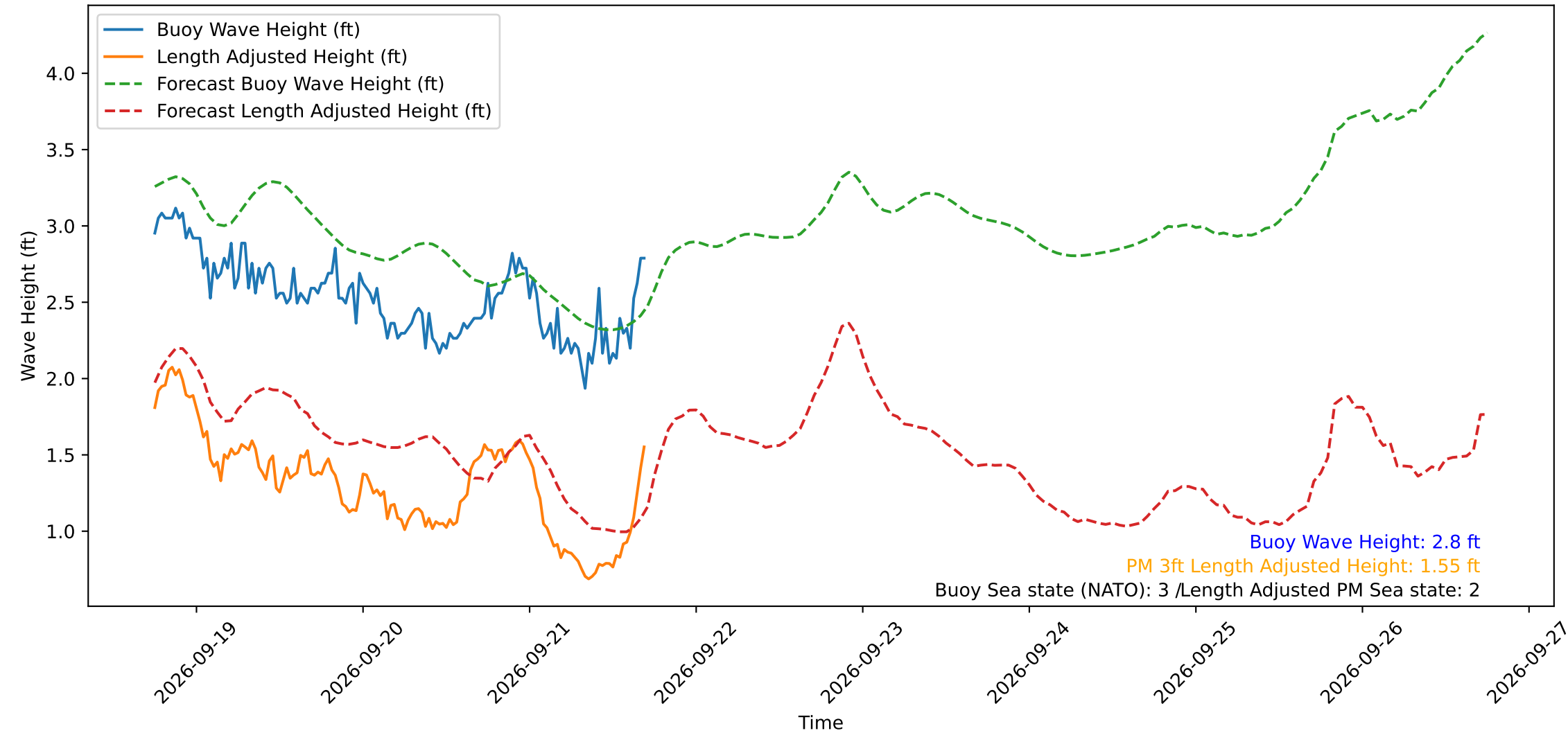
Wave Heights over Time for Green Beach at 2026-09-21 17:51:14
