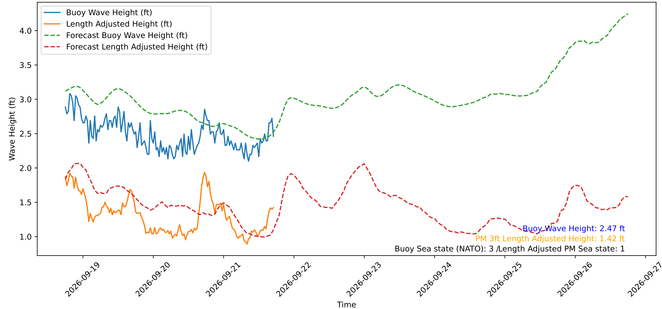
Wave Heights over Time for Oceanside Harbor at 2026-09-21 17:50:29
