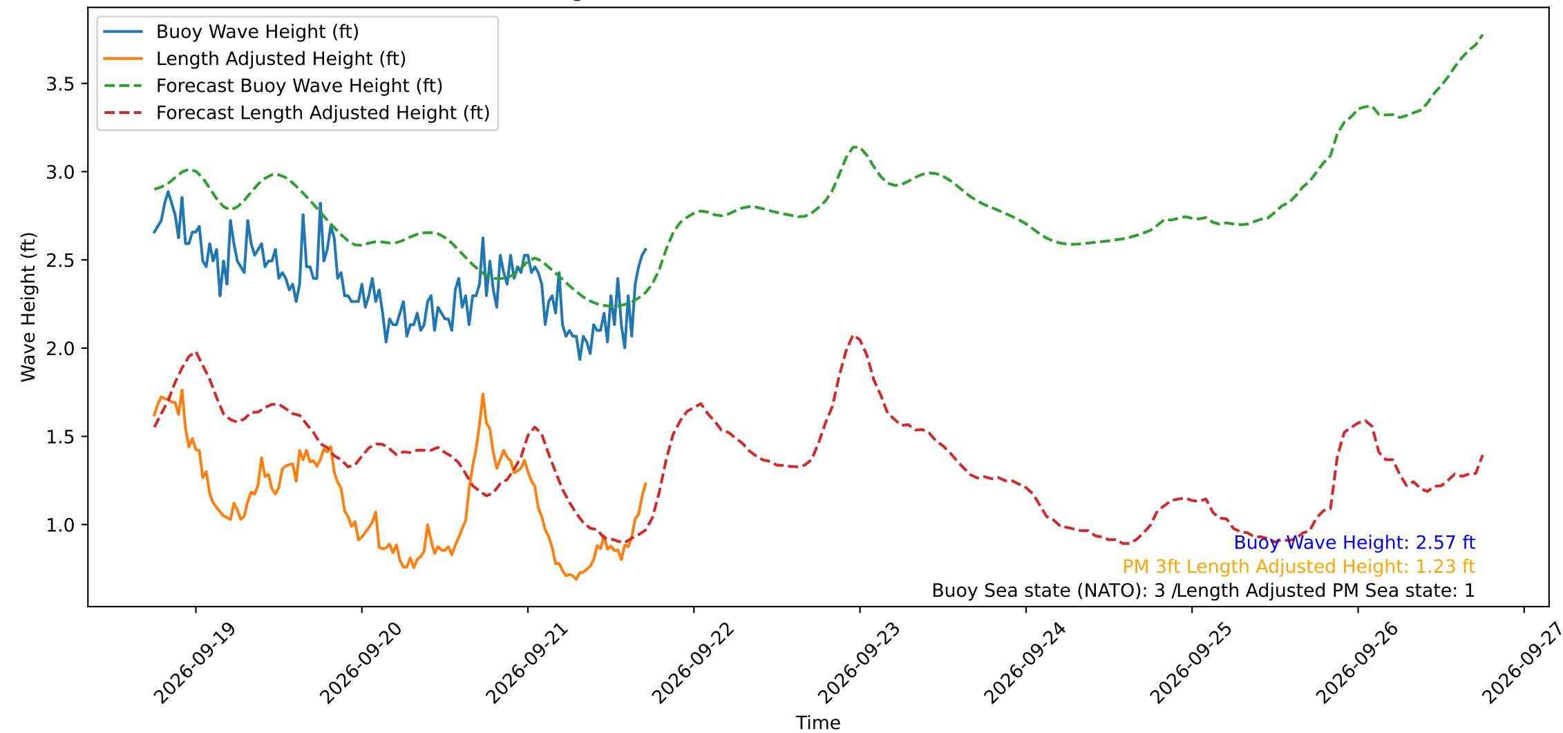
Wave Heights over Time for Red Beach at 2026-09-21 17:50:50
