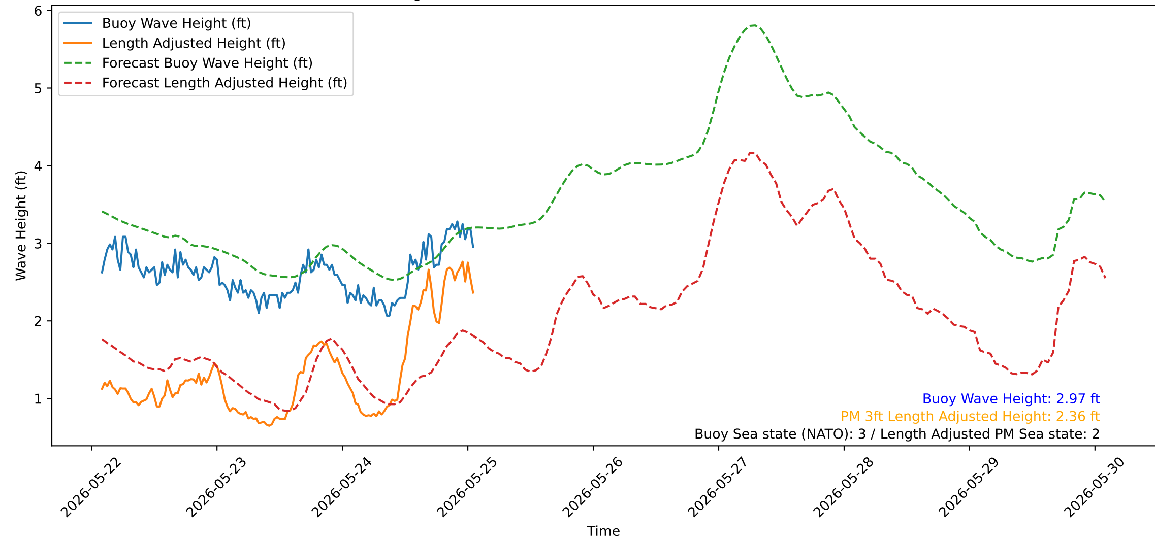
Wave Heights over Time for Green Beach at 2026-05-25 02:01:13
