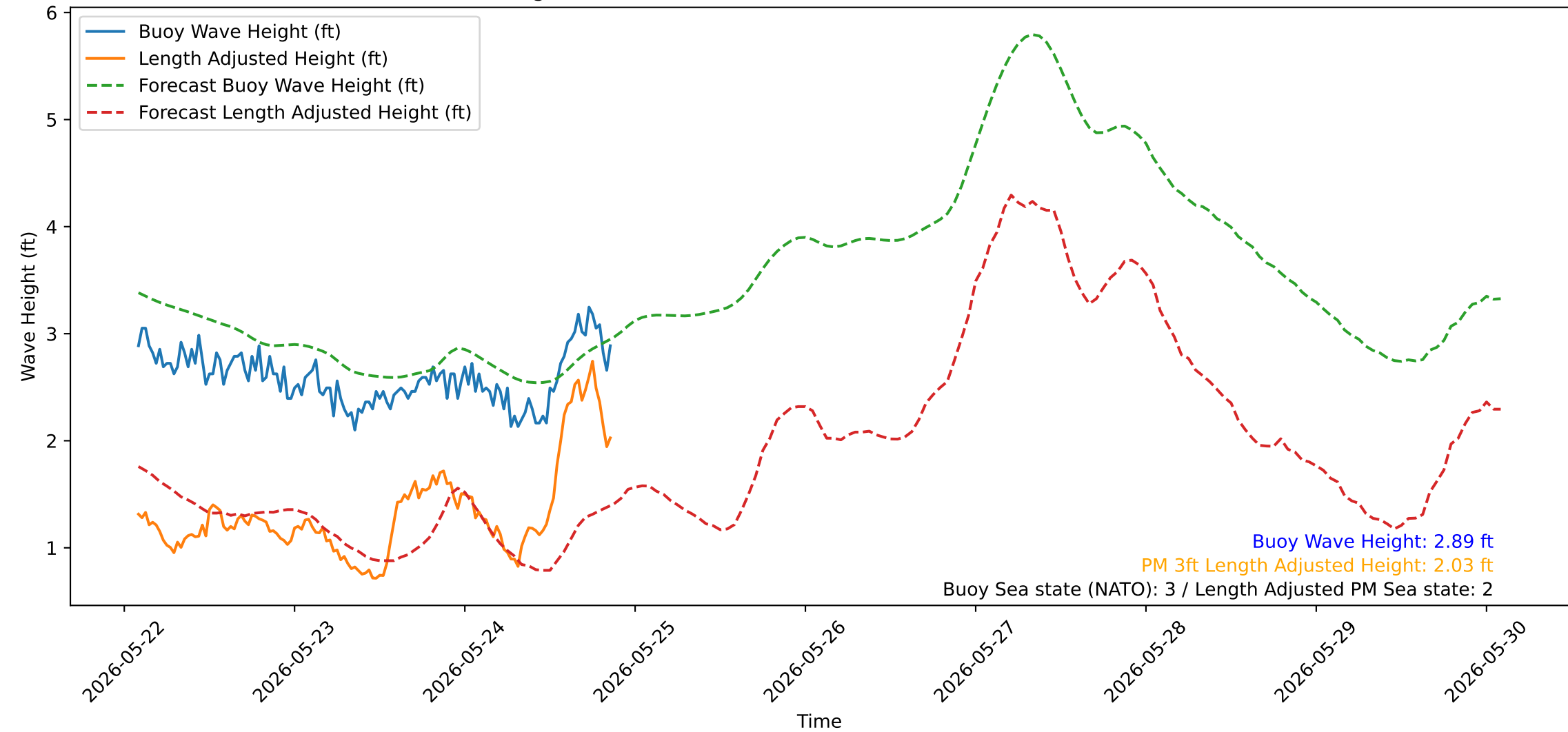
Wave Heights over Time for Oceanside Harbor at 2026-05-25 02:00:31
