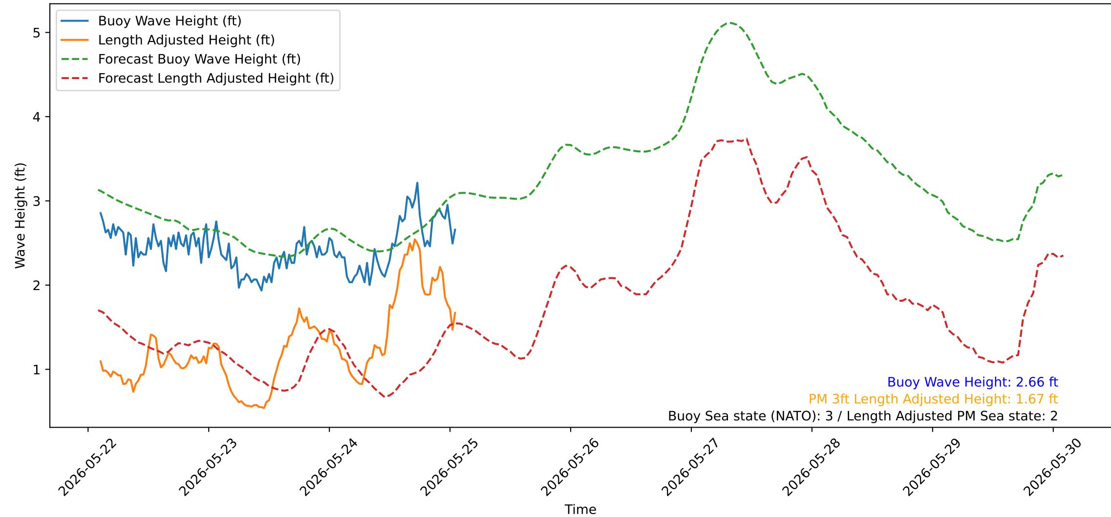
Wave Heights over Time for Red Beach at 2026-05-25 02:00:51
