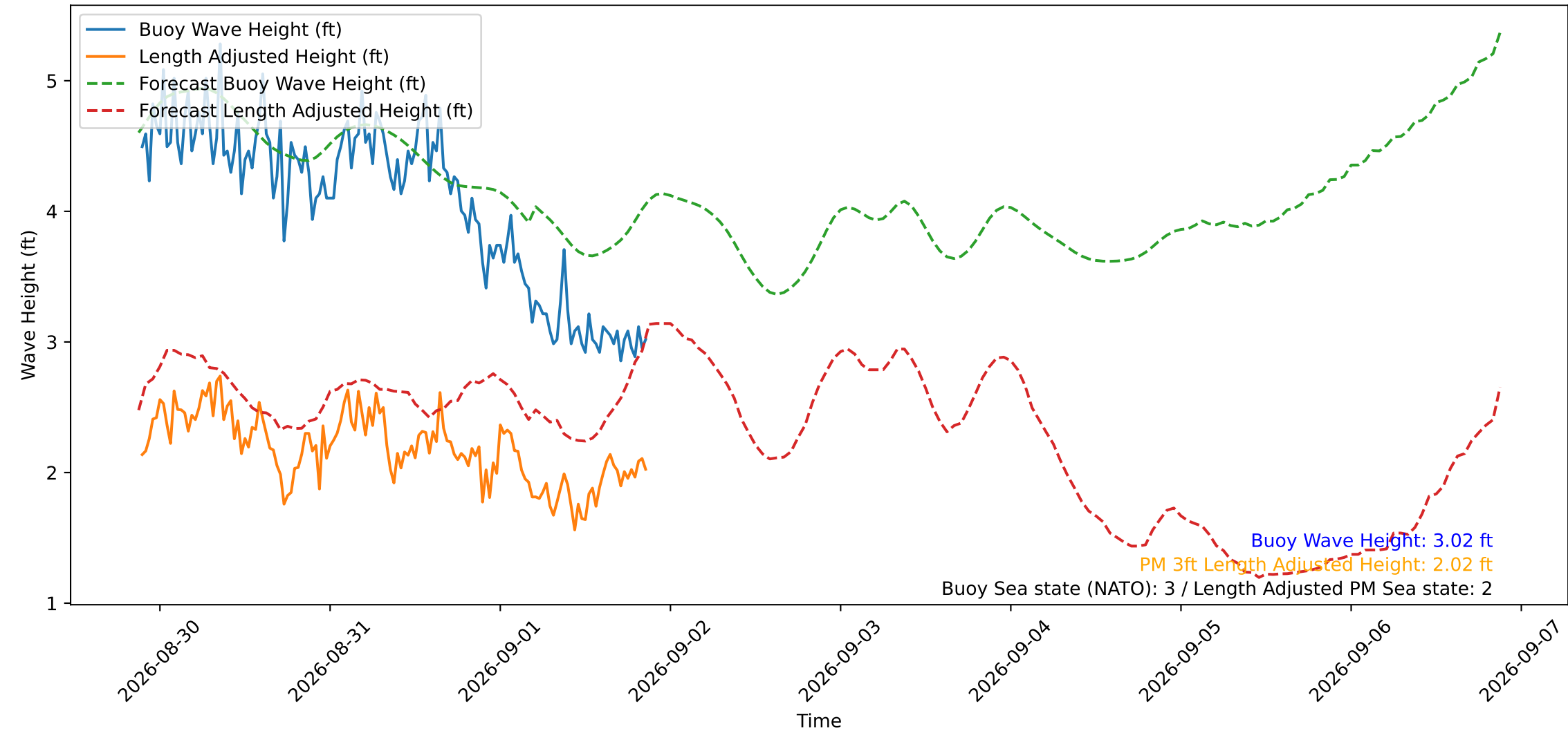
Wave Heights over Time for Oceanside Harbor at 2026-09-01 21:20:30
