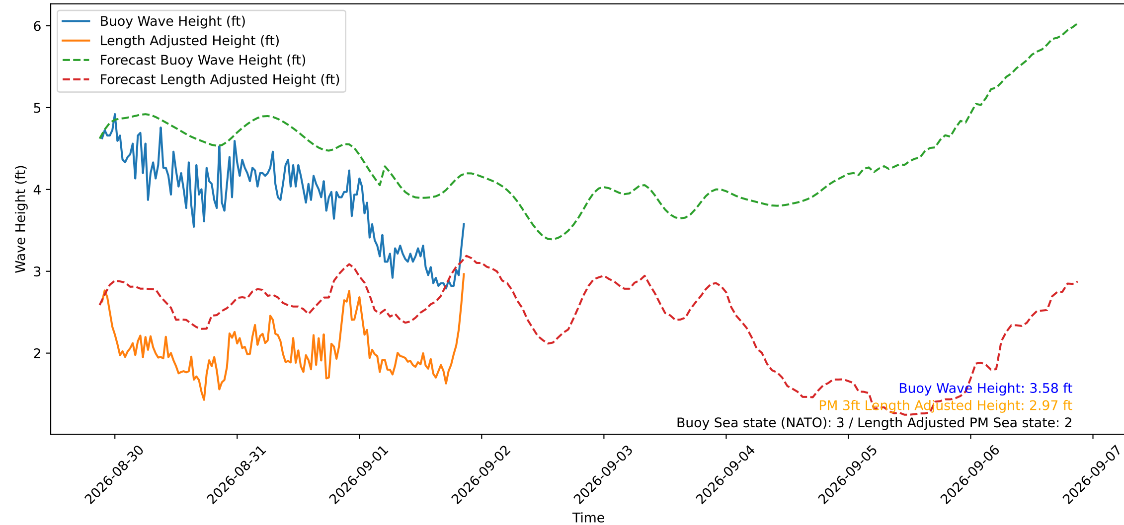
Wave Heights over Time for Green Beach at 2026-09-01 21:21:15
