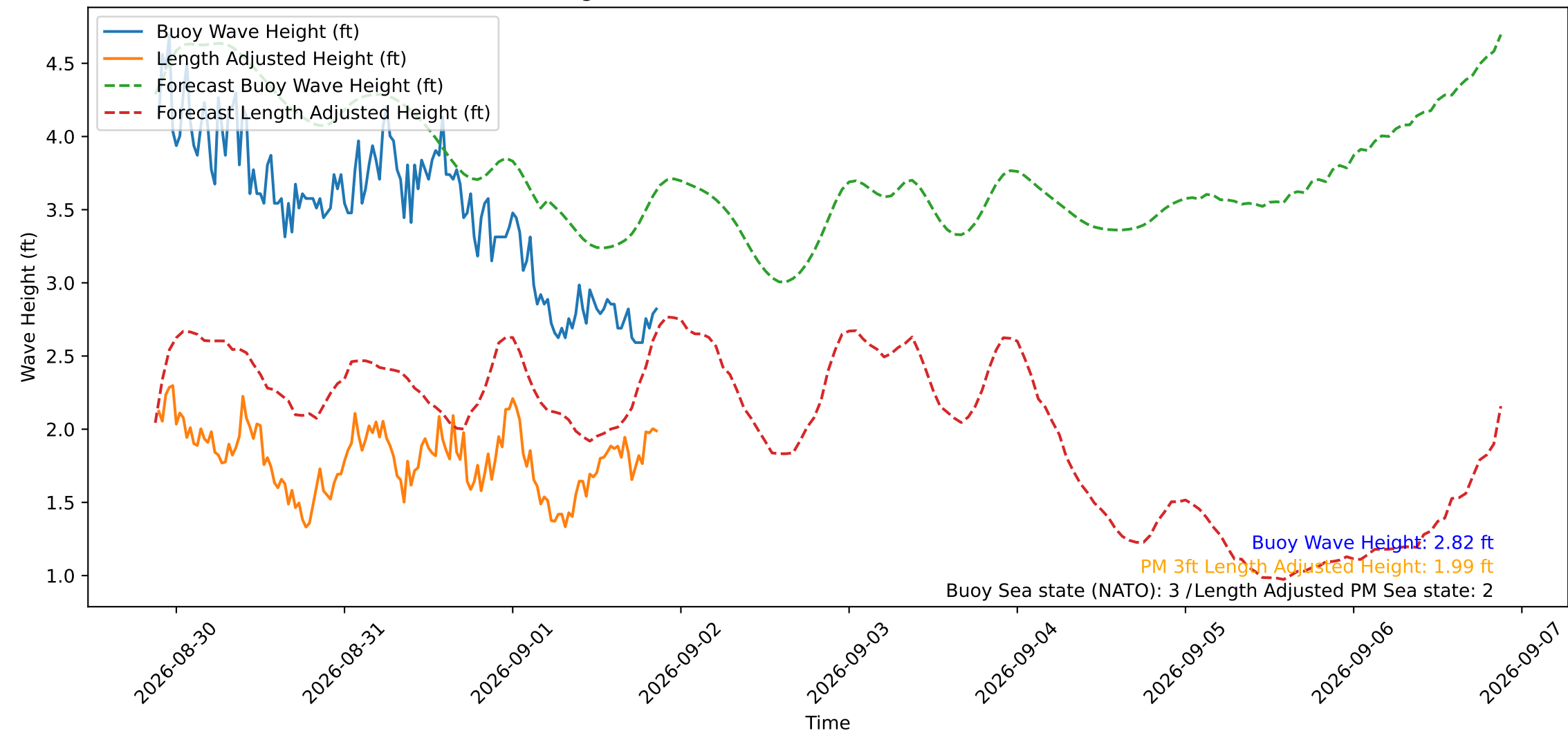
Wave Heights over Time for Red Beach at 2026-09-01 21:20:51
