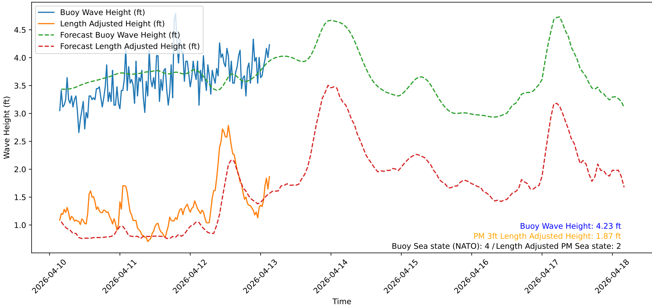
Wave Heights over Time for Oceanside Harbor at 2026-04-13 03:40:31
