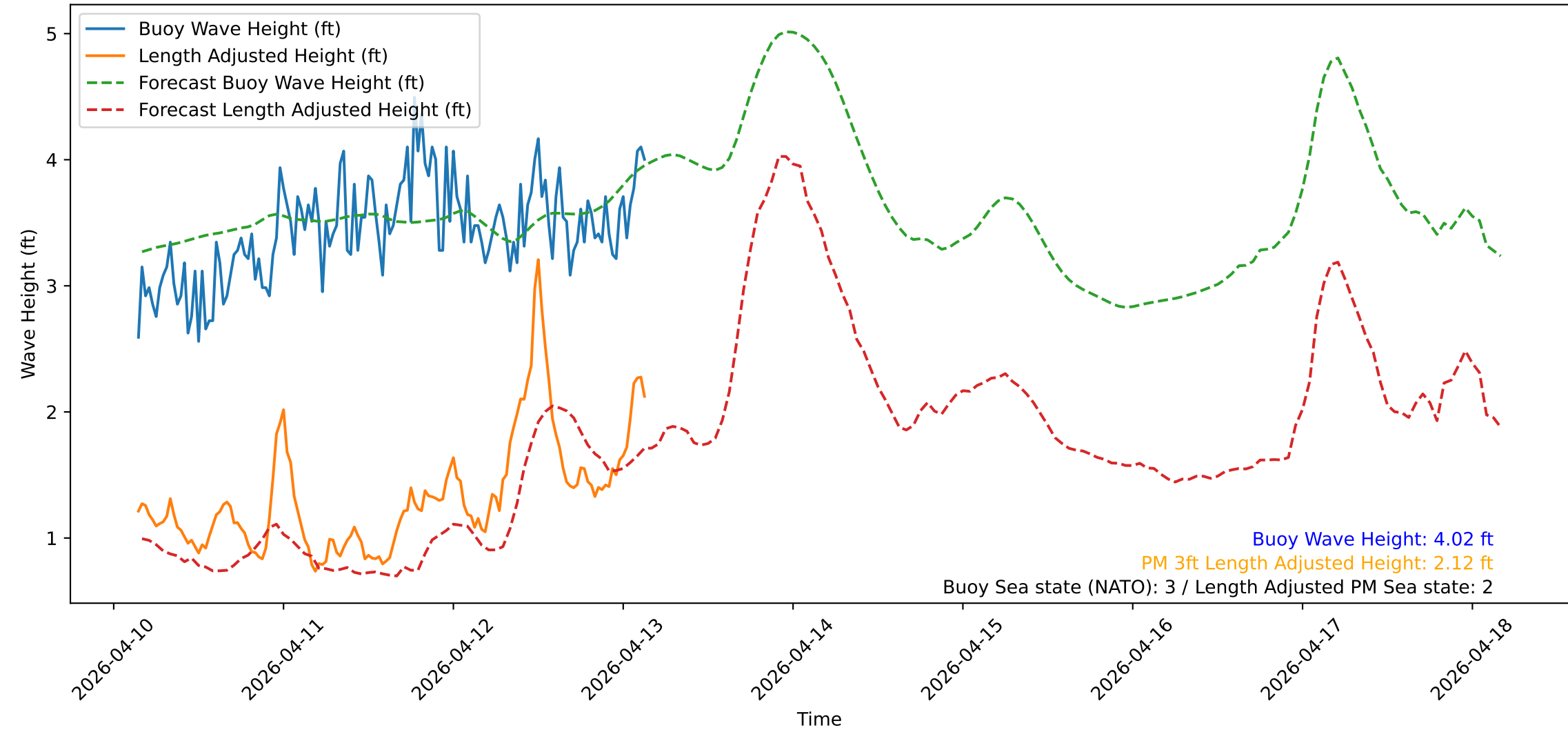
Wave Heights over Time for Green Beach at 2026-04-13 03:41:12
