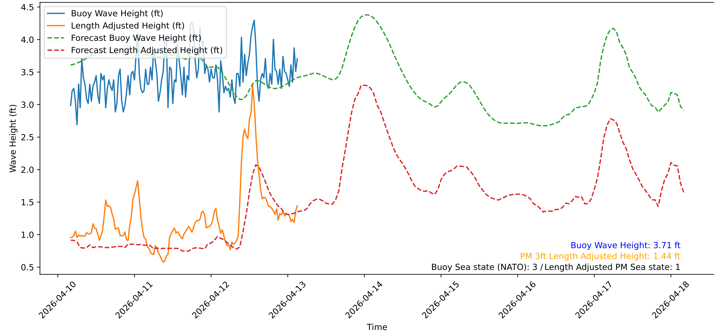
Wave Heights over Time for Red Beach at 2026-04-13 03:40:50
