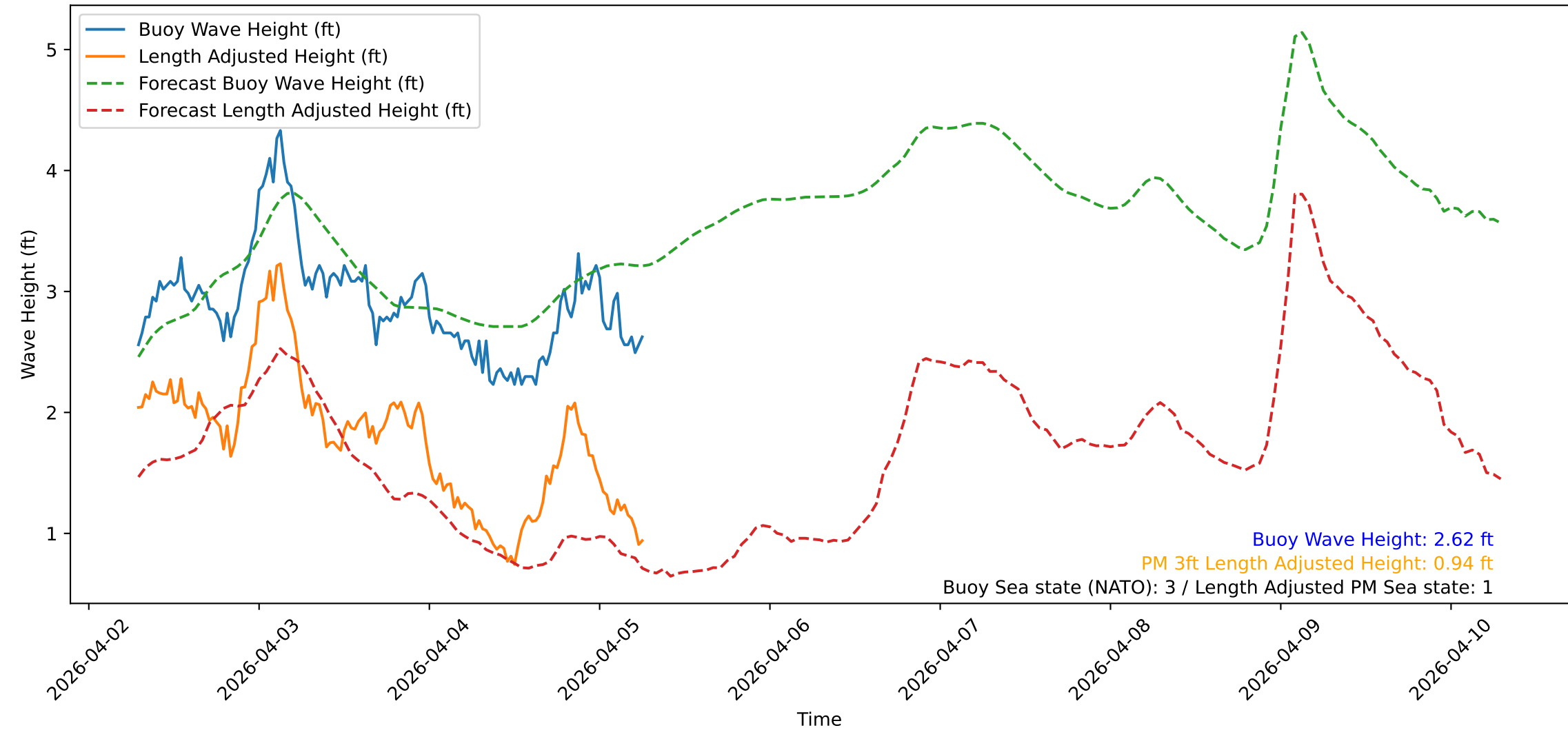
Wave Heights over Time for Green Beach at 2026-04-05 06:51:09
