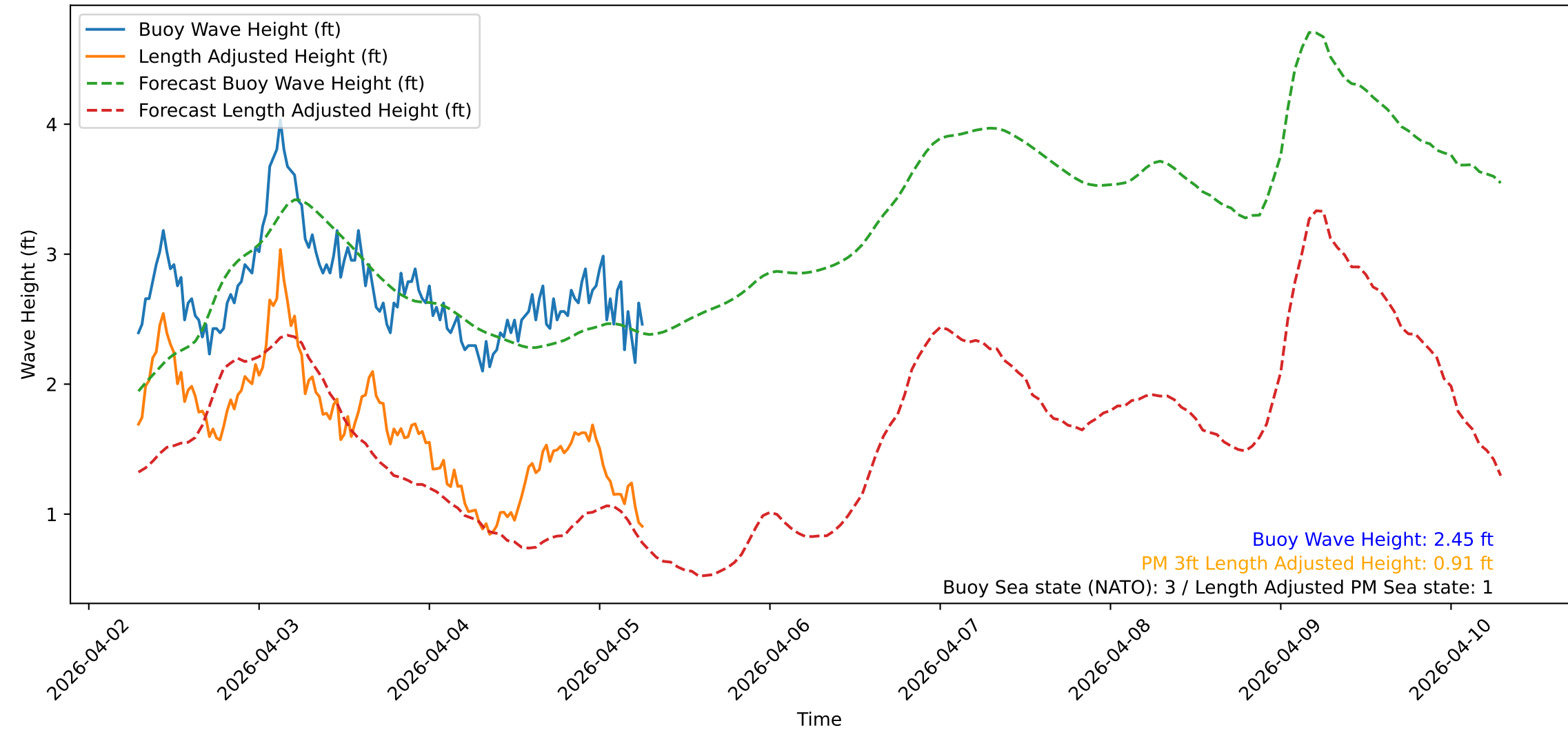
Wave Heights over Time for Oceanside Harbor at 2026-04-05 06:50:31
