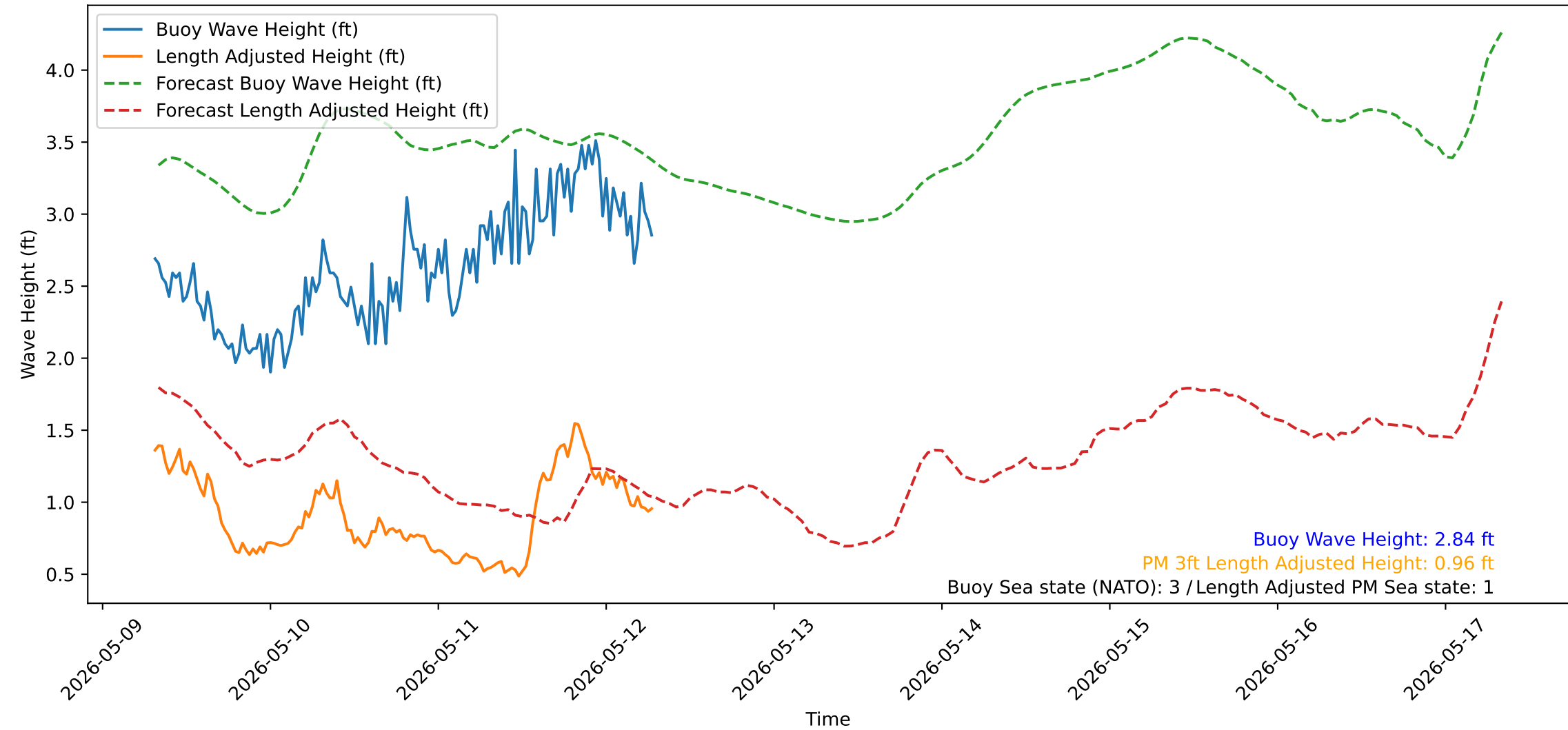
Wave Heights over Time for Green Beach at 2026-05-12 07:31:12
