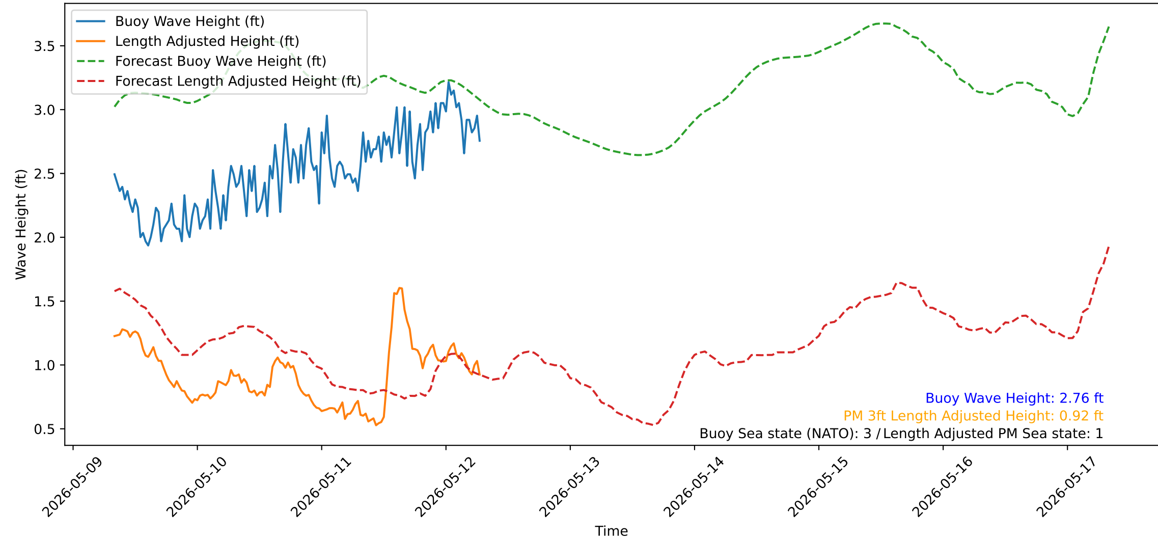
Wave Heights over Time for Red Beach at 2026-05-12 07:30:50
