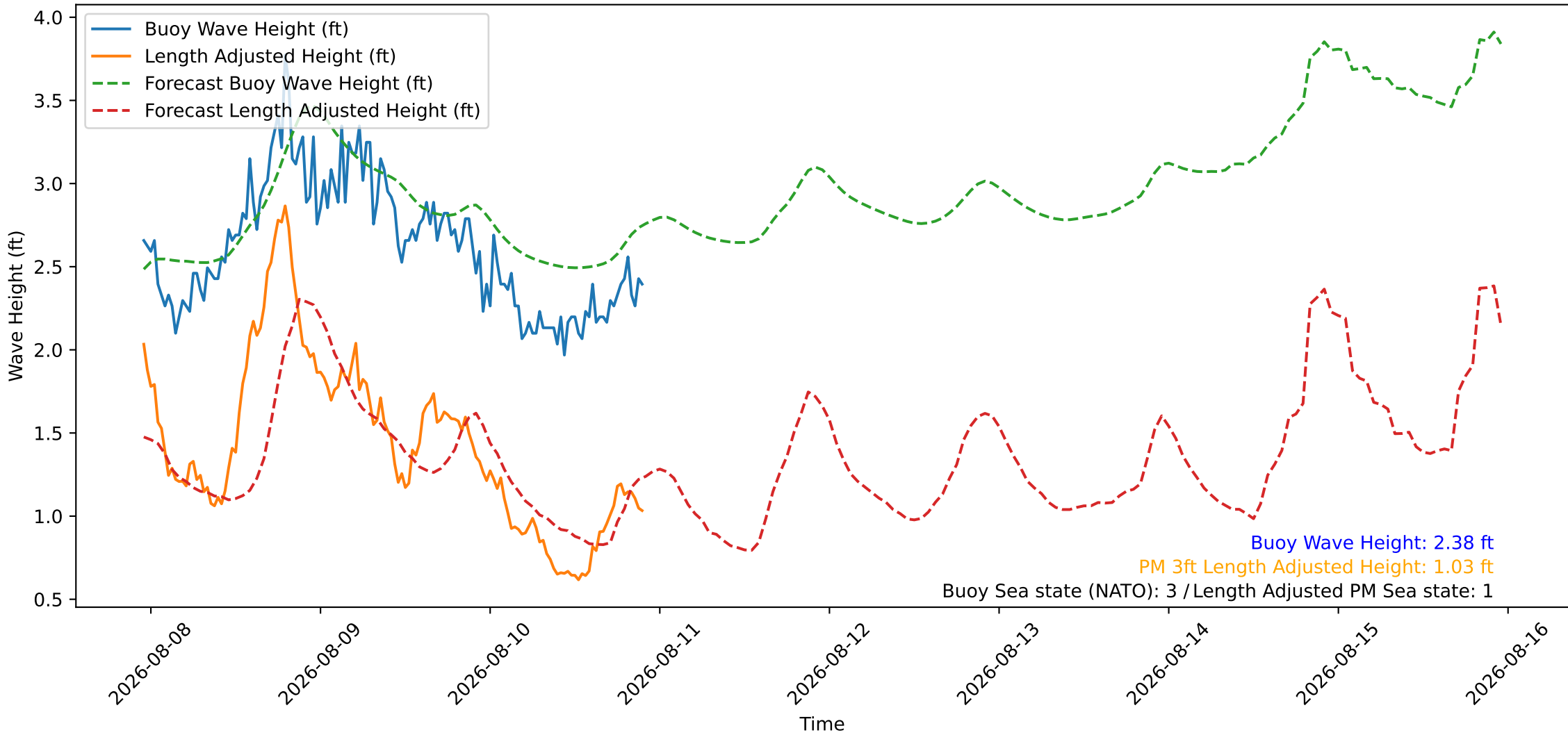
Wave Heights over Time for Green Beach at 2026-08-10 22:51:10
