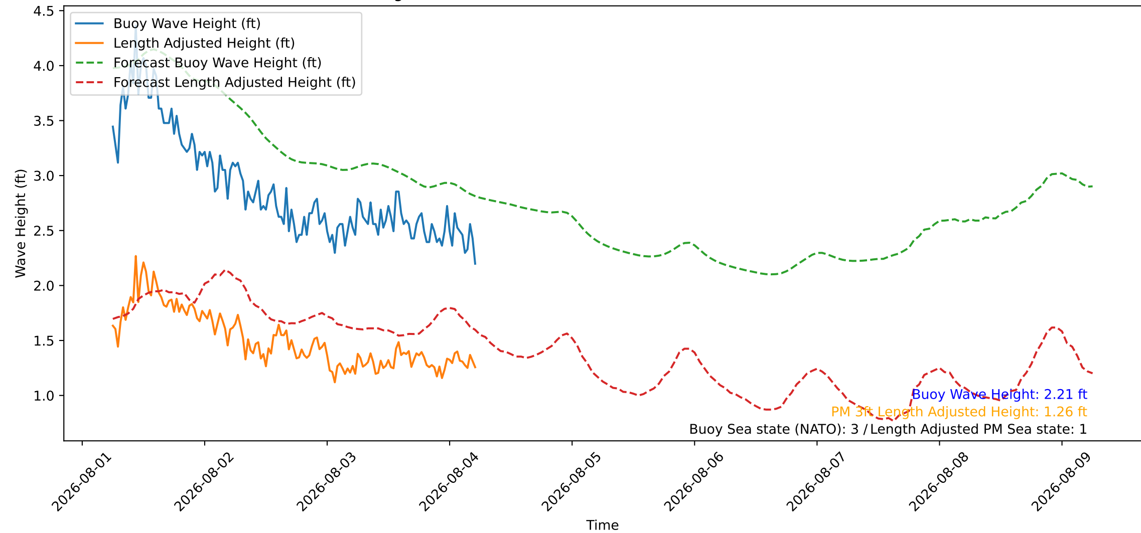
Wave Heights over Time for Oceanside Harbor at 2026-08-04 05:50:25
