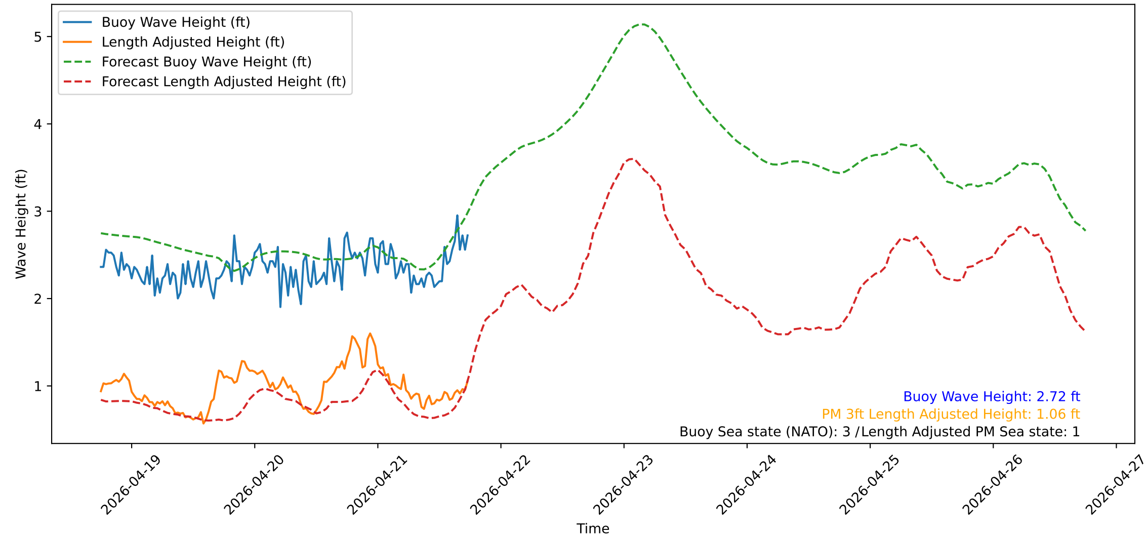
Wave Heights over Time for Oceanside Harbor at 2026-04-21 18:00:32
