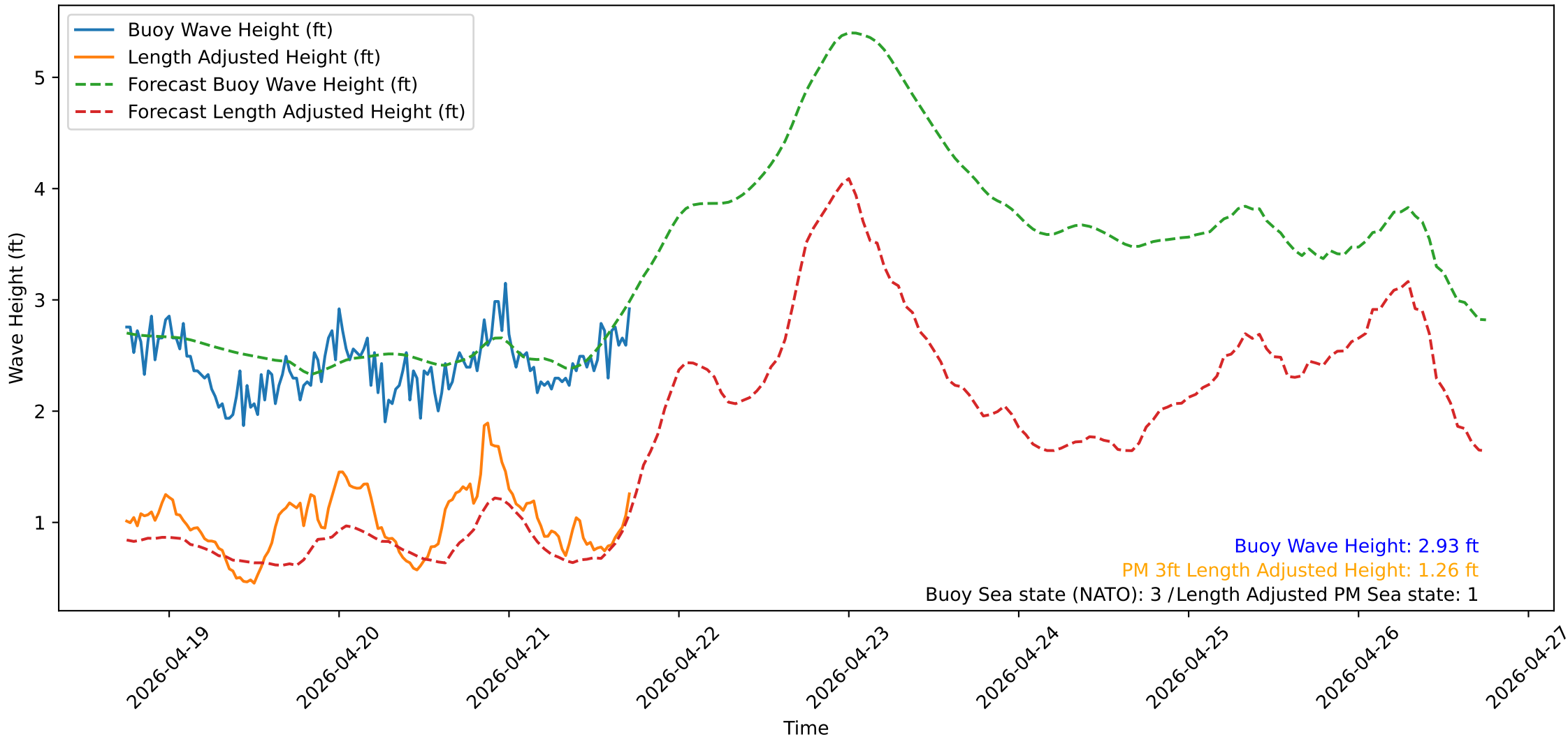
Wave Heights over Time for Green Beach at 2026-04-21 18:01:13
