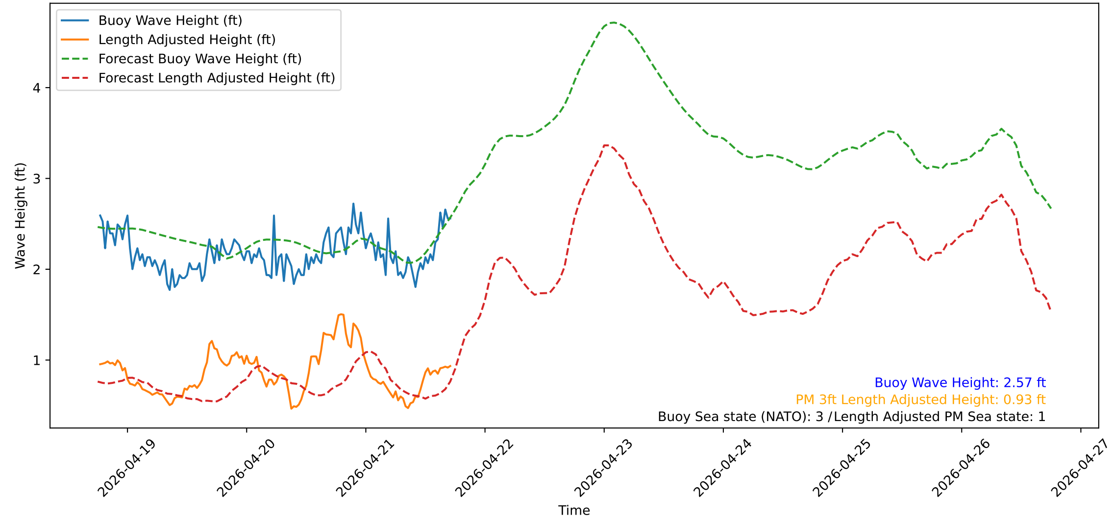
Wave Heights over Time for Red Beach at 2026-04-21 18:00:51
