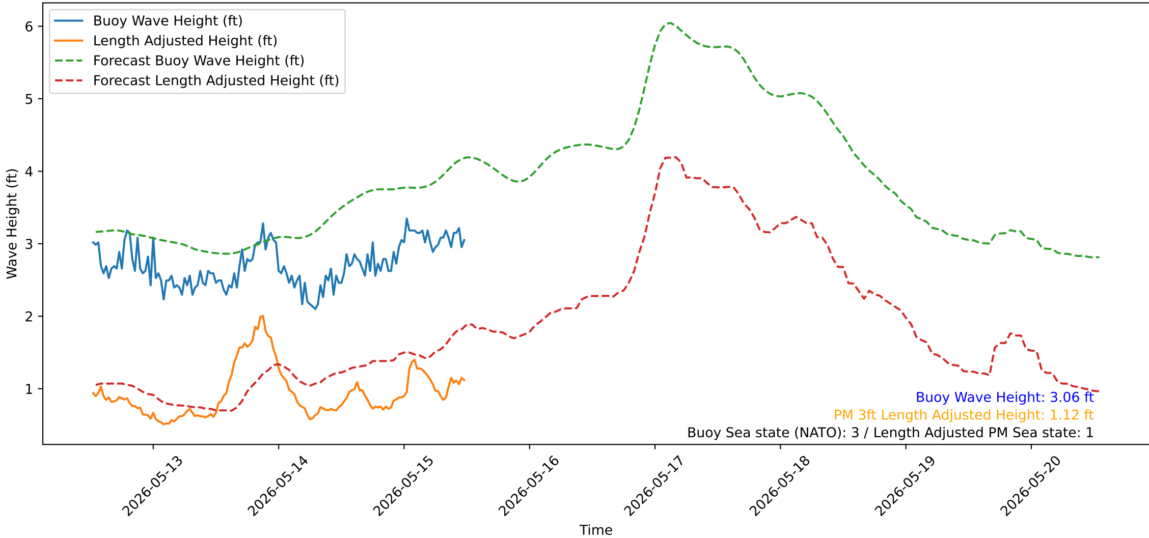
Wave Heights over Time for Green Beach at 2026-05-15 12:31:14
