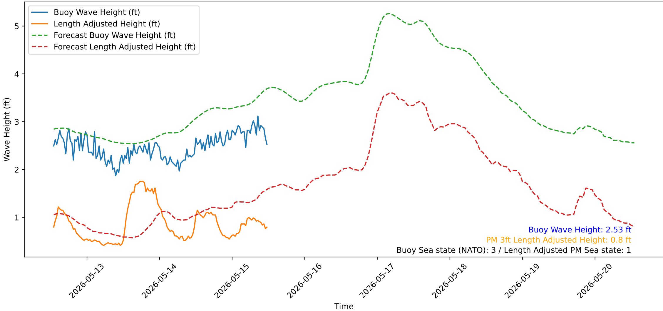
Wave Heights over Time for Red Beach at 2026-05-15 12:30:51
