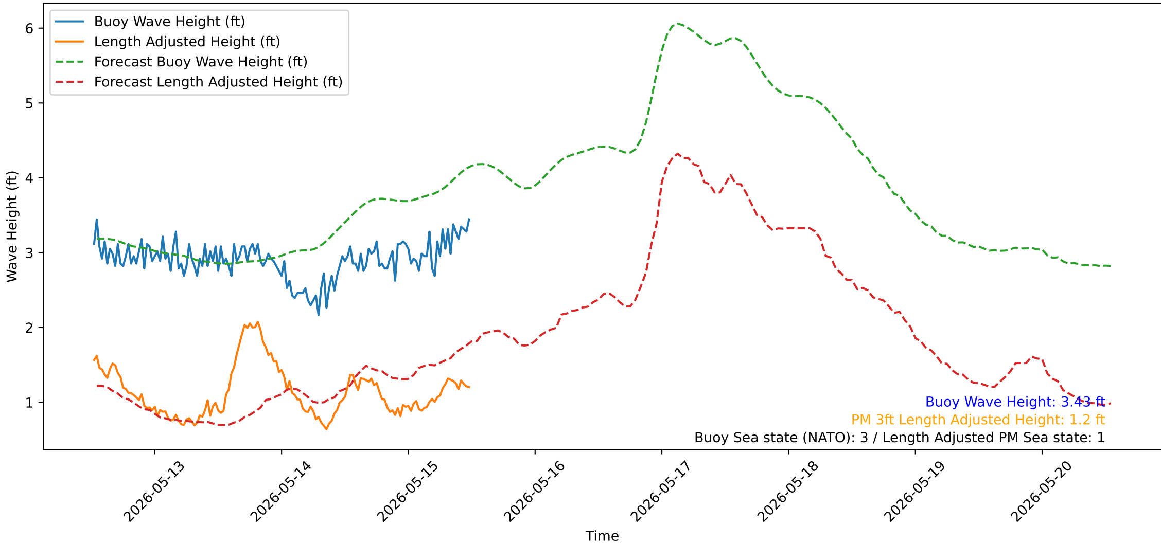
Wave Heights over Time for Oceanside Harbor at 2026-05-15 12:30:32
