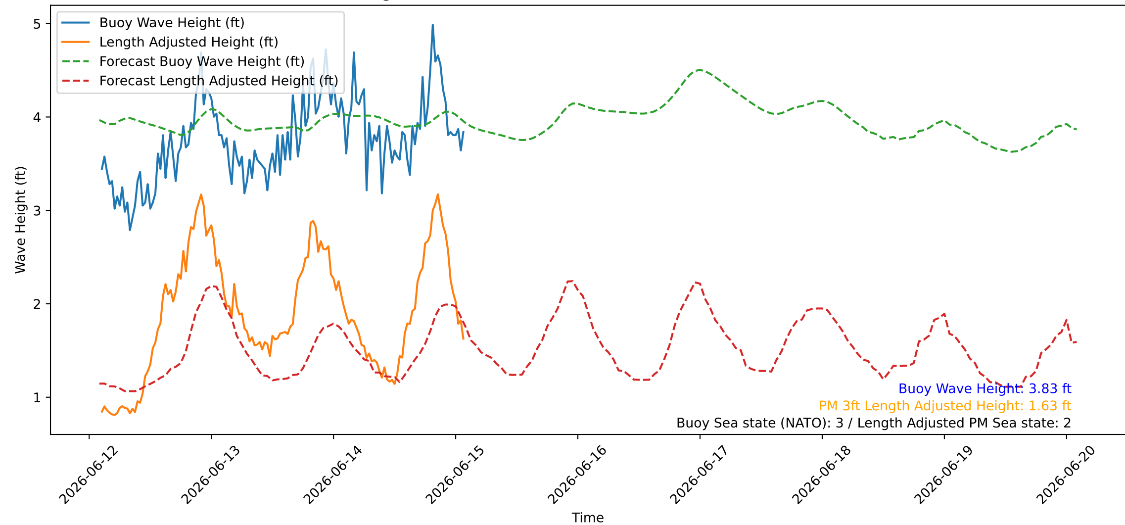
Wave Heights over Time for Oceanside Harbor at 2026-06-15 02:20:26
