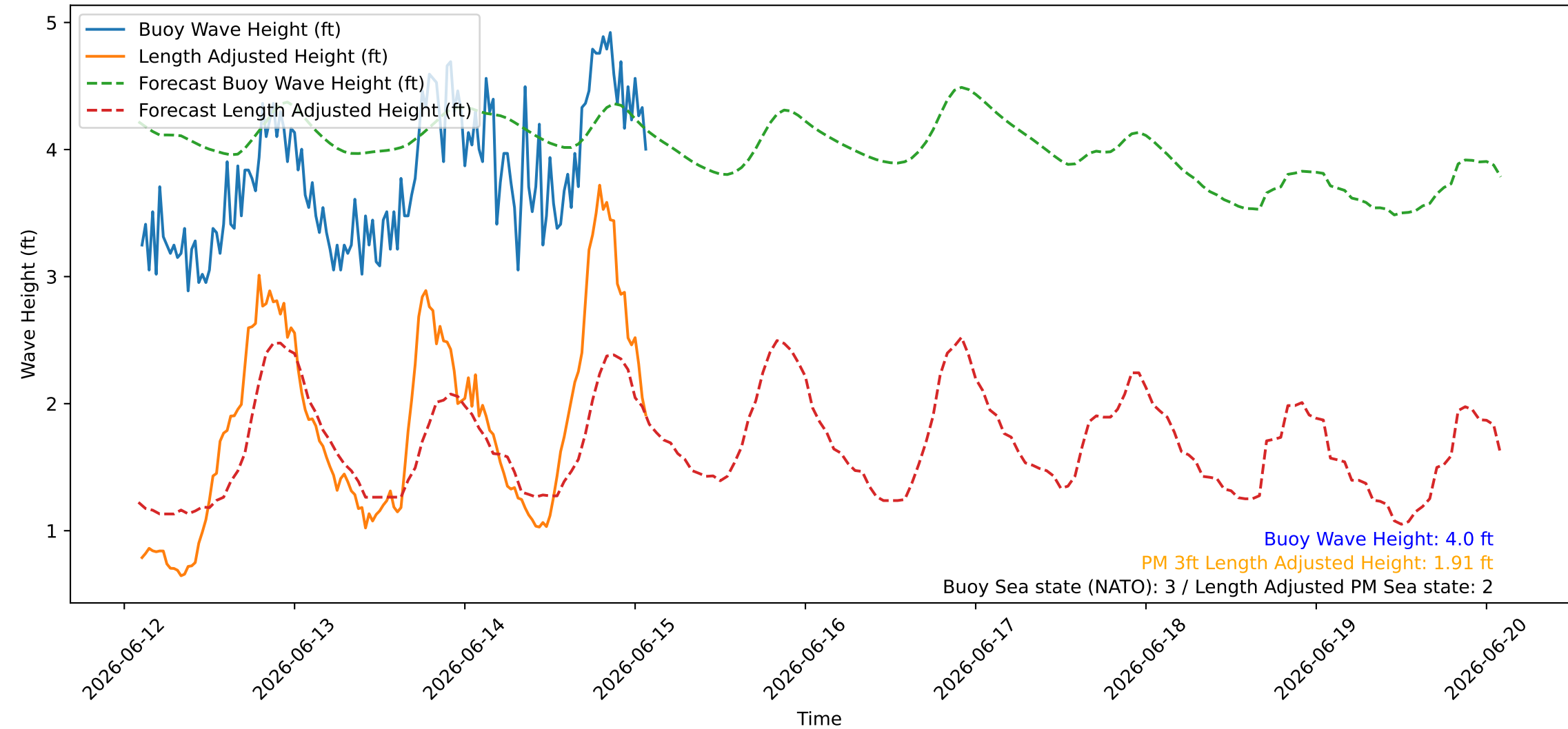
Wave Heights over Time for Green Beach at 2026-06-15 02:21:09
