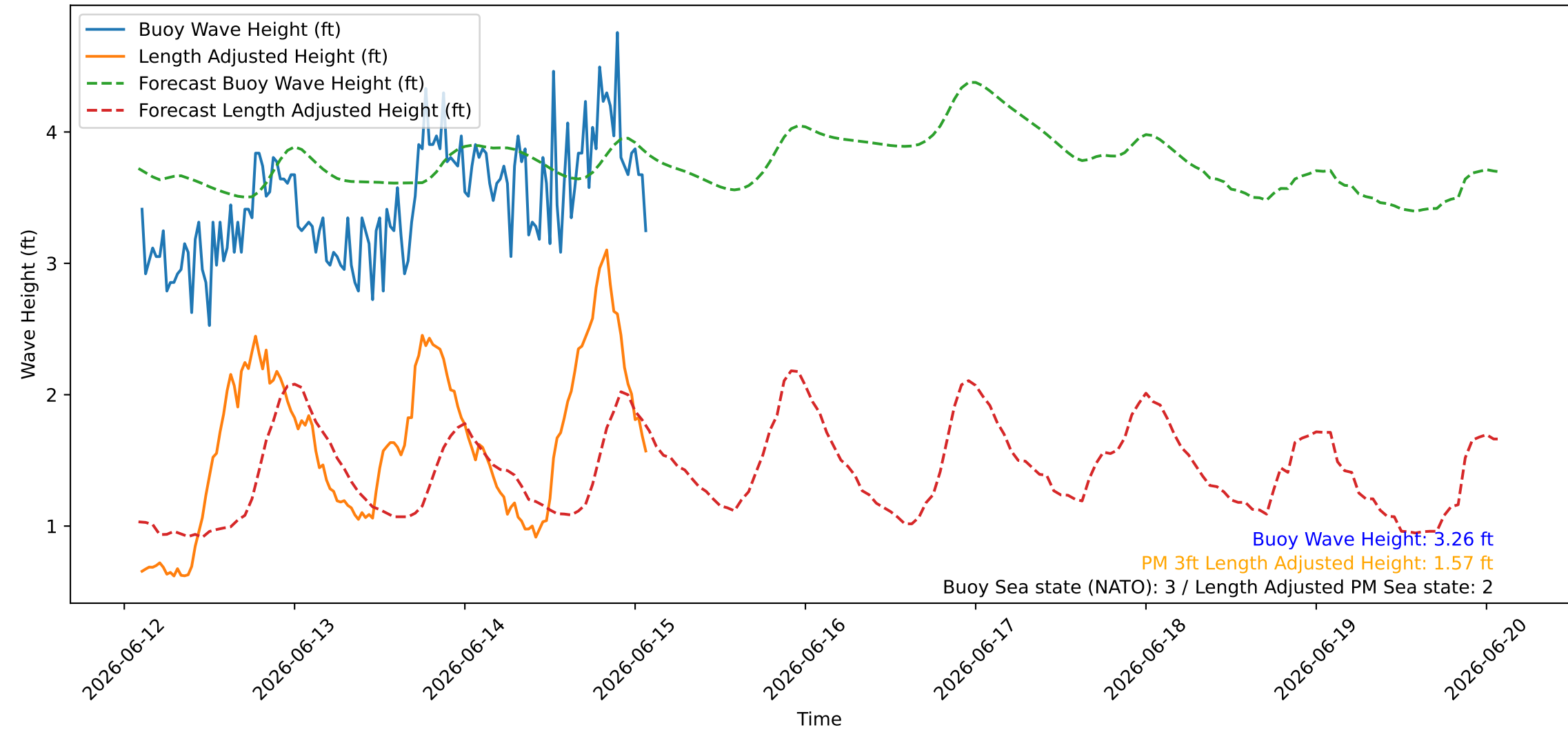
Wave Heights over Time for Red Beach at 2026-06-15 02:20:46
