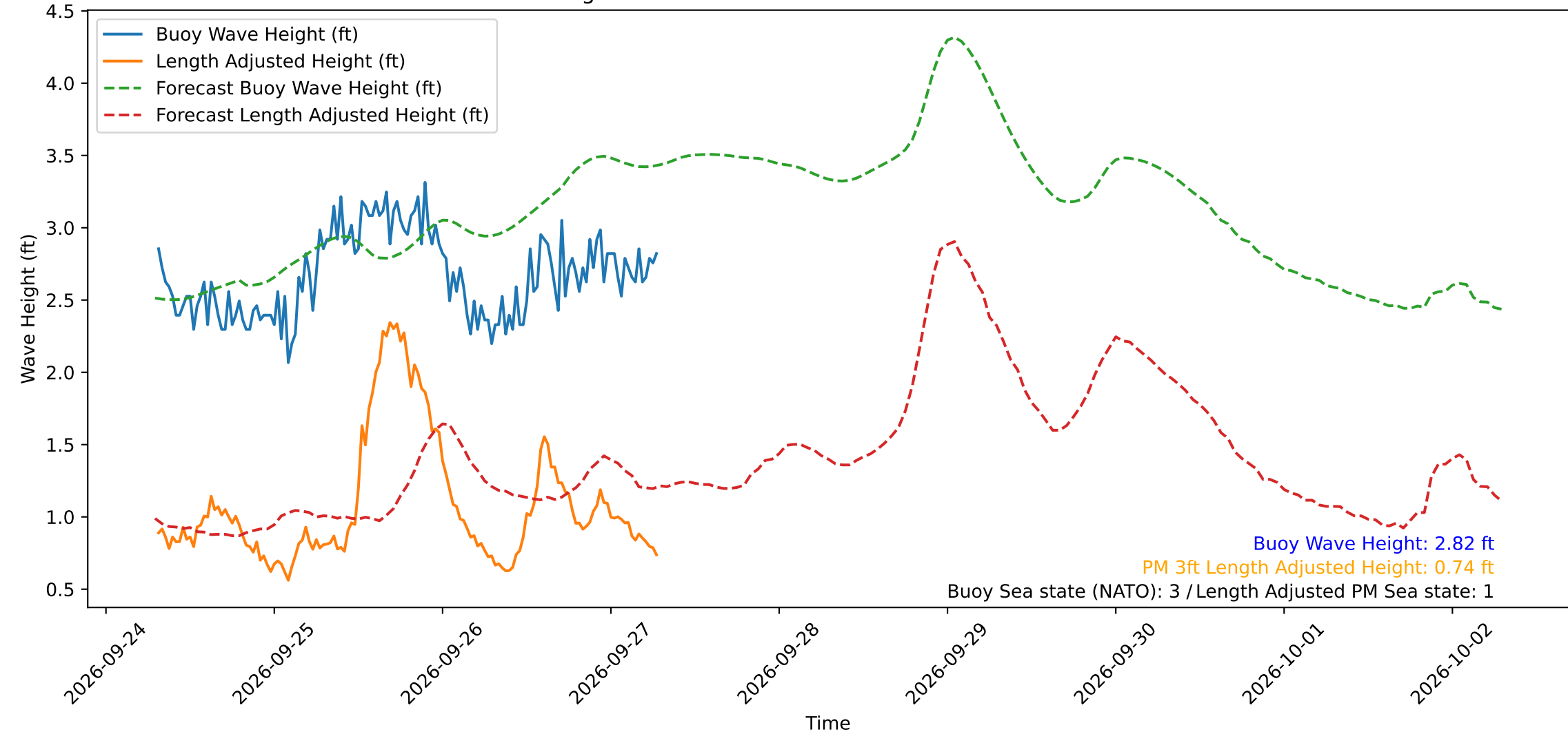
Wave Heights over Time for Red Beach at 2026-09-27 07:20:51
