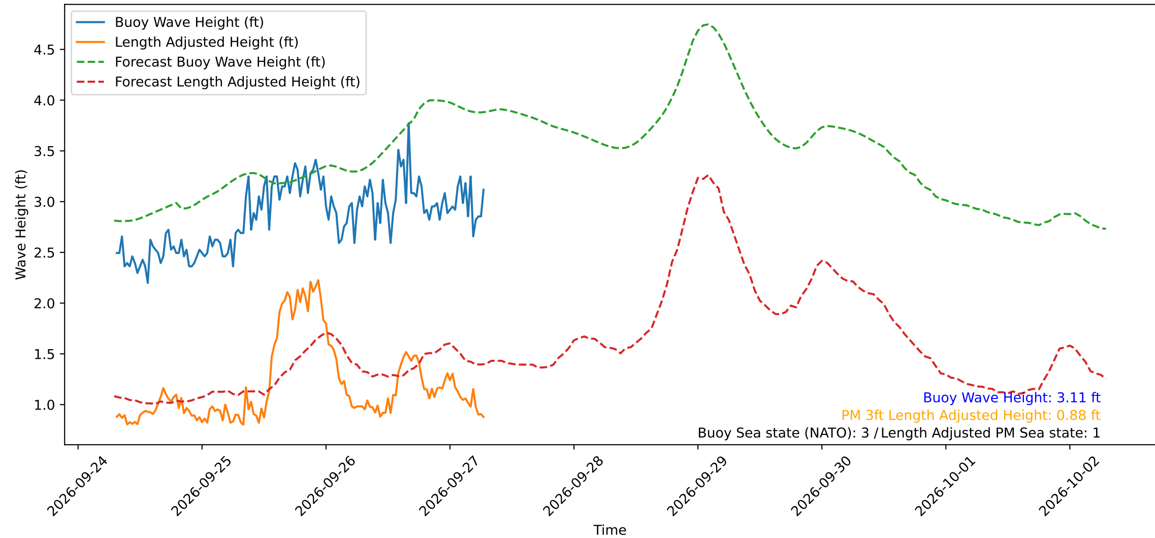
Wave Heights over Time for Oceanside Harbor at 2026-09-27 07:20:30
