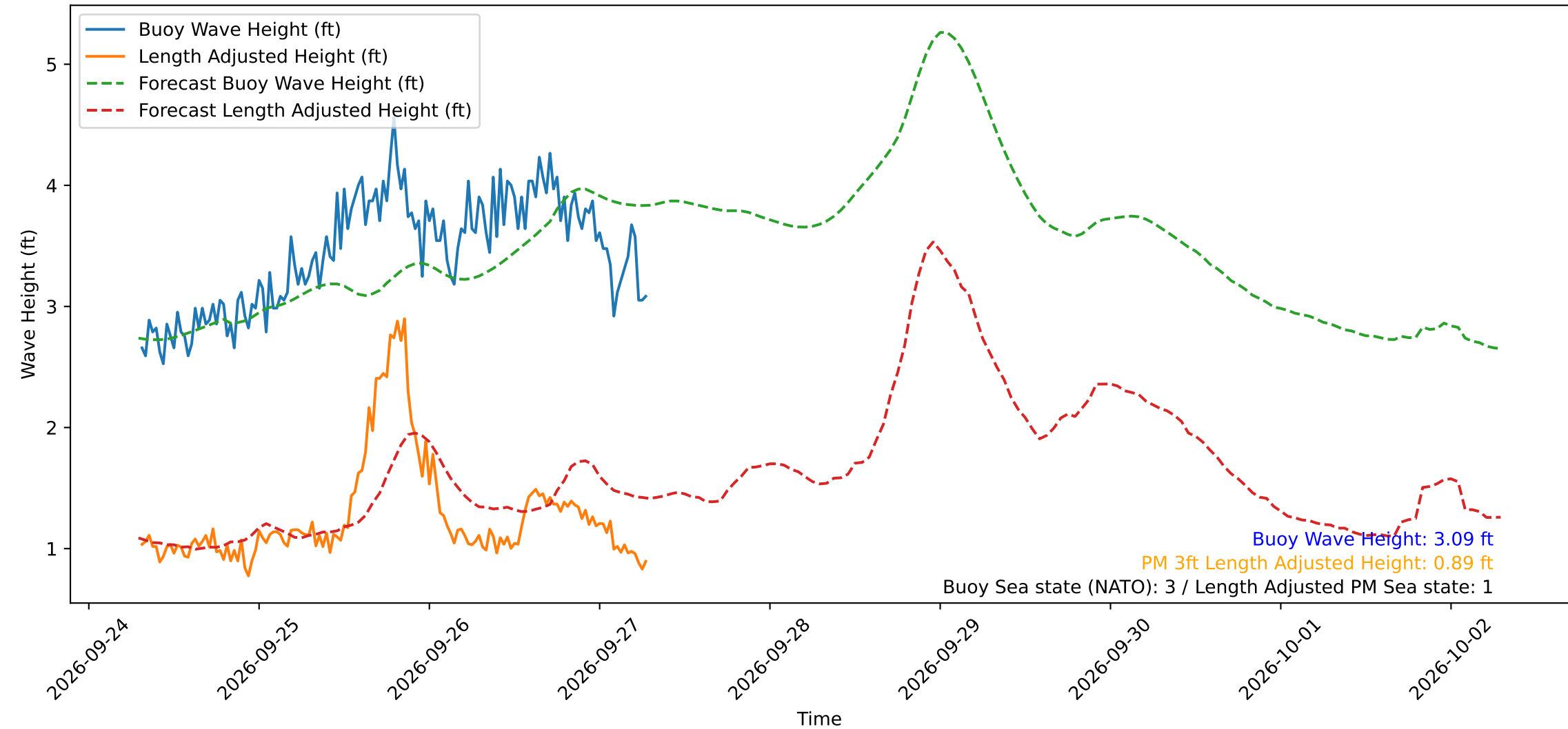
Wave Heights over Time for Green Beach at 2026-09-27 07:21:15
