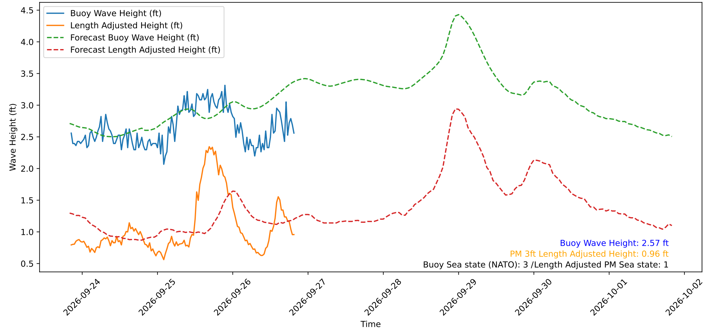
Wave Heights over Time for Red Beach at 2026-09-26 20:20:50
