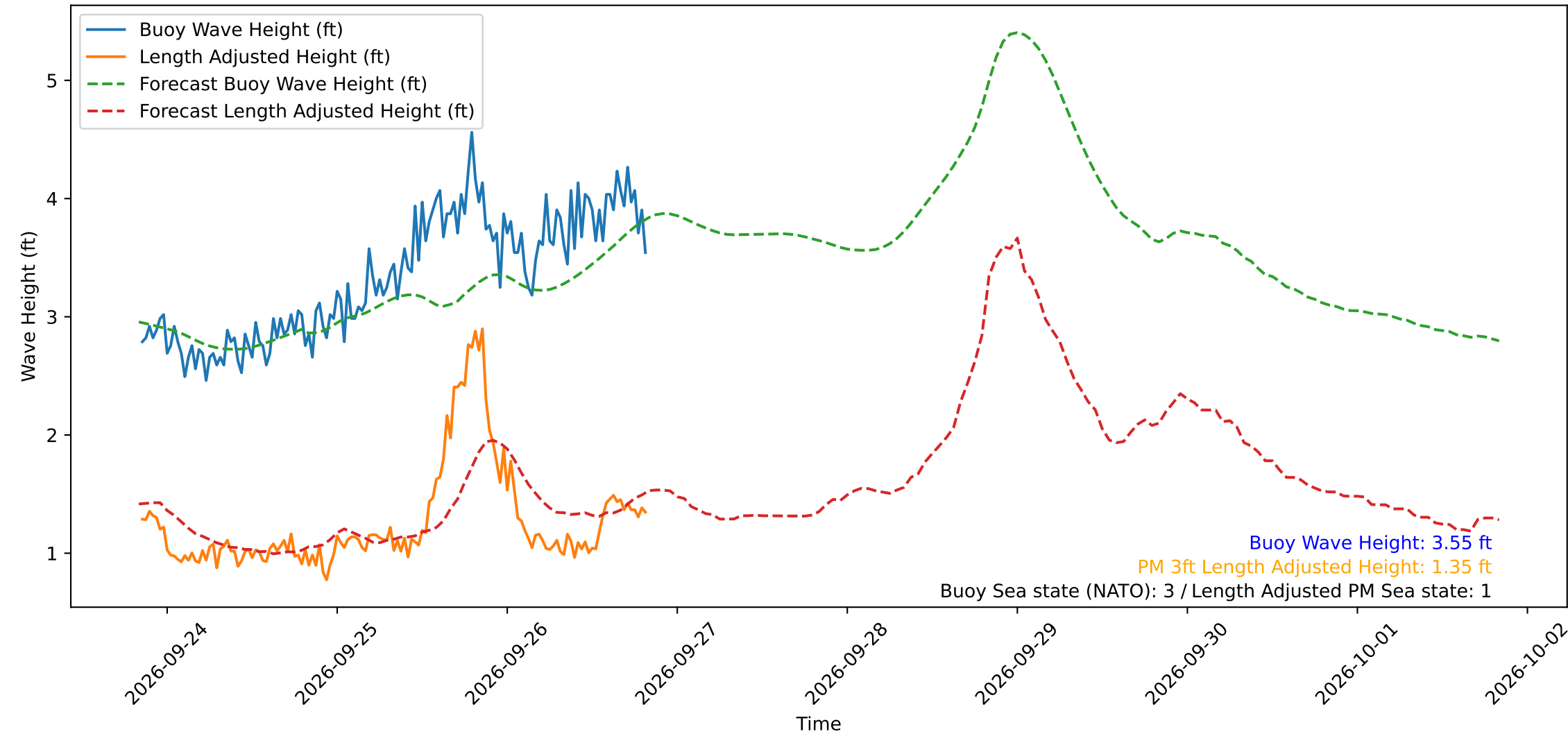
Wave Heights over Time for Green Beach at 2026-09-26 20:21:14
