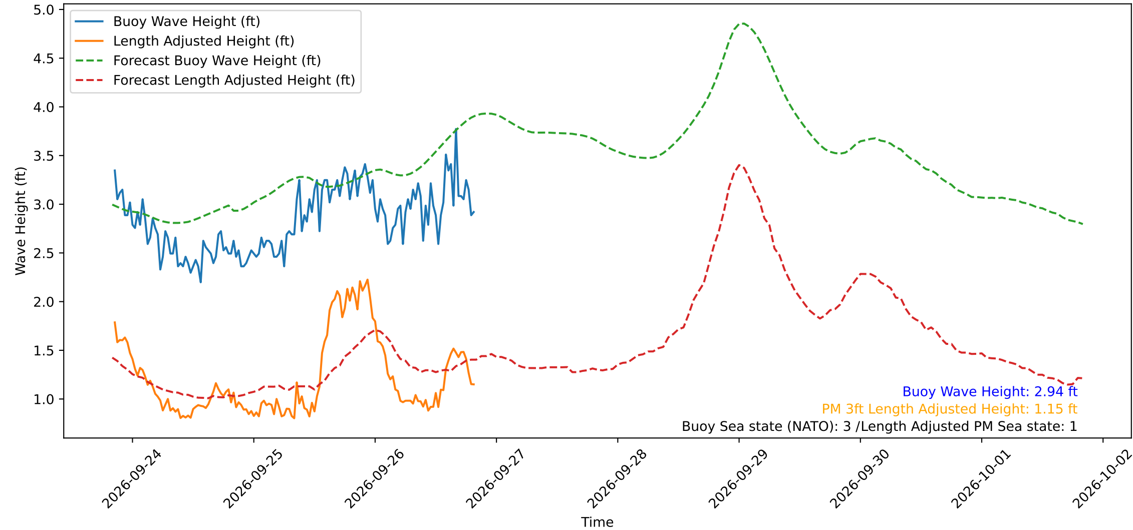
Wave Heights over Time for Oceanside Harbor at 2026-09-26 20:20:30
