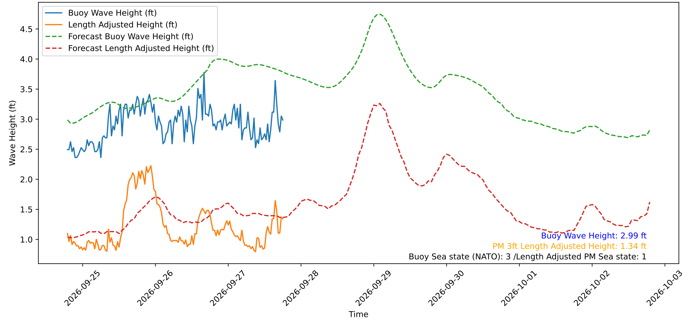
Wave Heights over Time for Oceanside Harbor at 2026-09-27 19:00:31
