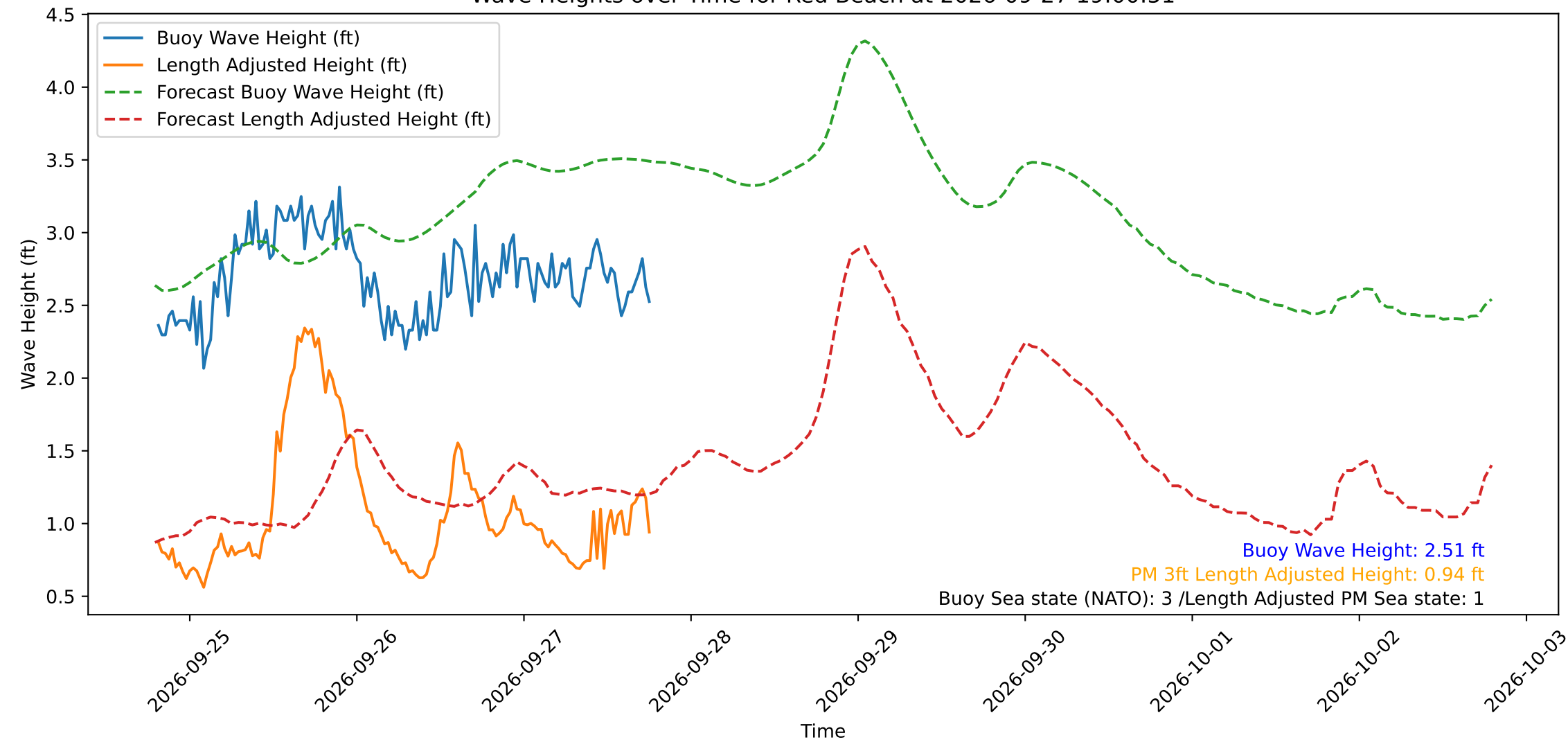
Wave Heights over Time for Red Beach at 2026-09-27 19:00:51
