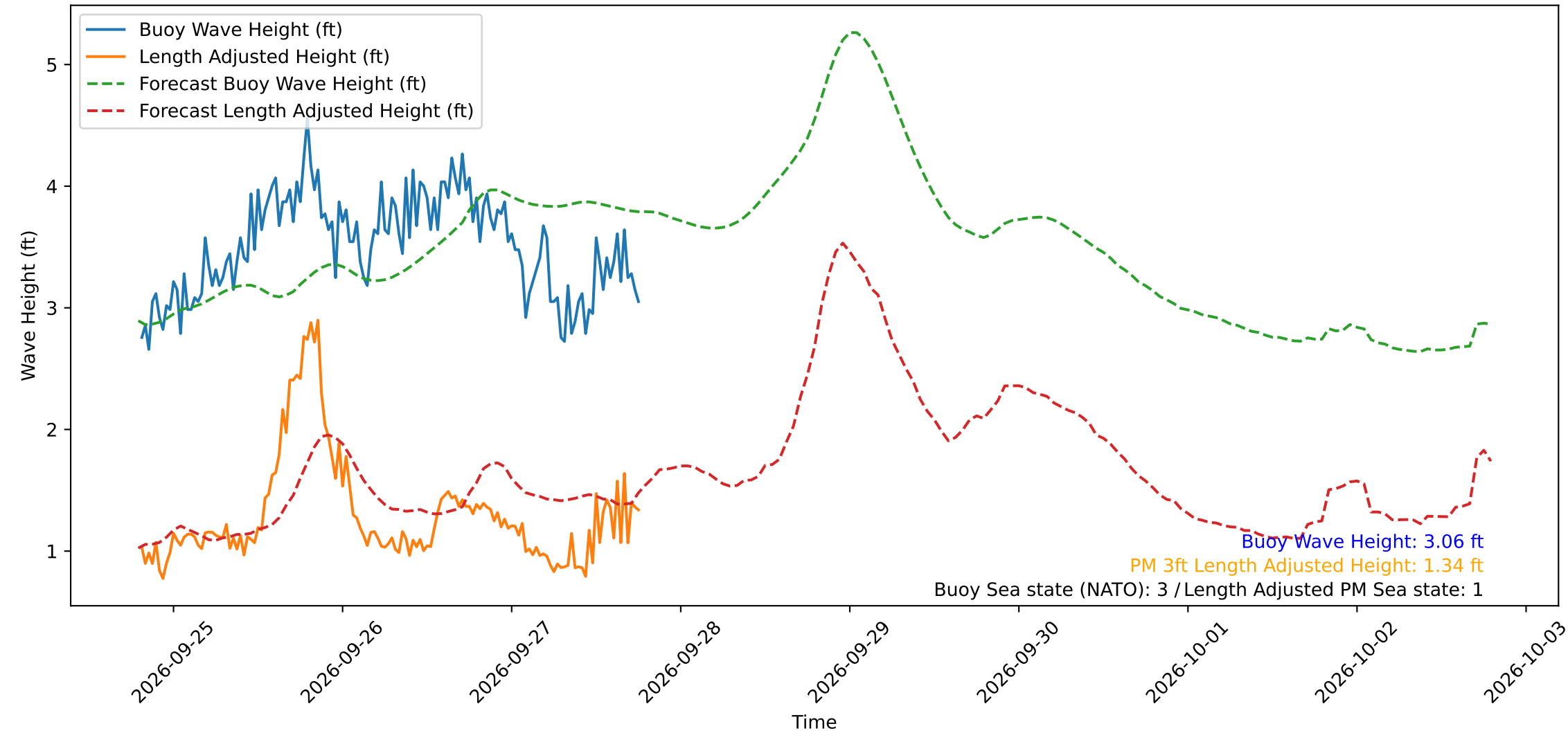
Wave Heights over Time for Green Beach at 2026-09-27 19:01:14
