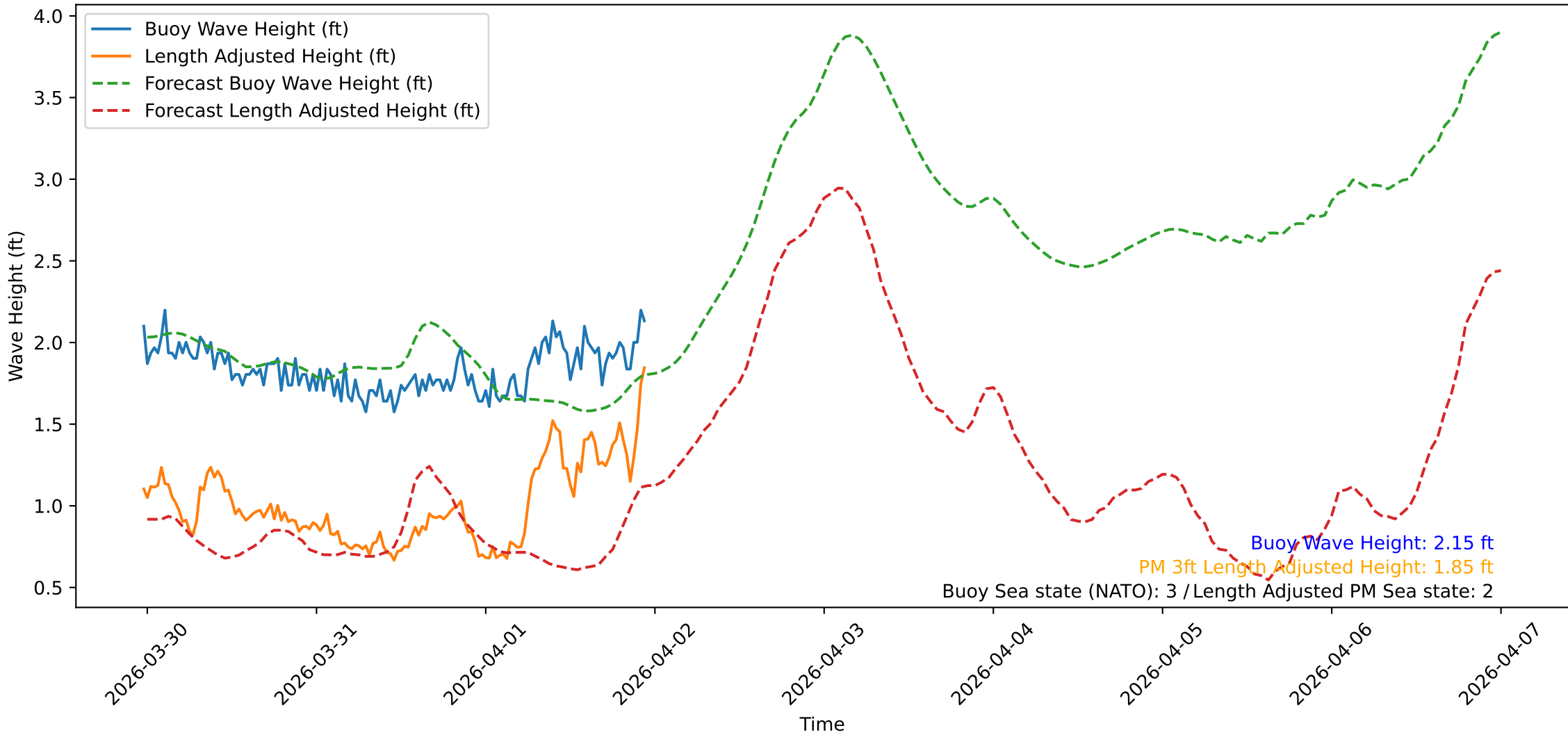
Wave Heights over Time for Oceanside Harbor at 2026-04-01 23:30:31
