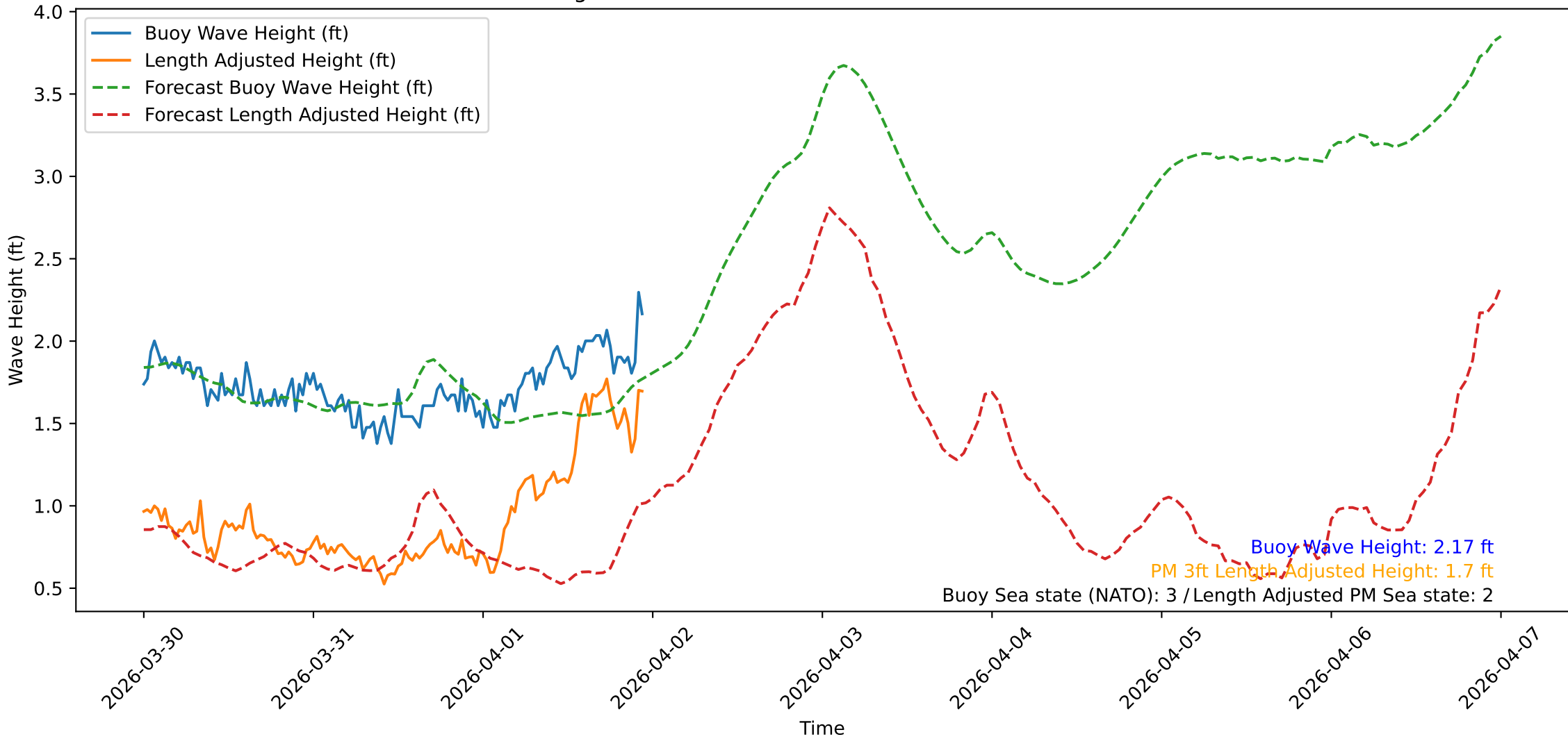
Wave Heights over Time for Red Beach at 2026-04-01 23:30:47
