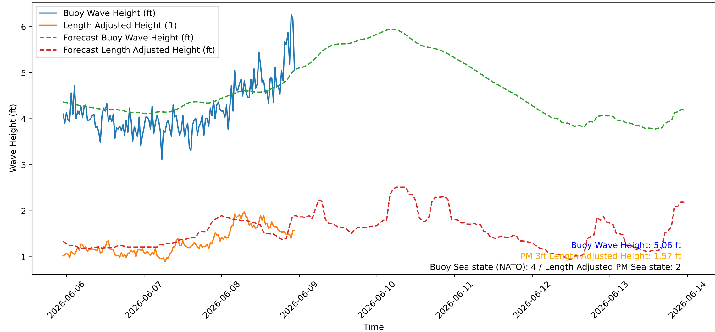
Wave Heights over Time for Green Beach at 2026-06-08 23:11:09
