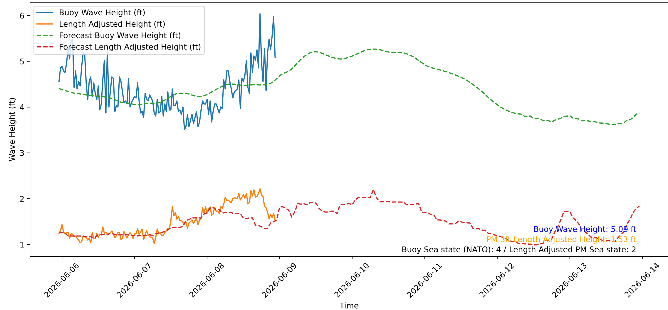
Wave Heights over Time for Oceanside Harbor at 2026-06-08 23:10:26
