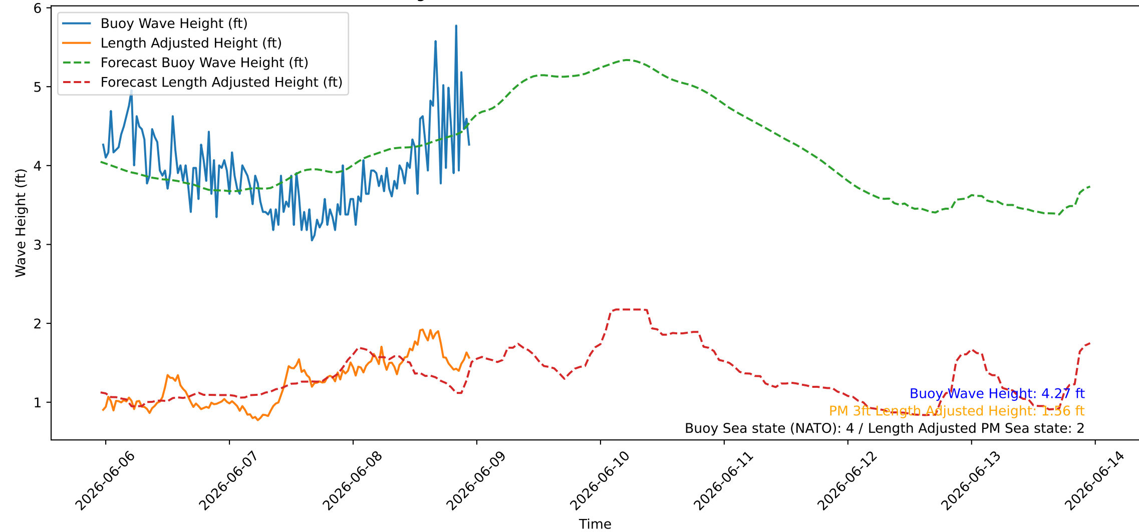
Wave Heights over Time for Red Beach at 2026-06-08 23:10:46
