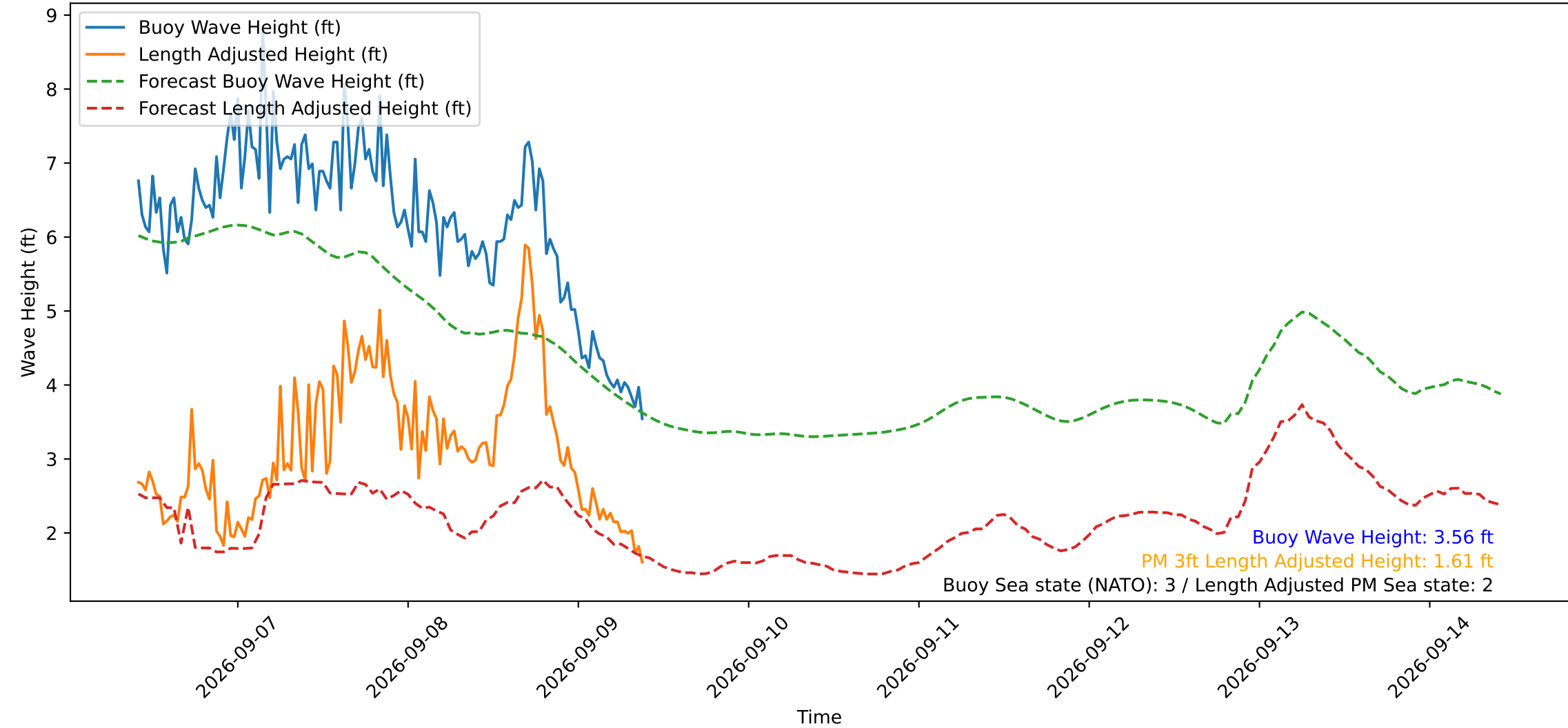
Wave Heights over Time for Green Beach at 2026-09-09 09:51:14
