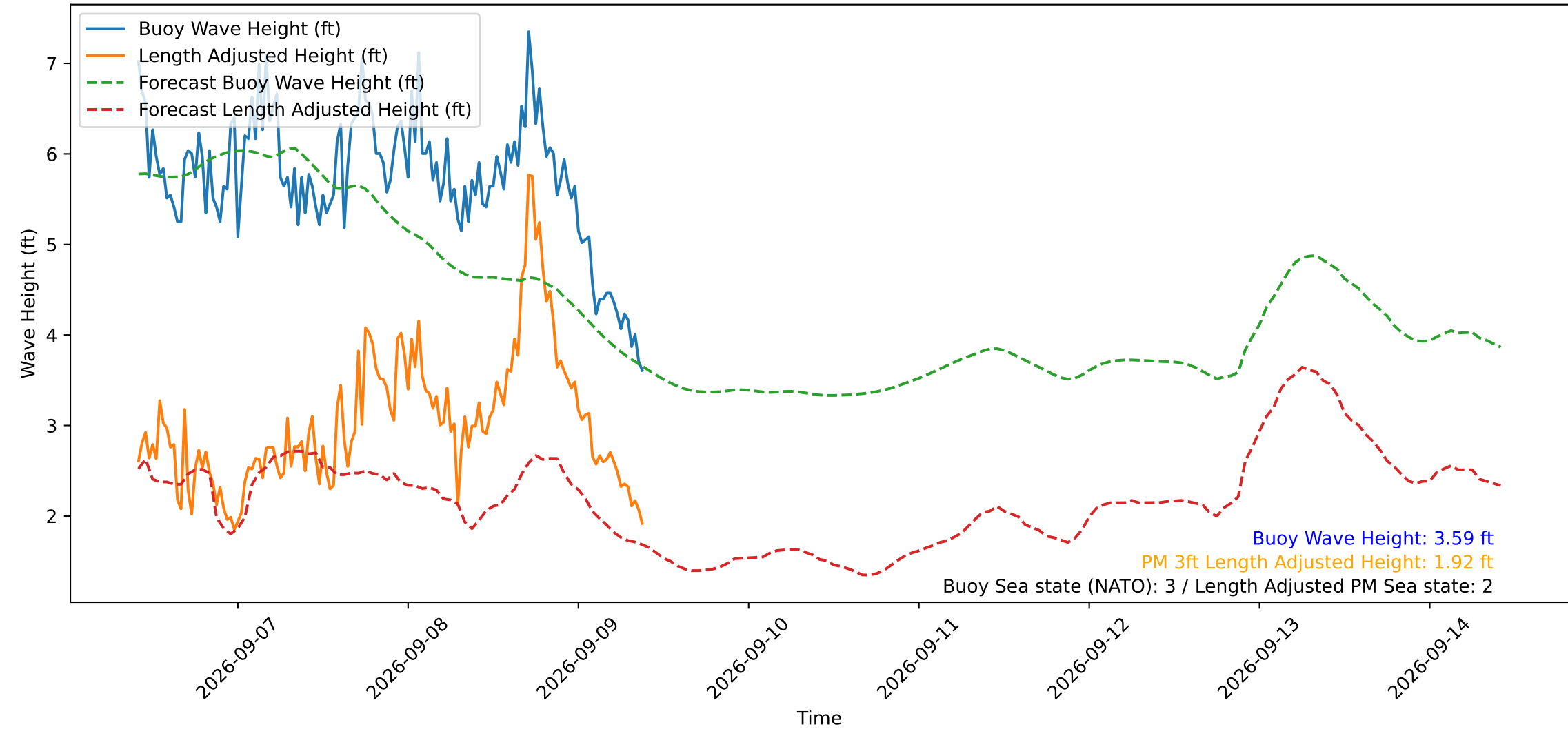
Wave Heights over Time for Oceanside Harbor at 2026-09-09 09:50:30
