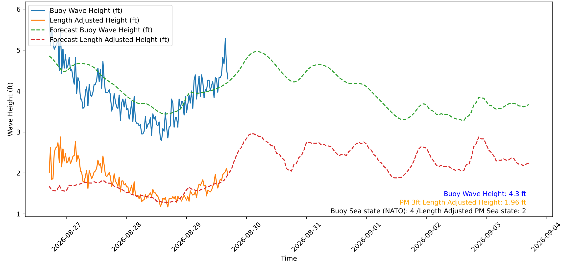
Wave Heights over Time for Oceanside Harbor at 2026-08-29 17:10:29
