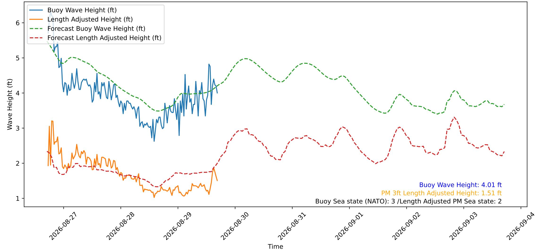
Wave Heights over Time for Green Beach at 2026-08-29 17:11:12
