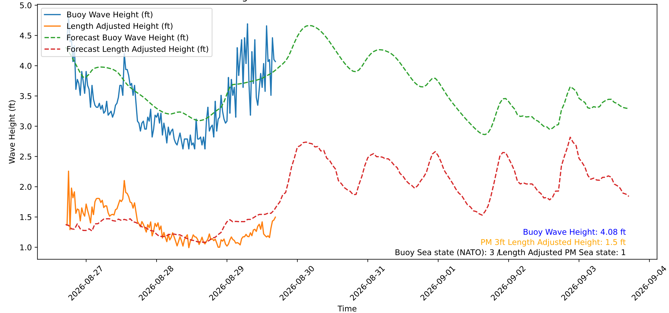
Wave Heights over Time for Red Beach at 2026-08-29 17:10:48
