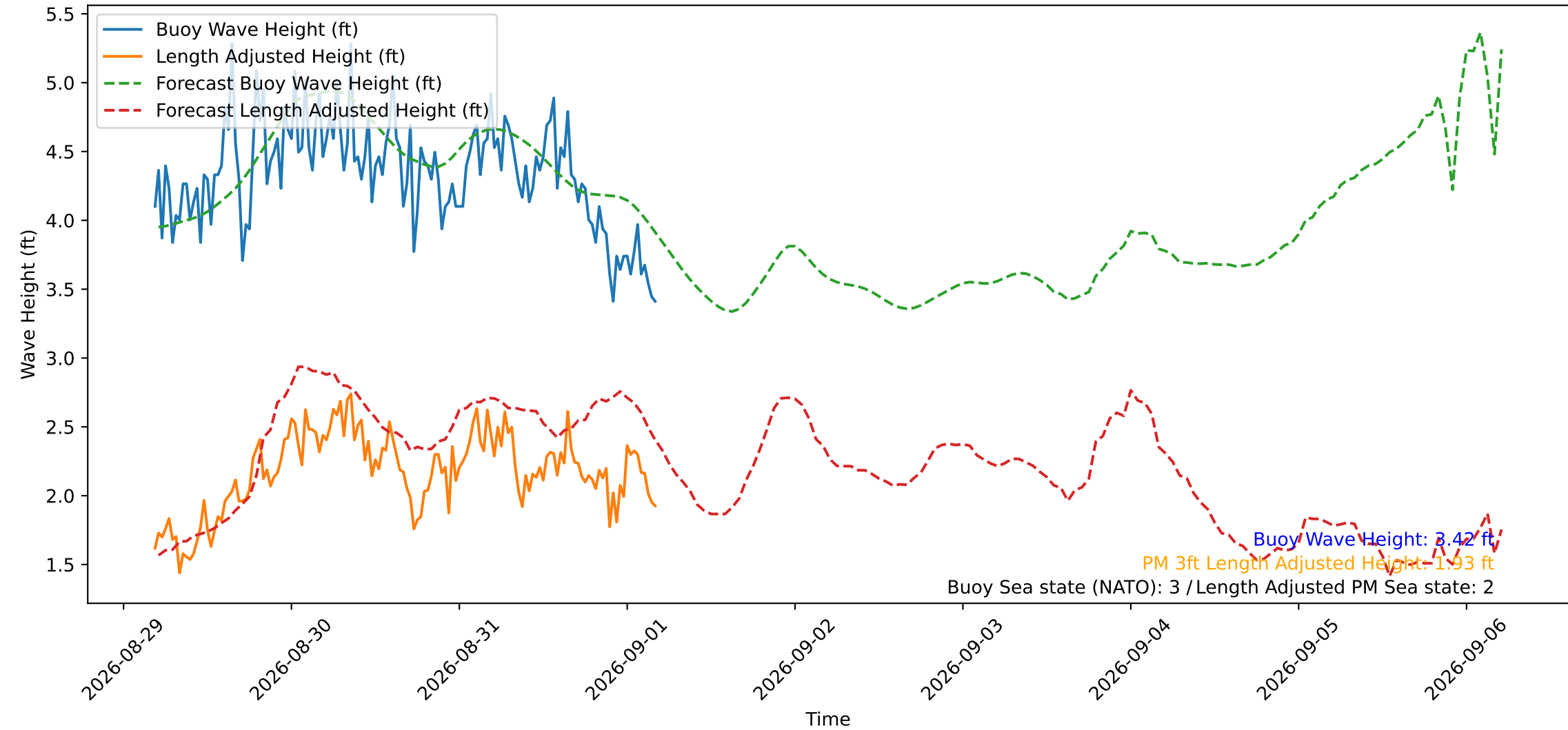
Wave Heights over Time for Oceanside Harbor at 2026-09-01 04:40:29
