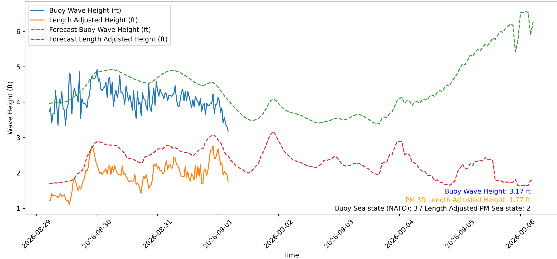
Wave Heights over Time for Green Beach at 2026-09-01 04:41:13
