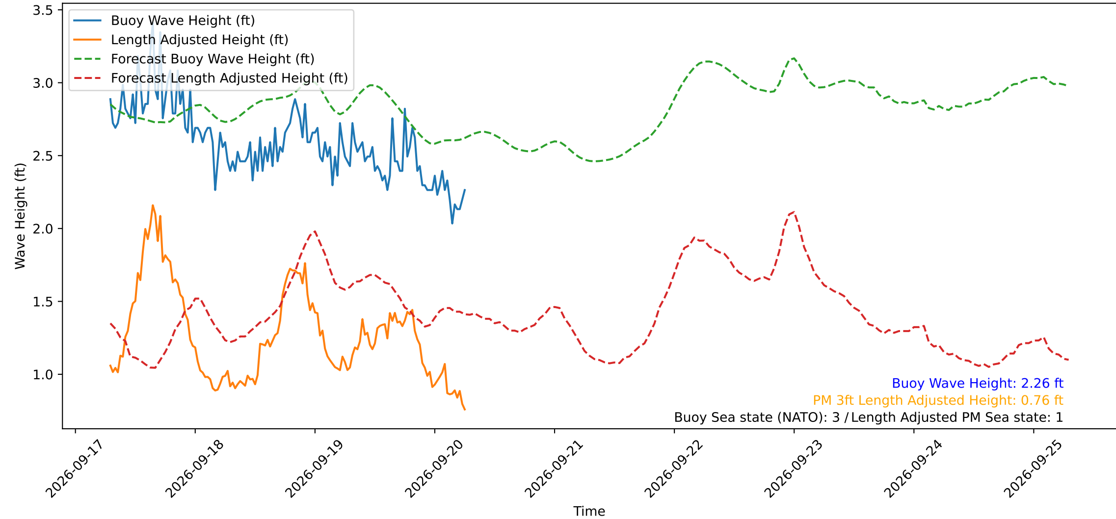
Wave Heights over Time for Red Beach at 2026-09-20 06:50:50
