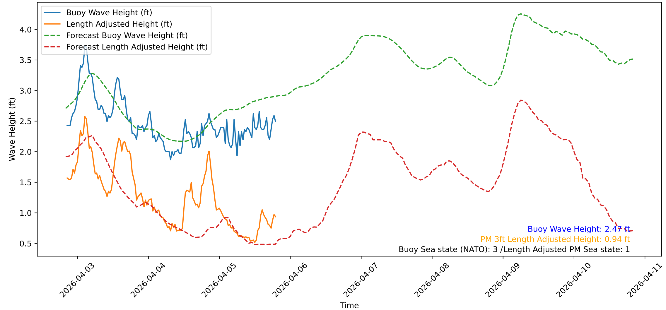
Wave Heights over Time for Red Beach at 2026-04-05 20:00:59
