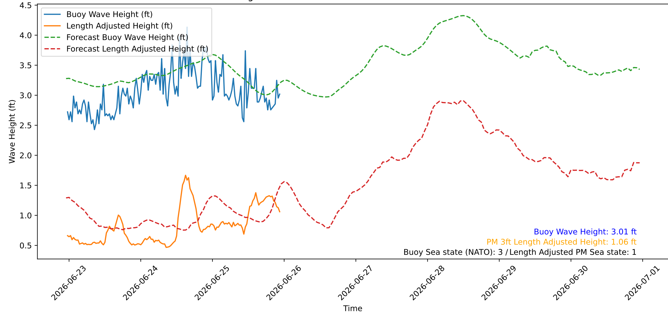
Wave Heights over Time for Red Beach at 2026-06-25 23:20:47
