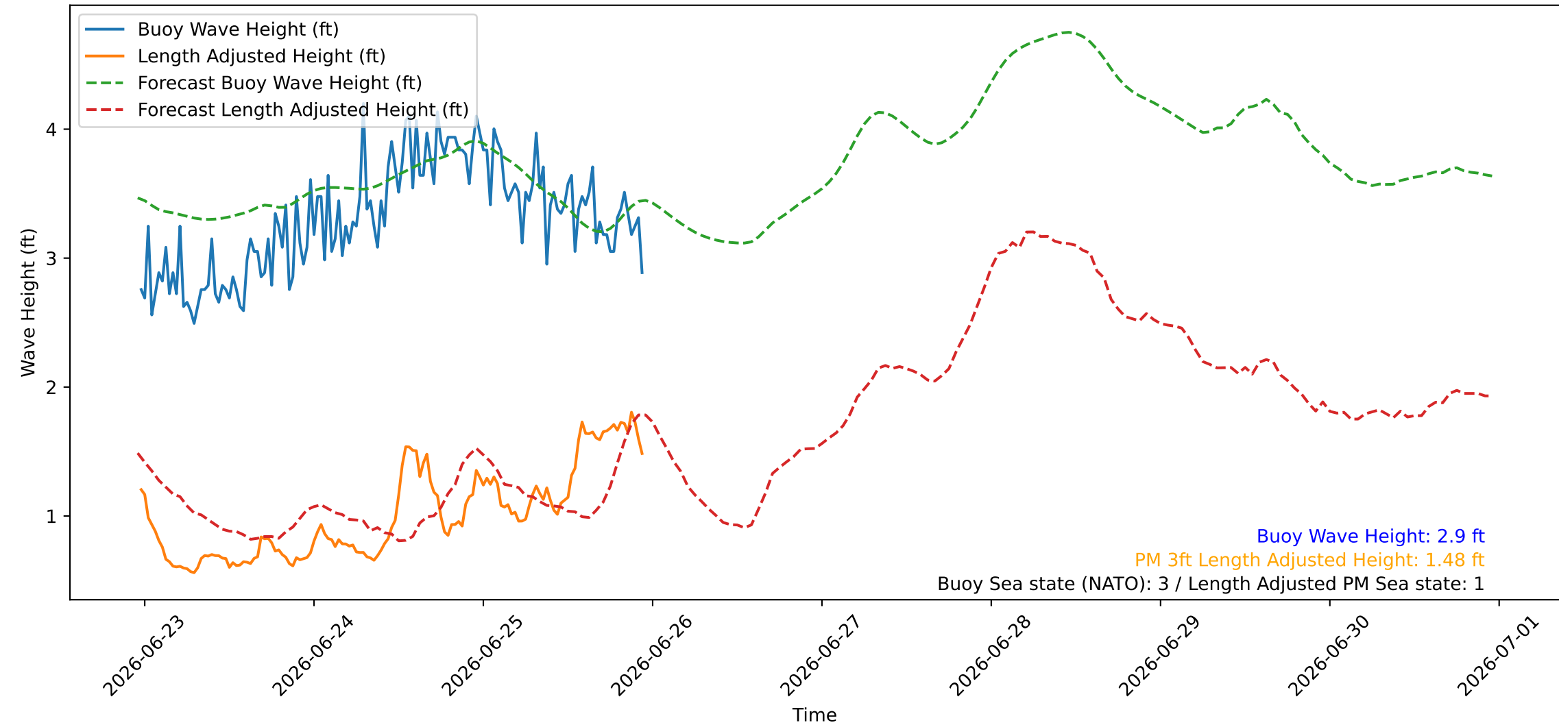
Wave Heights over Time for Green Beach at 2026-06-25 23:21:09
