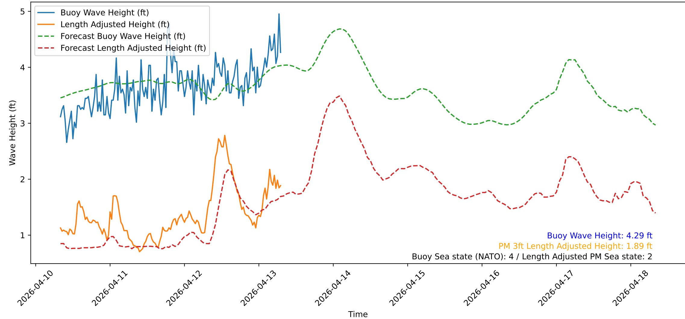
Wave Heights over Time for Oceanside Harbor at 2026-04-13 07:50:31
