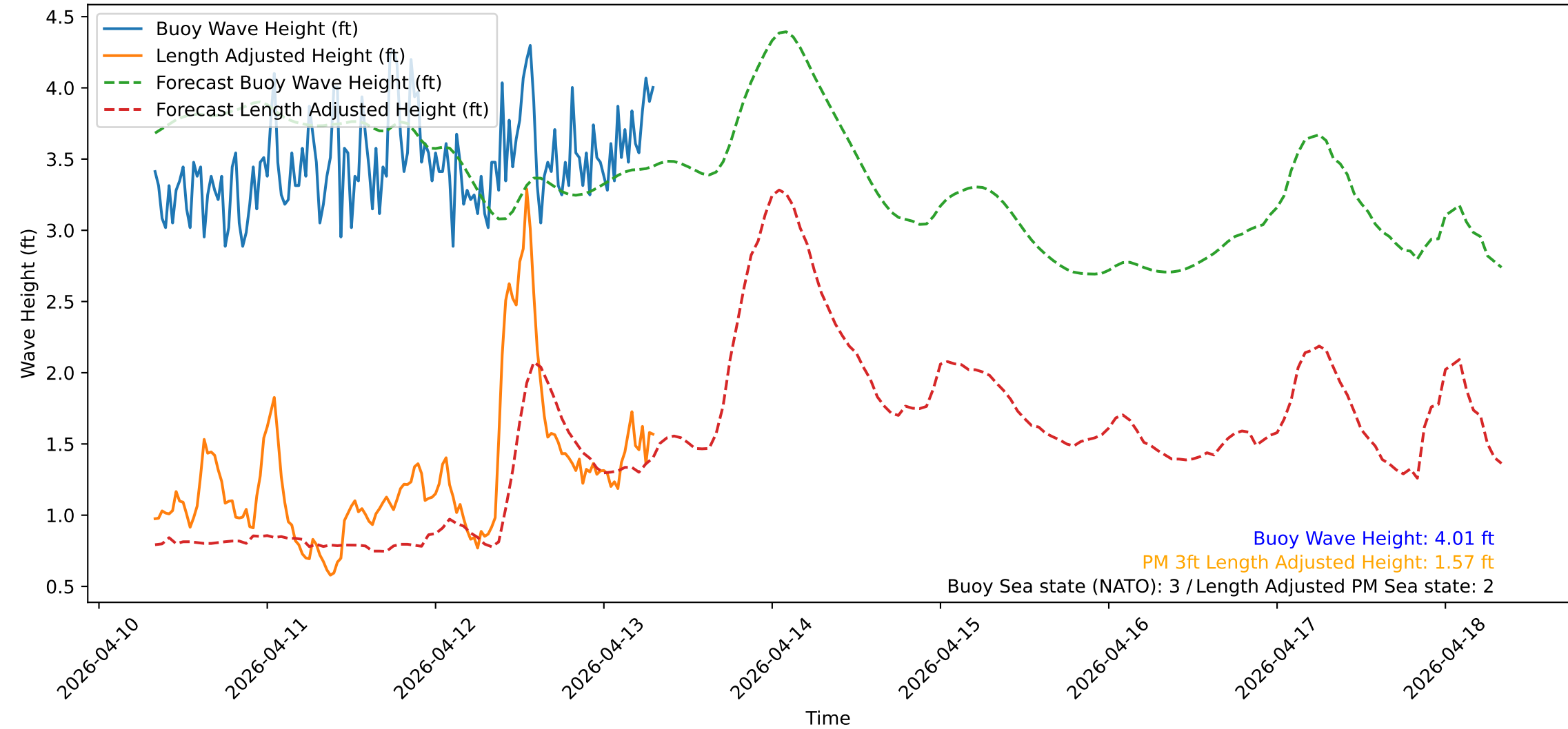
Wave Heights over Time for Red Beach at 2026-04-13 07:50:51
