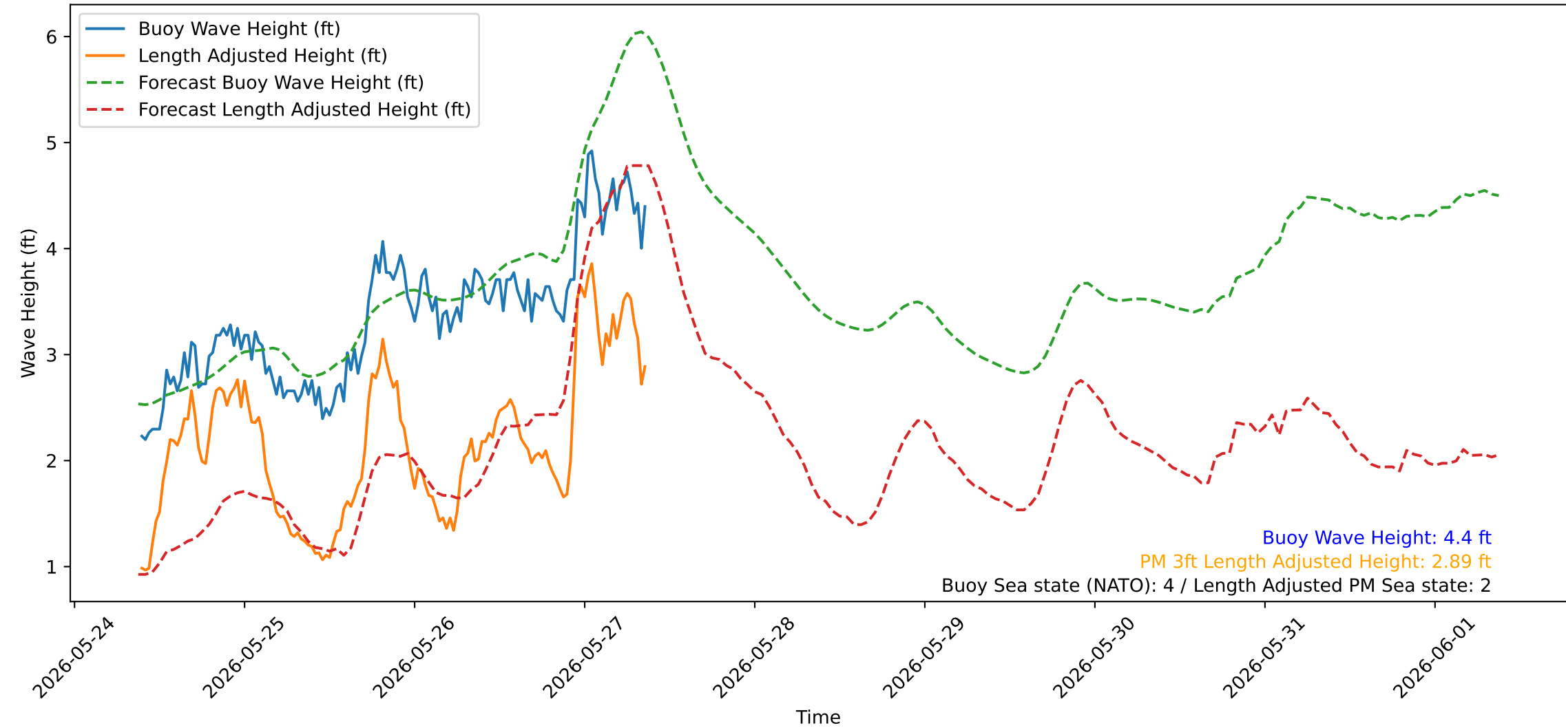
Wave Heights over Time for Green Beach at 2026-05-27 09:21:08
