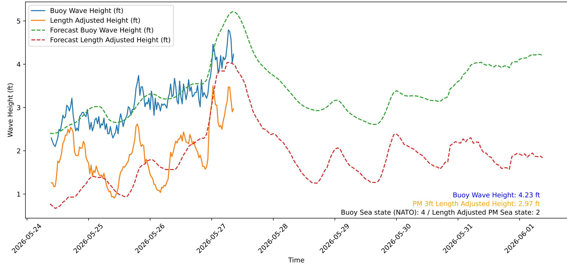
Wave Heights over Time for Red Beach at 2026-05-27 09:20:46
