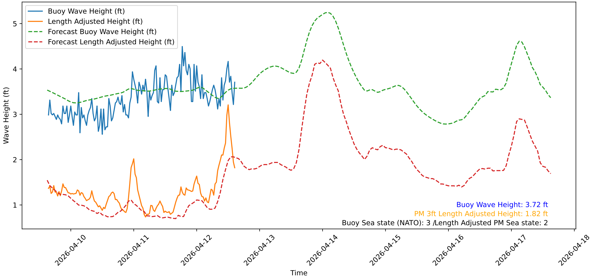
Wave Heights over Time for Green Beach at 2026-04-12 15:21:13
