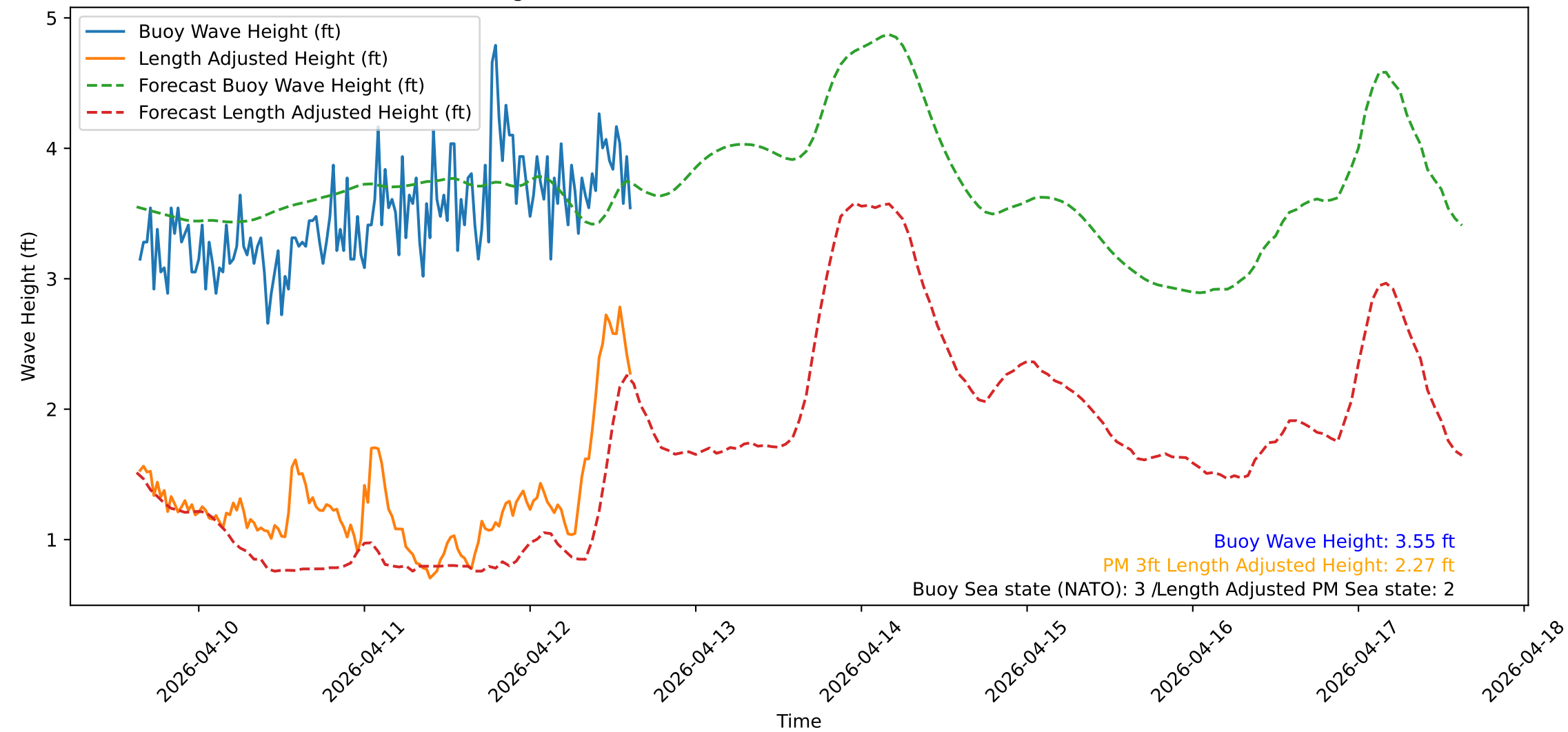
Wave Heights over Time for Oceanside Harbor at 2026-04-12 15:20:31
