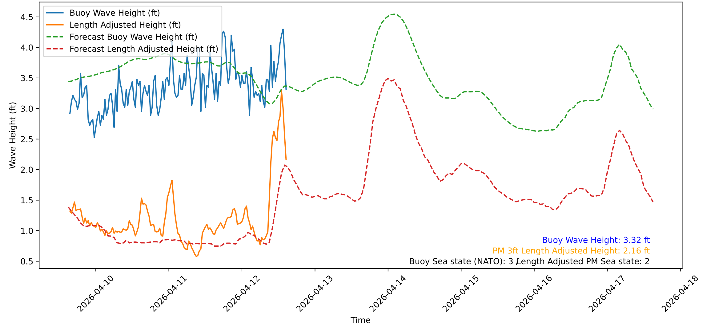
Wave Heights over Time for Red Beach at 2026-04-12 15:20:51
