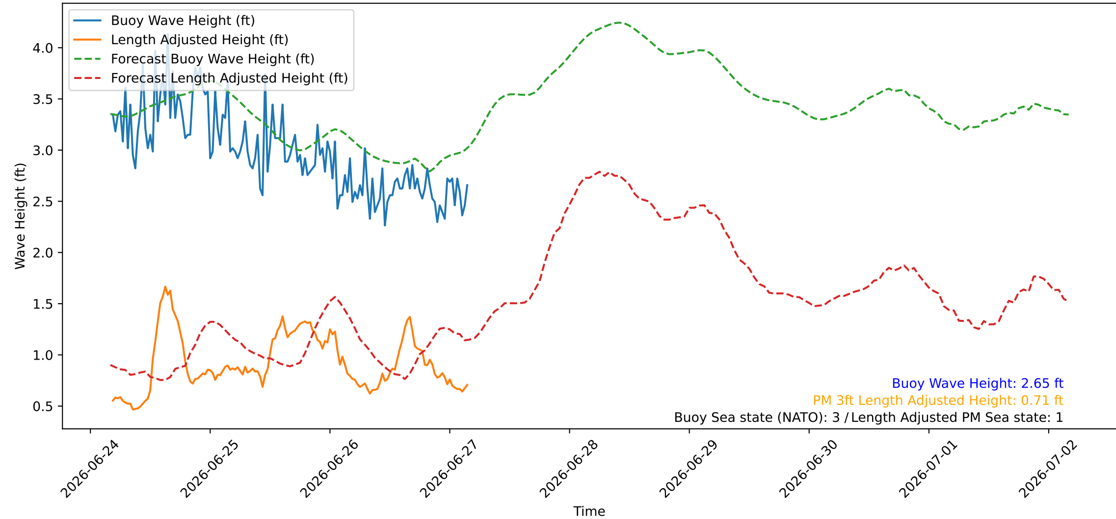
Wave Heights over Time for Red Beach at 2026-06-27 04:20:46
