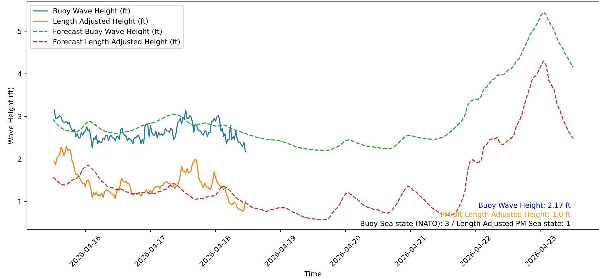
Wave Heights over Time for Red Beach at 2026-04-18 12:20:52
