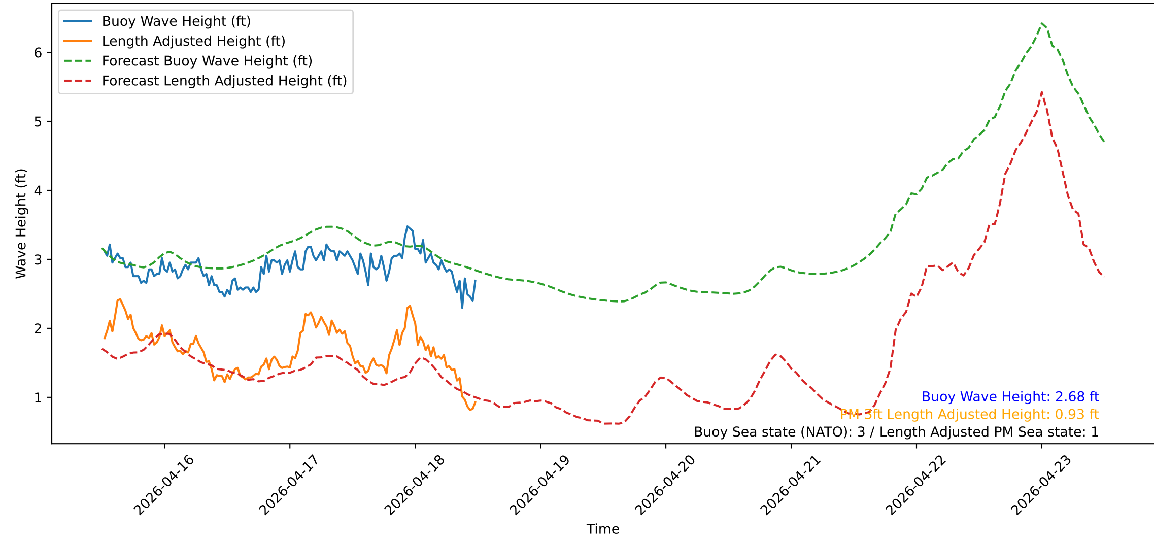
Wave Heights over Time for Green Beach at 2026-04-18 12:21:14
