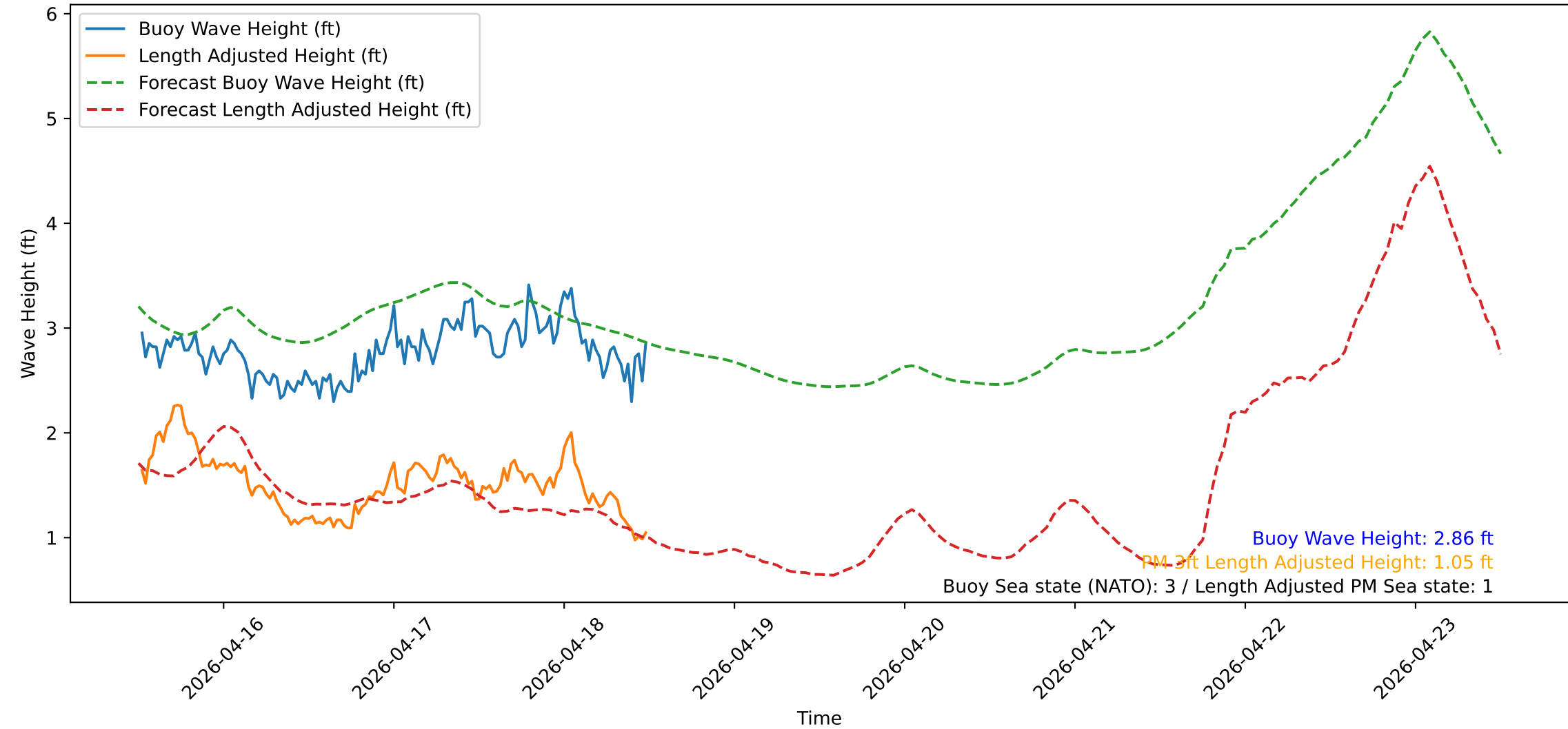
Wave Heights over Time for Oceanside Harbor at 2026-04-18 12:20:31
