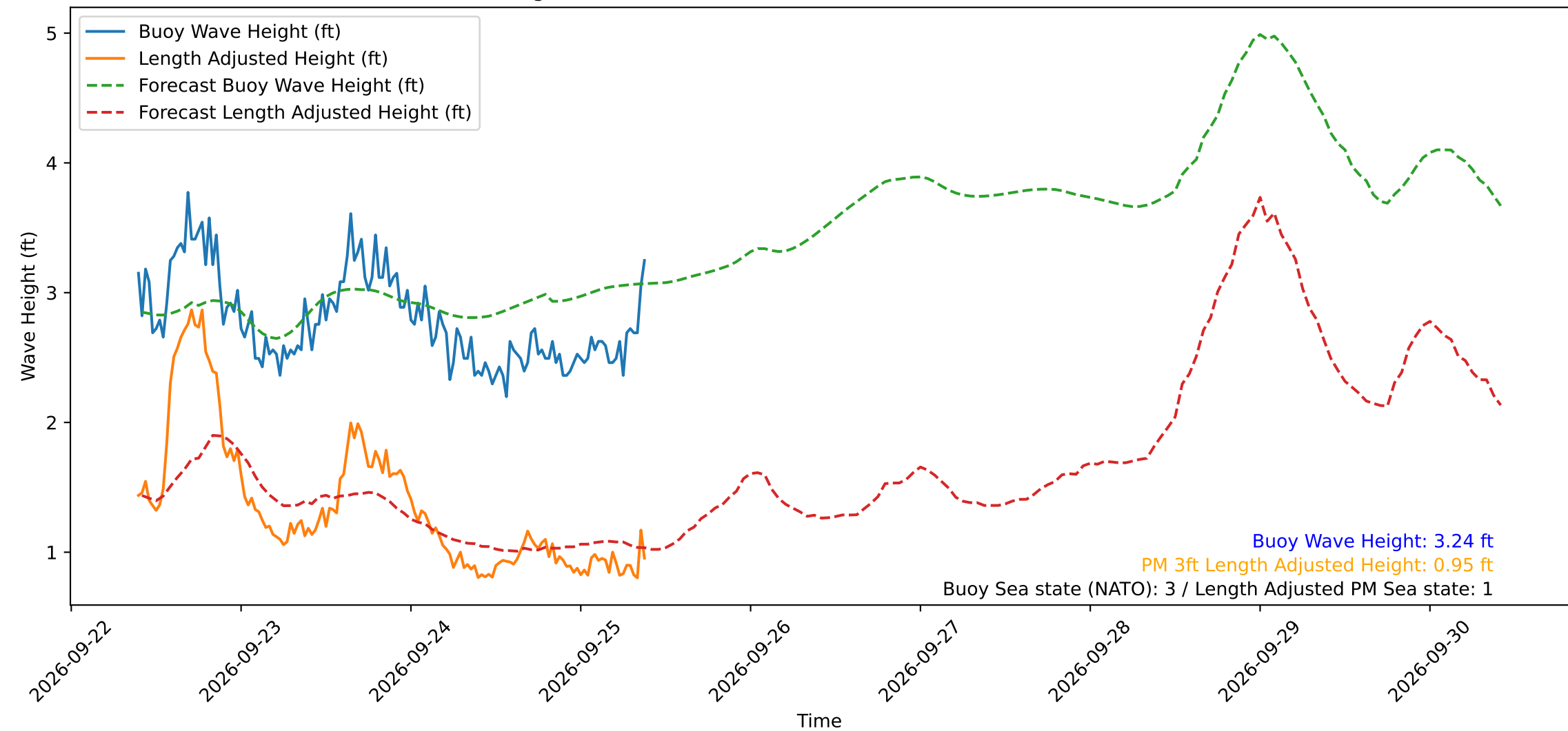
Wave Heights over Time for Oceanside Harbor at 2026-09-25 09:30:30
