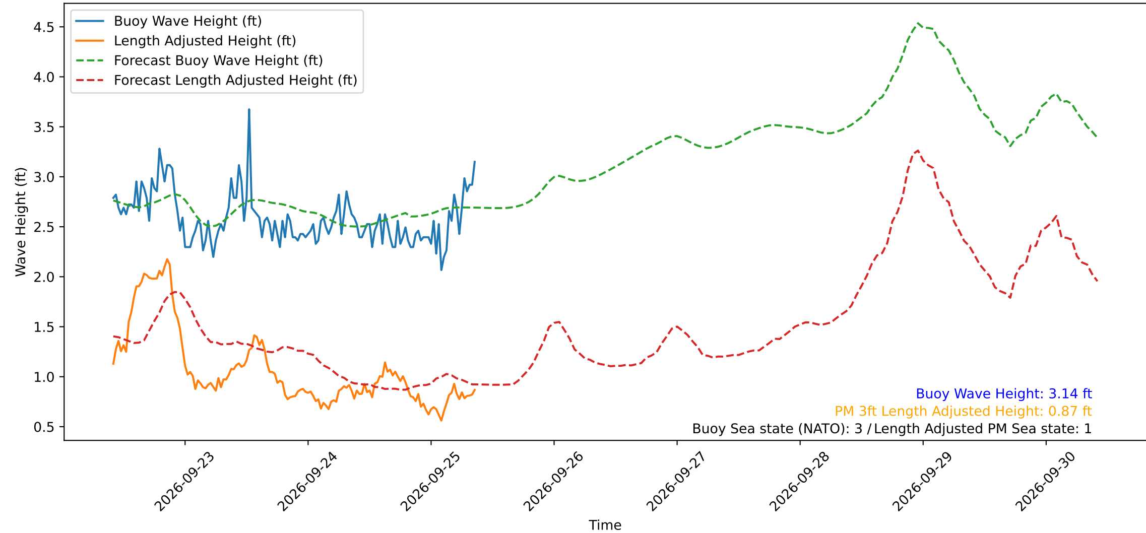
Wave Heights over Time for Red Beach at 2026-09-25 09:30:50
