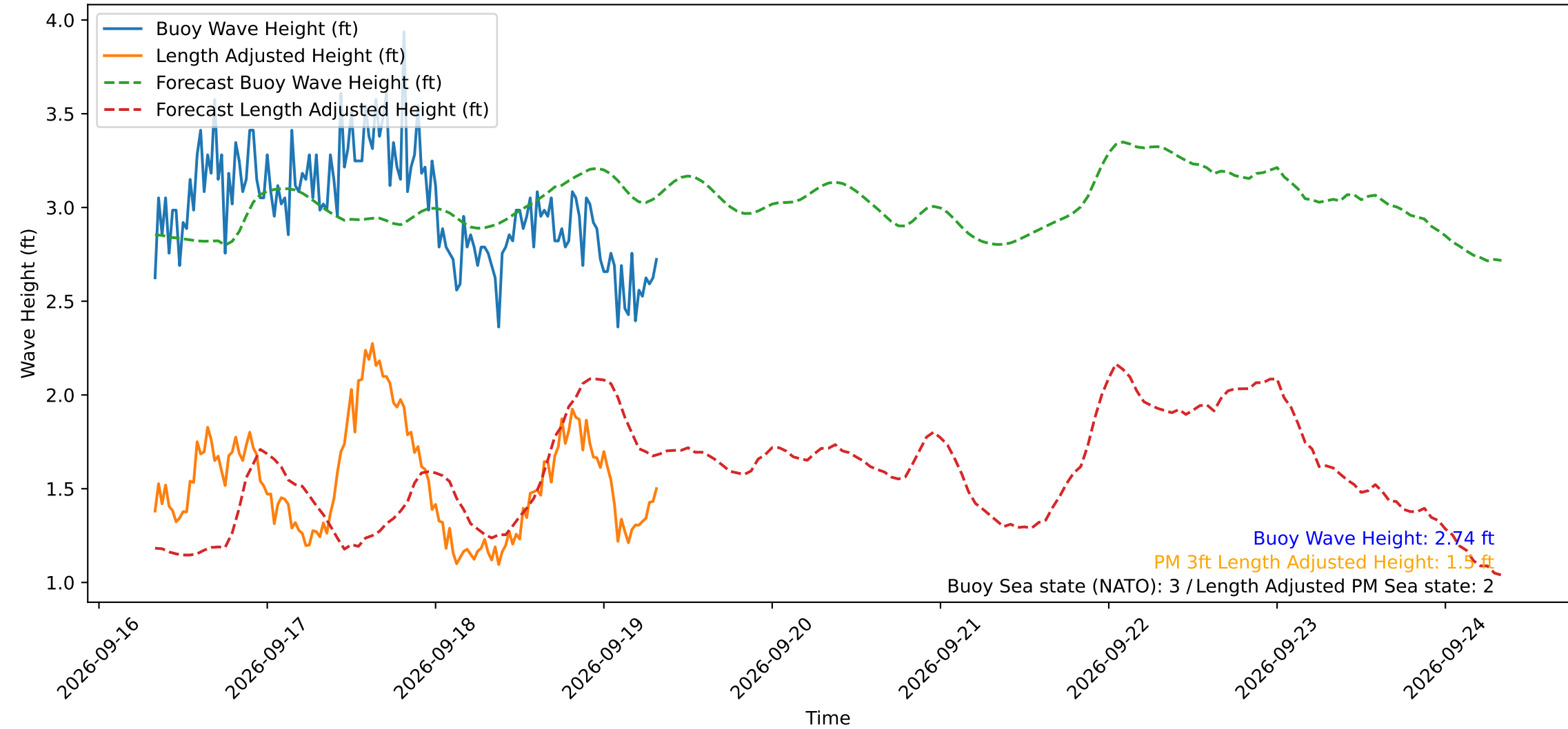
Wave Heights over Time for Oceanside Harbor at 2026-09-19 08:00:30
