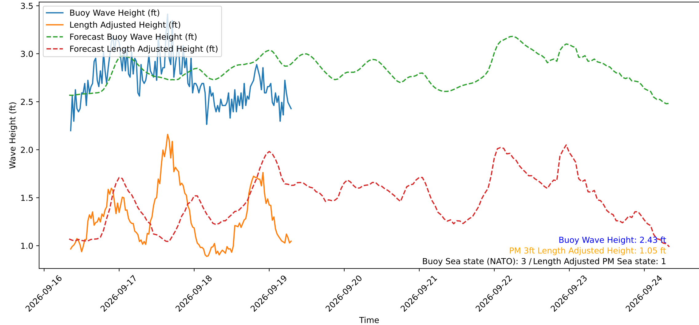
Wave Heights over Time for Red Beach at 2026-09-19 08:00:49
