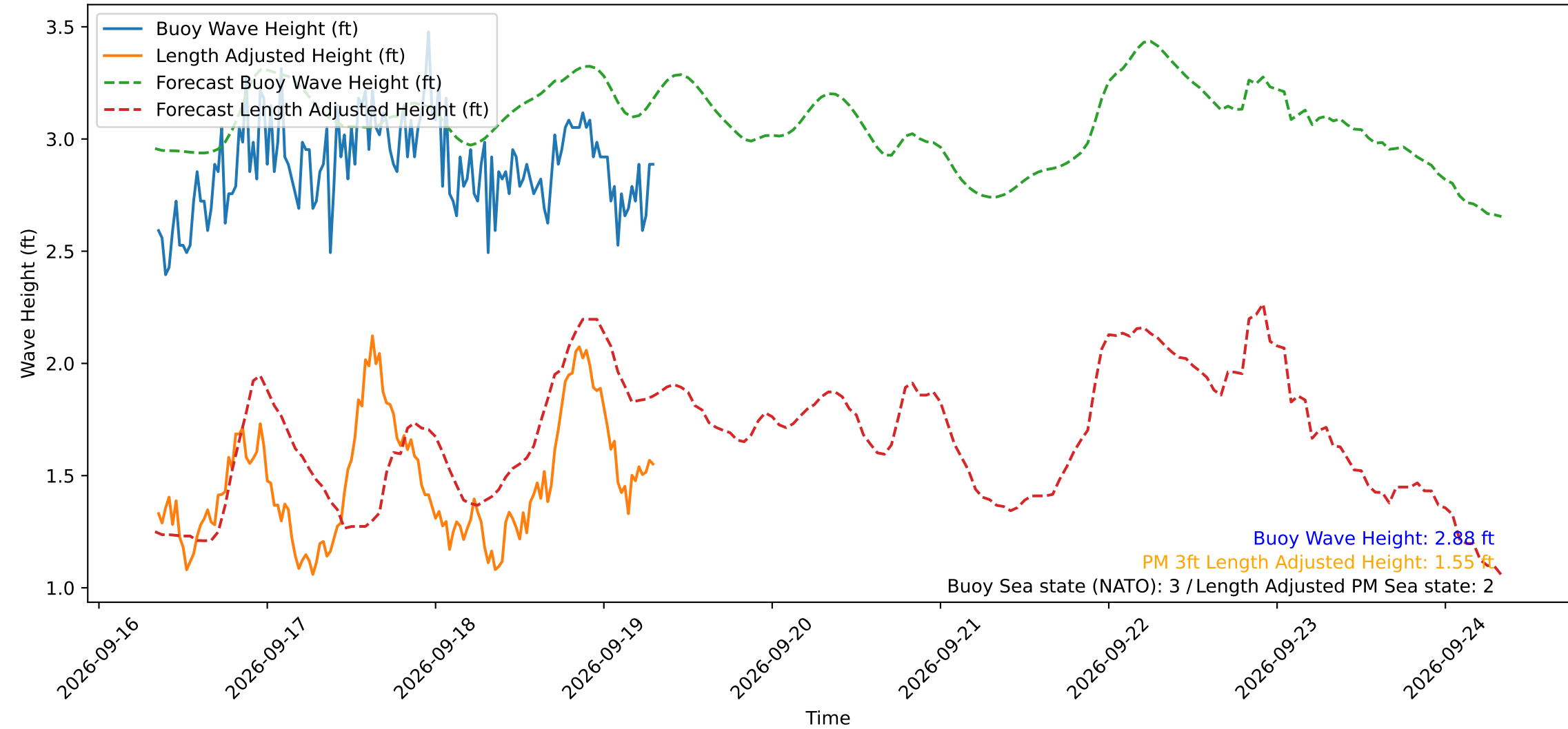
Wave Heights over Time for Green Beach at 2026-09-19 08:01:11
