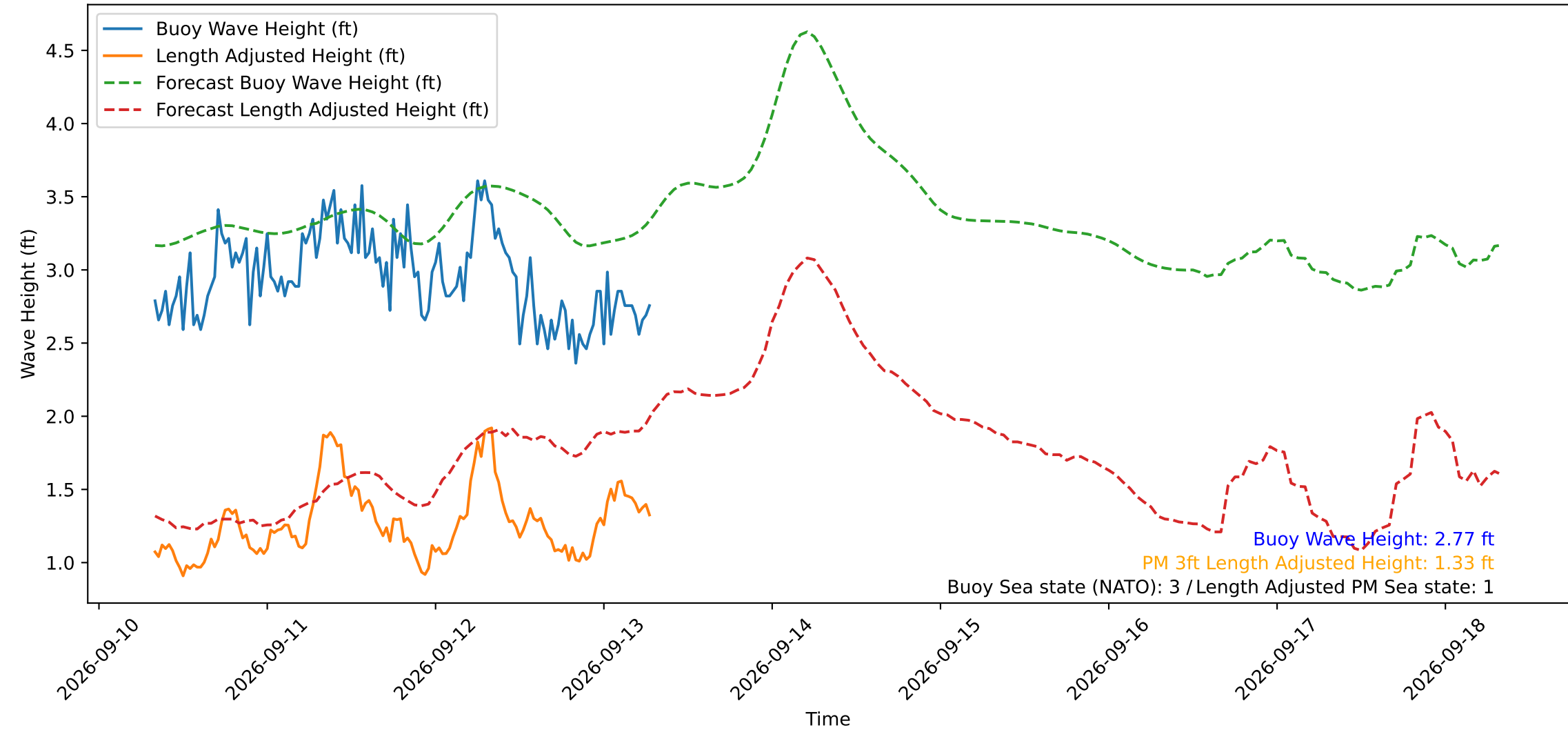
Wave Heights over Time for Green Beach at 2026-09-13 07:31:11
