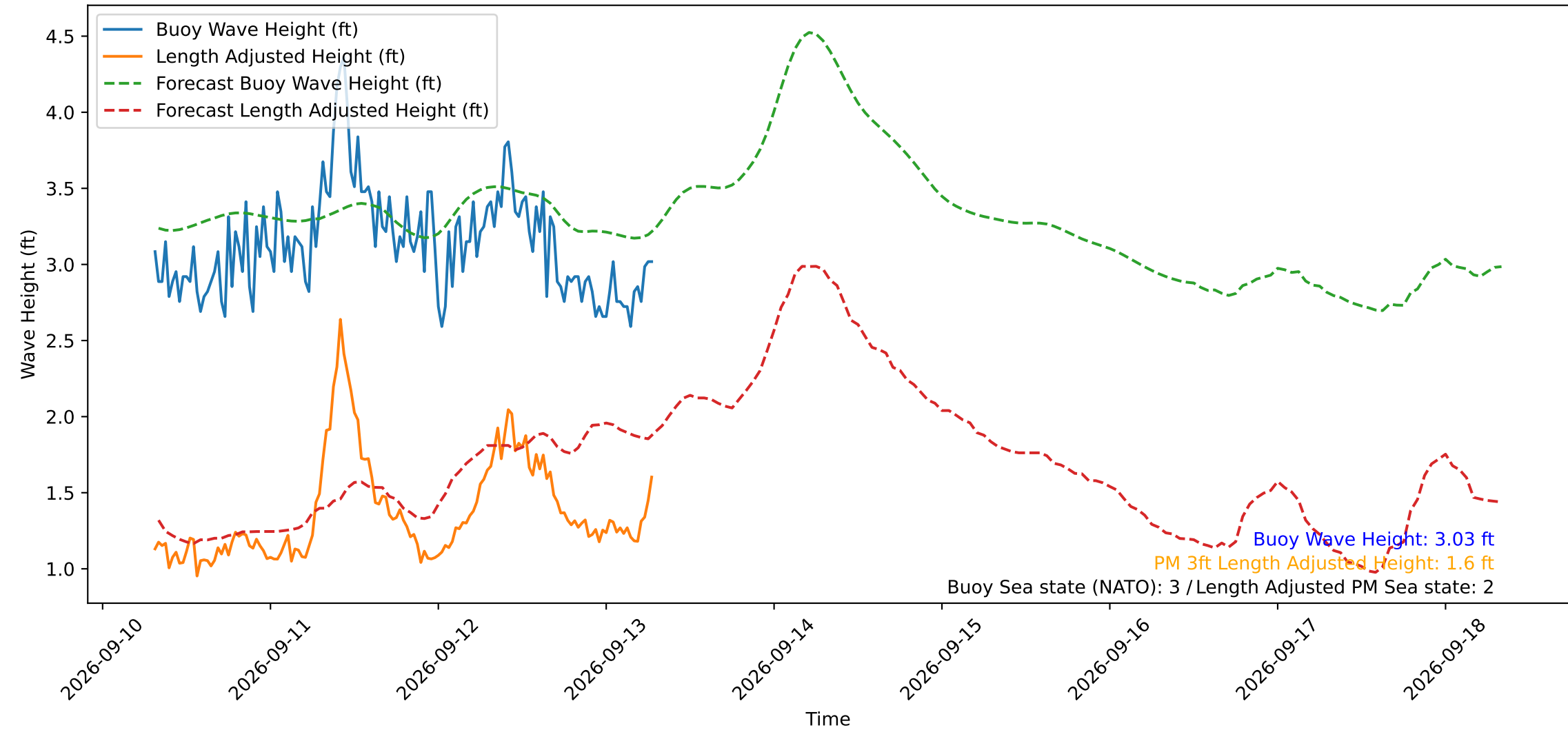
Wave Heights over Time for Oceanside Harbor at 2026-09-13 07:30:29
