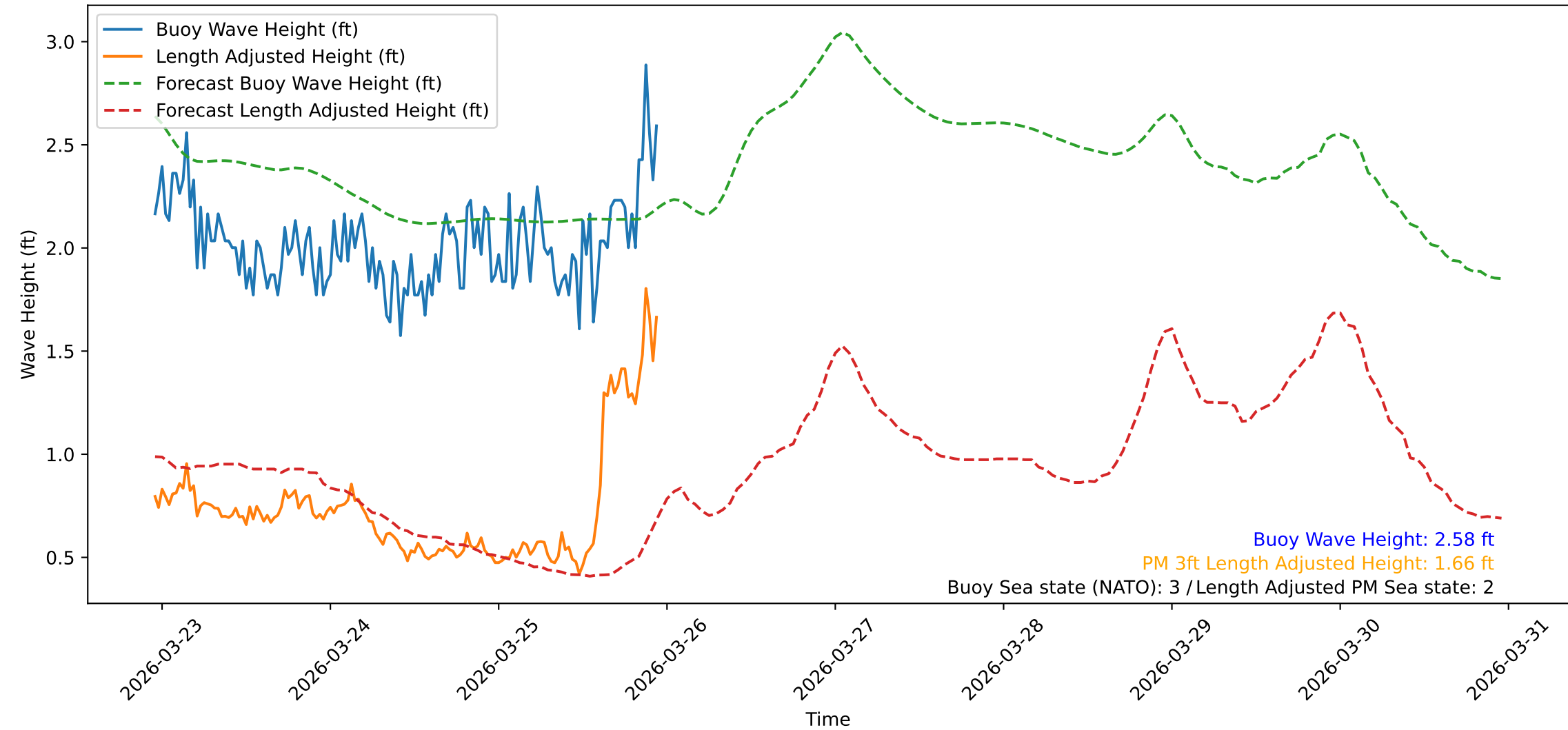
Wave Heights over Time for Oceanside Harbor at 2026-03-25 23:10:31
