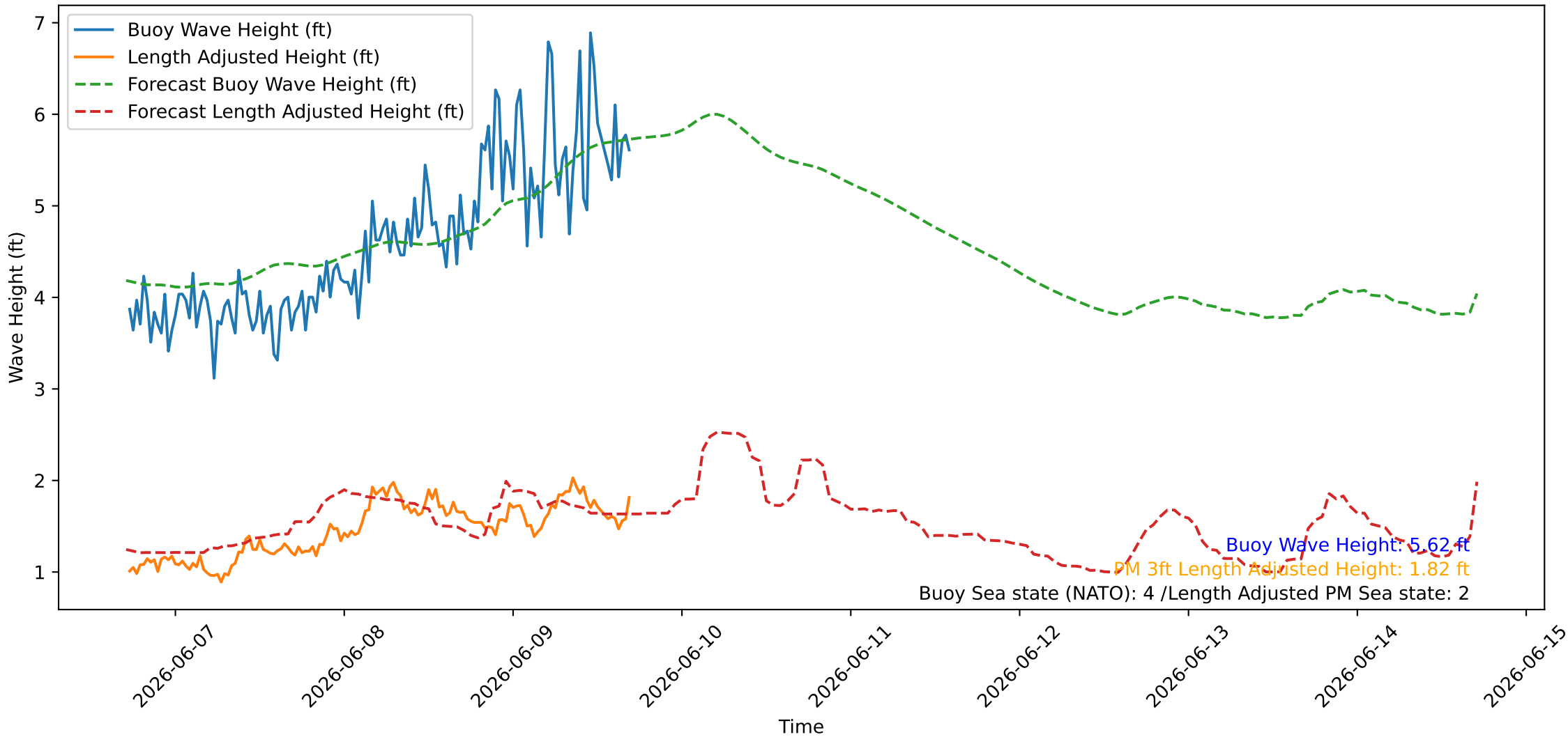
Wave Heights over Time for Green Beach at 2026-06-09 17:21:09
