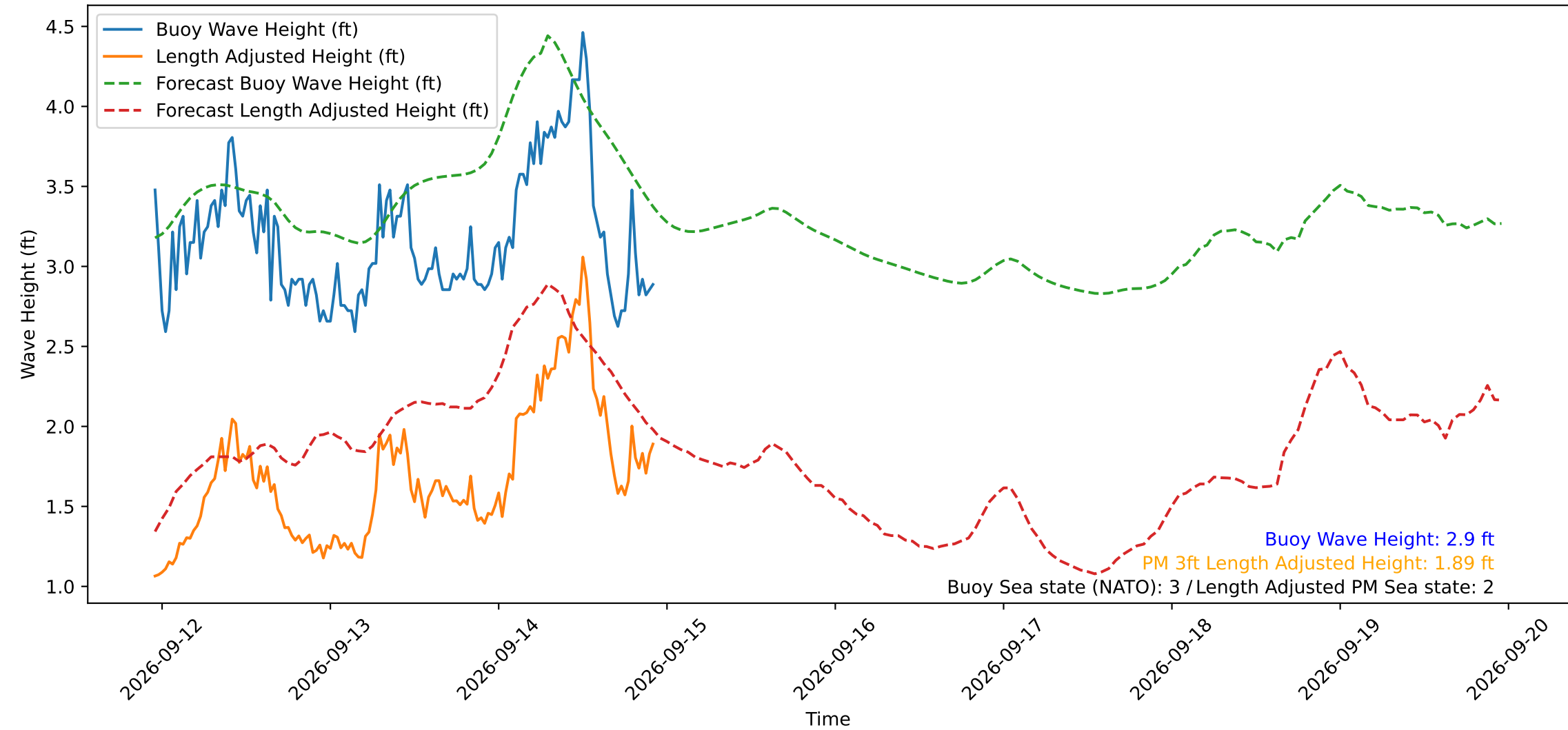
Wave Heights over Time for Oceanside Harbor at 2026-09-14 22:50:29
