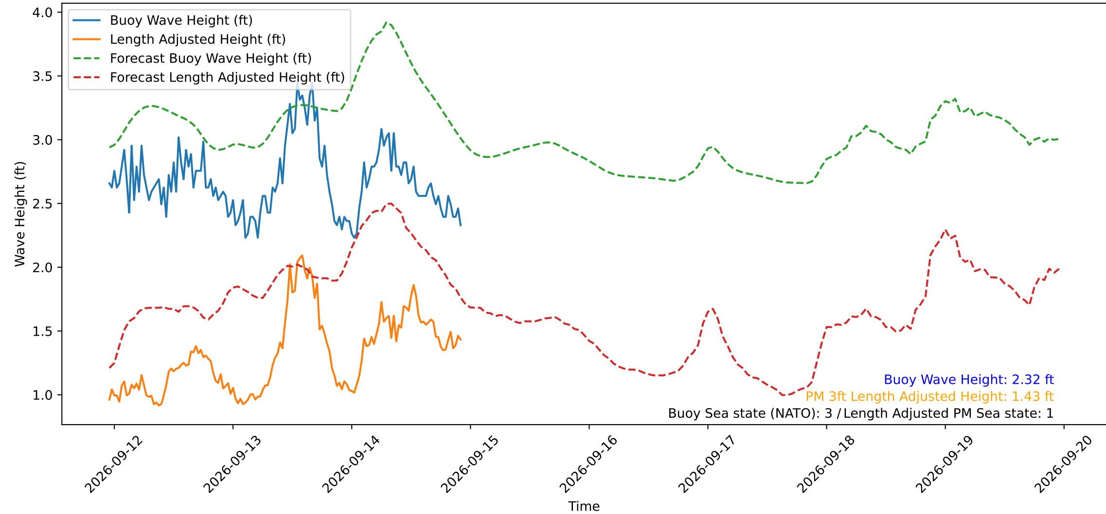
Wave Heights over Time for Red Beach at 2026-09-14 22:50:49
