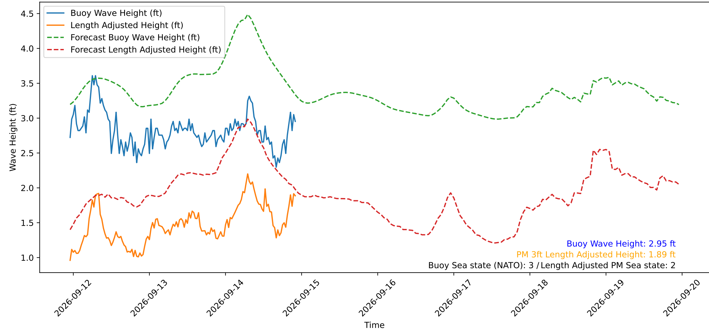
Wave Heights over Time for Green Beach at 2026-09-14 22:51:13
