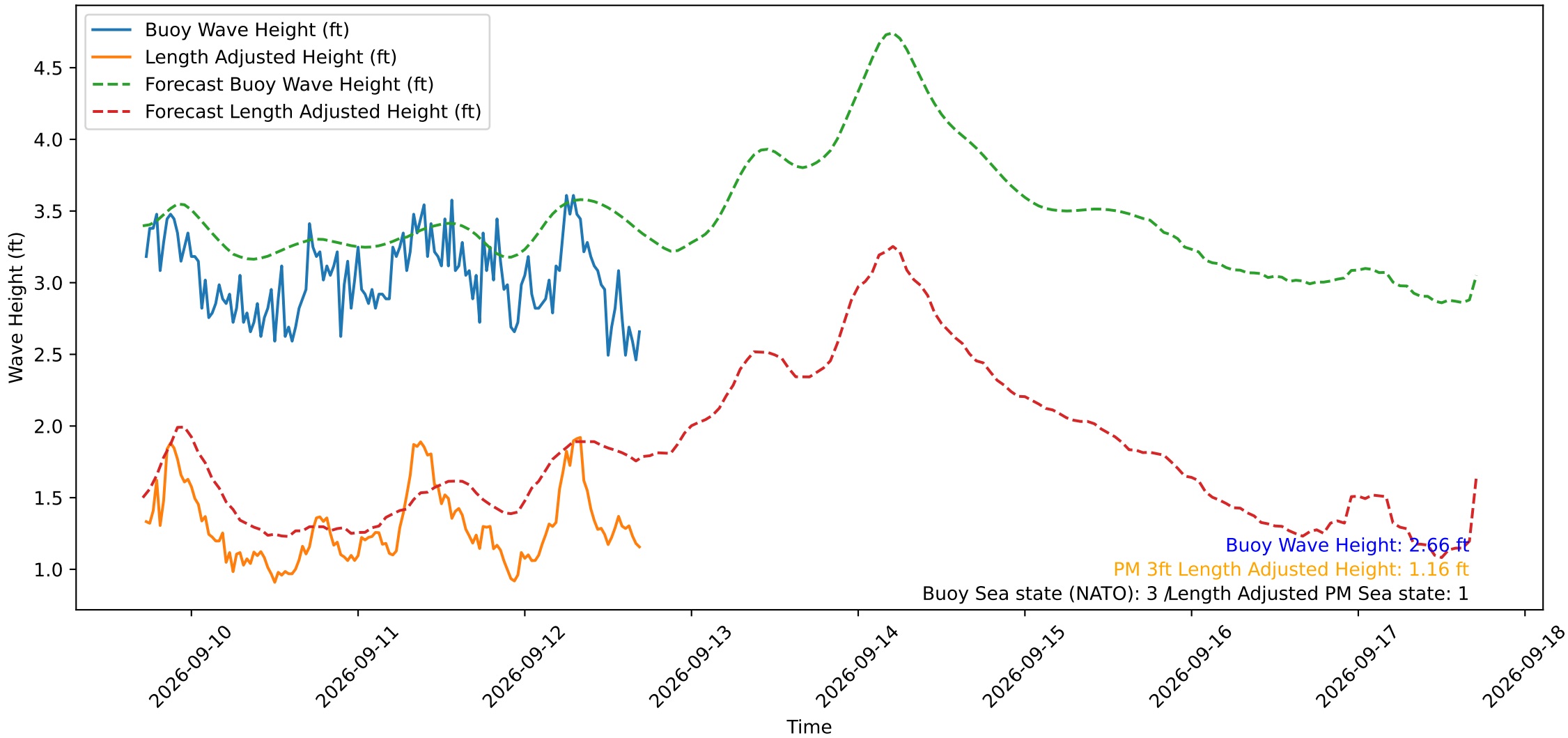
Wave Heights over Time for Green Beach at 2026-09-12 17:21:14
