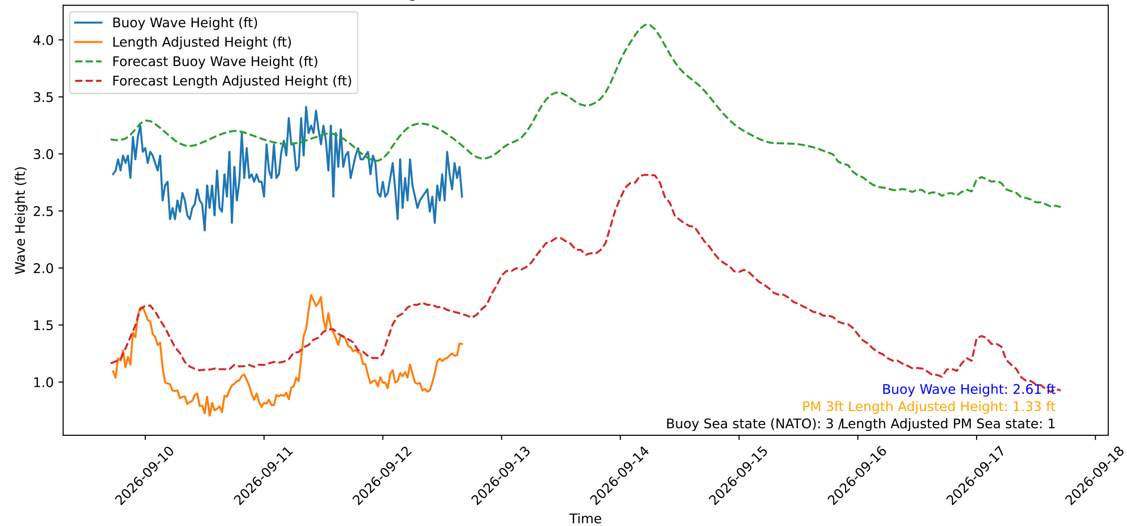
Wave Heights over Time for Red Beach at 2026-09-12 17:20:50
