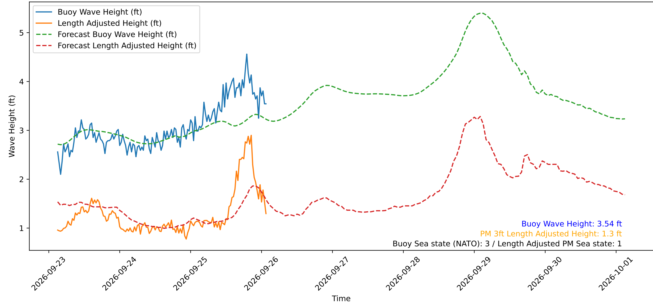
Wave Heights over Time for Green Beach at 2026-09-26 02:31:12
