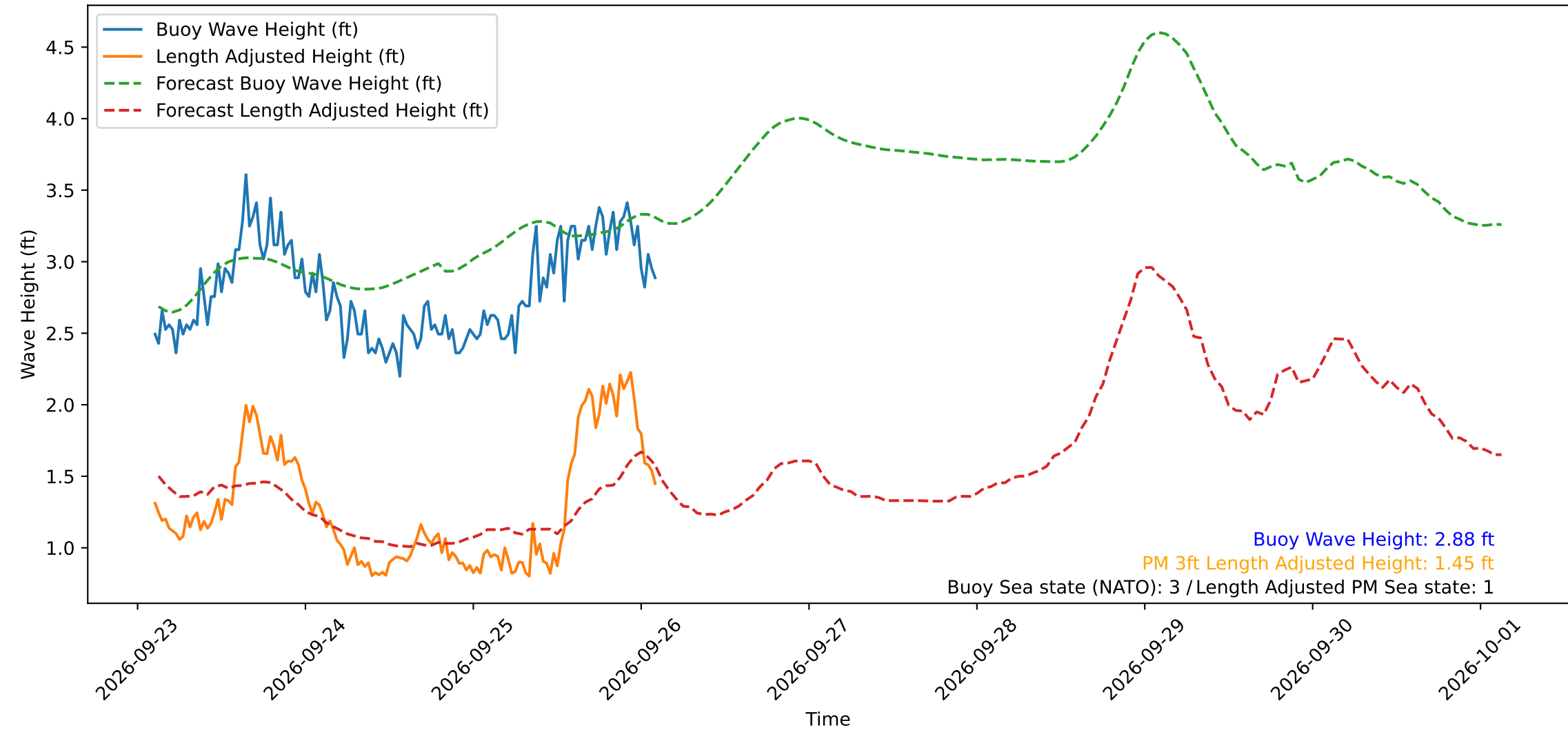
Wave Heights over Time for Oceanside Harbor at 2026-09-26 02:30:30
