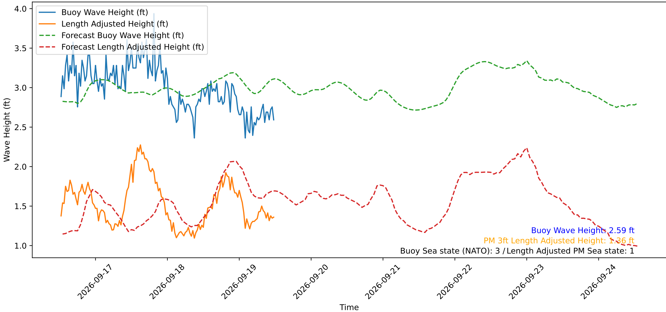
Wave Heights over Time for Oceanside Harbor at 2026-09-19 12:30:30
