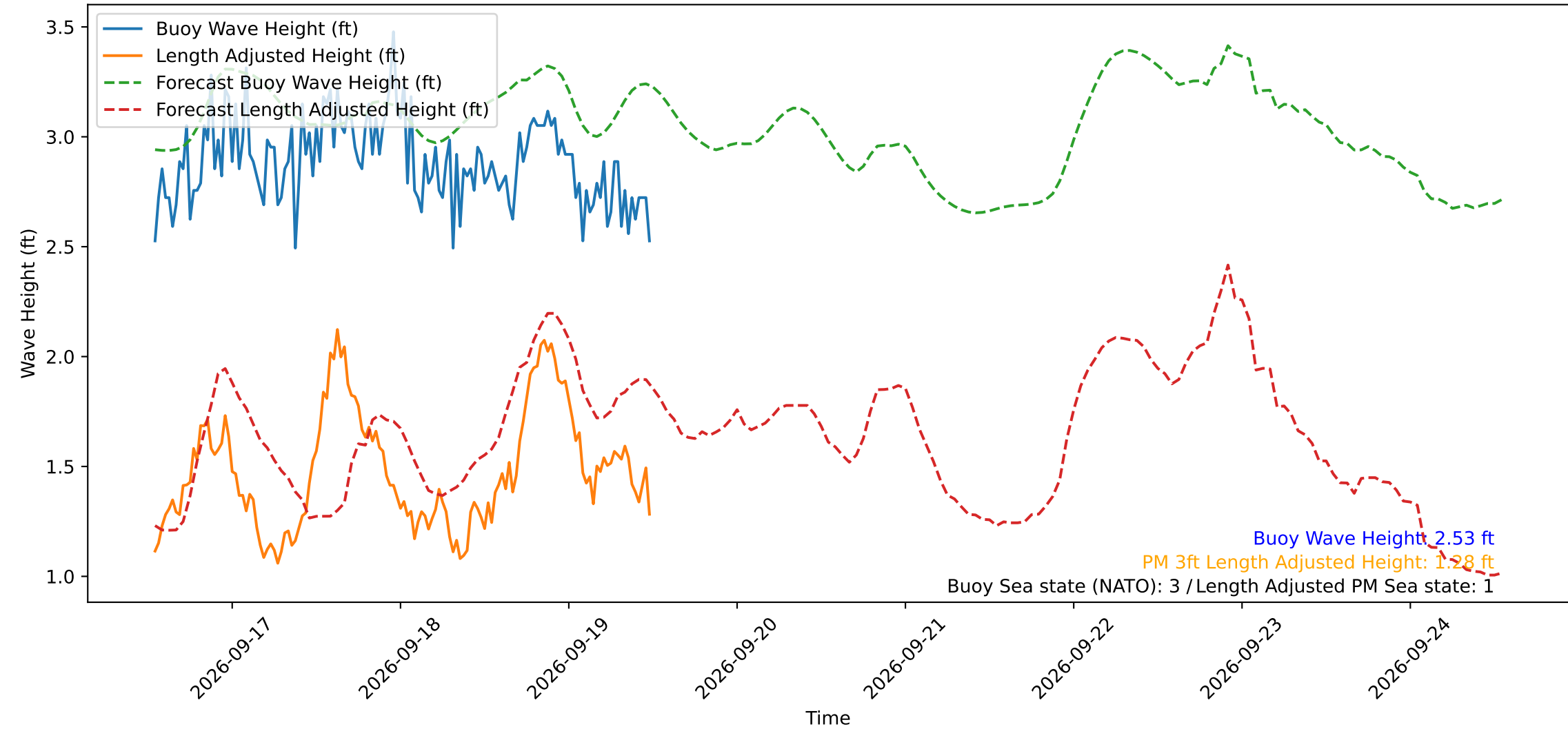
Wave Heights over Time for Green Beach at 2026-09-19 12:31:12
