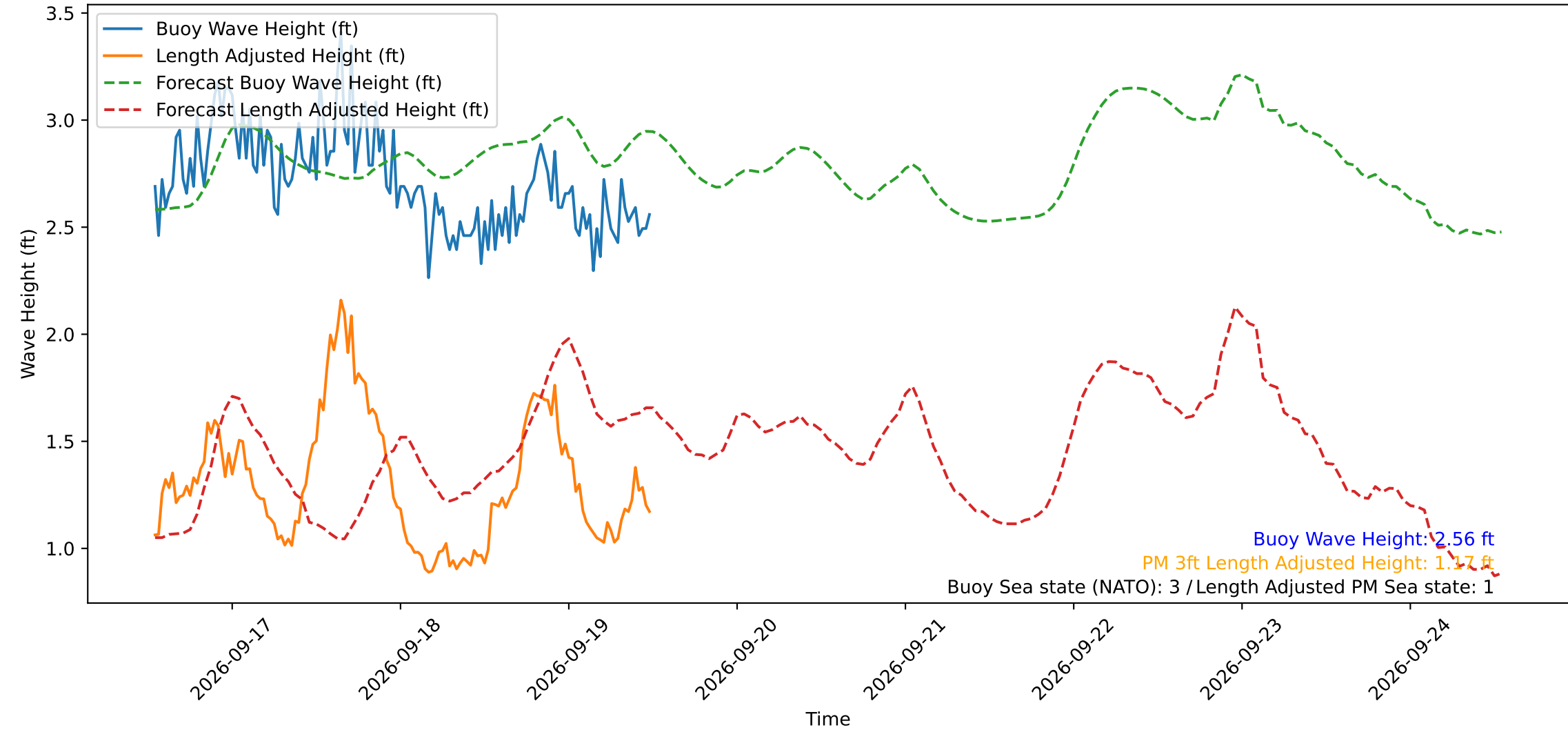
Wave Heights over Time for Red Beach at 2026-09-19 12:30:50
