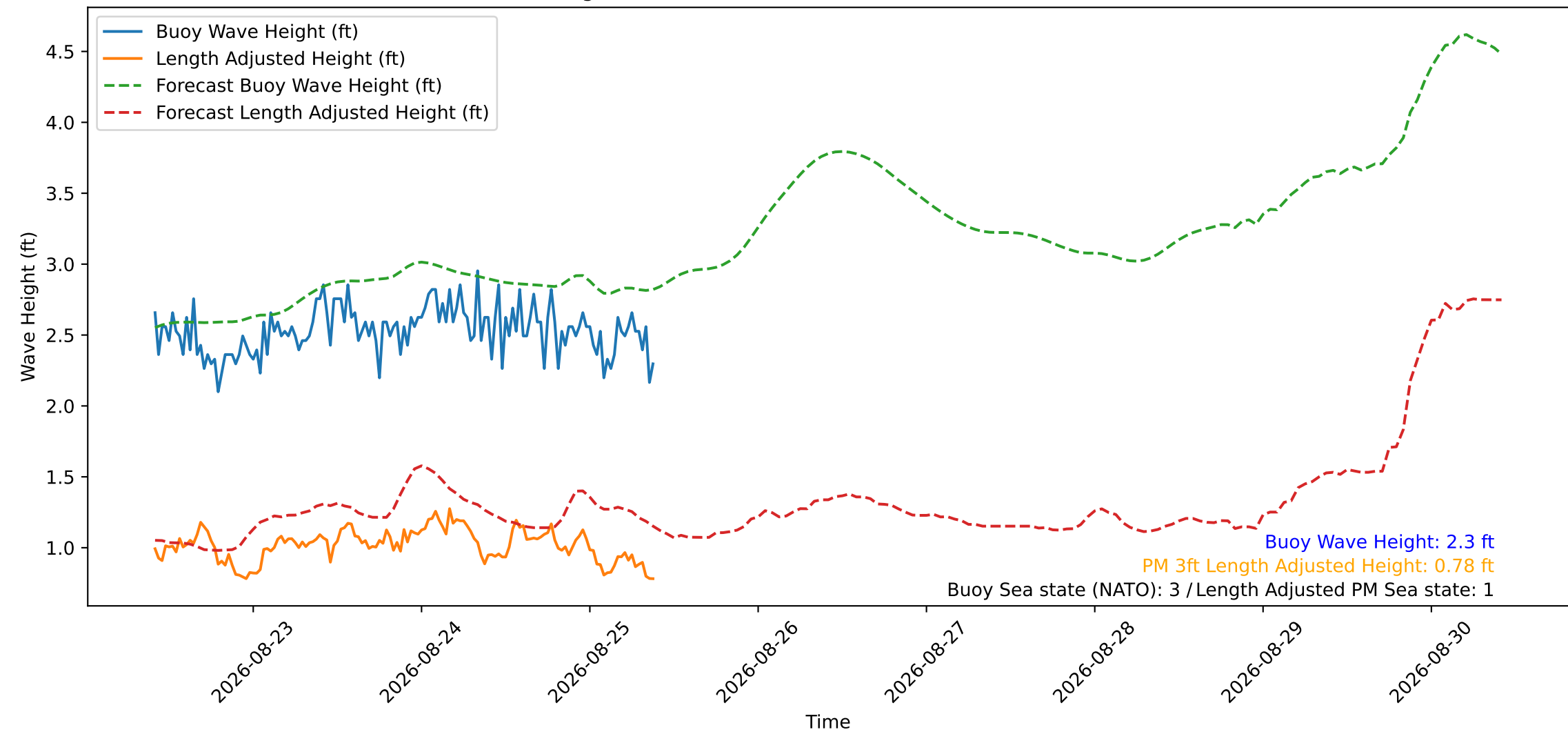
Wave Heights over Time for Red Beach at 2026-08-25 09:50:50
