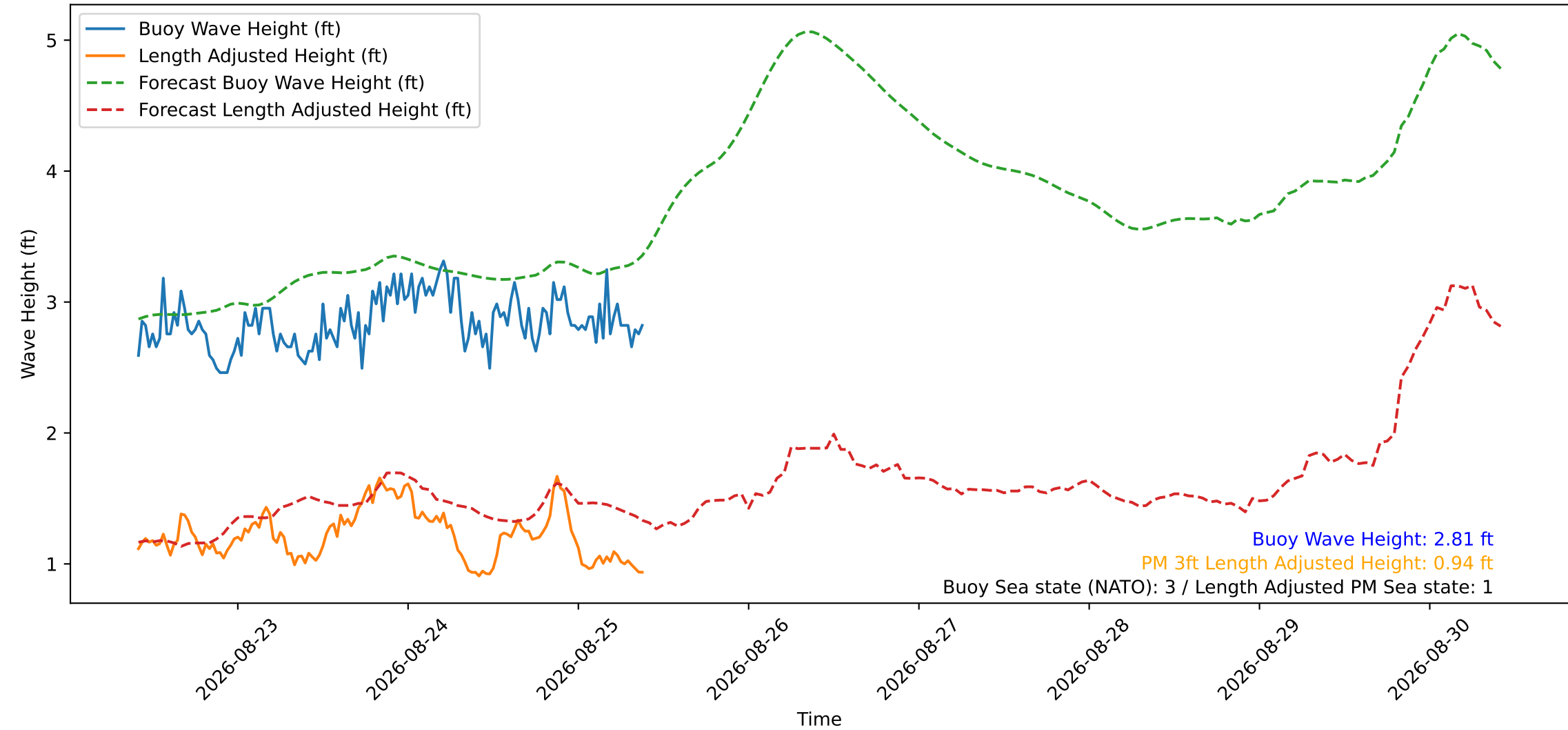
Wave Heights over Time for Green Beach at 2026-08-25 09:51:14
