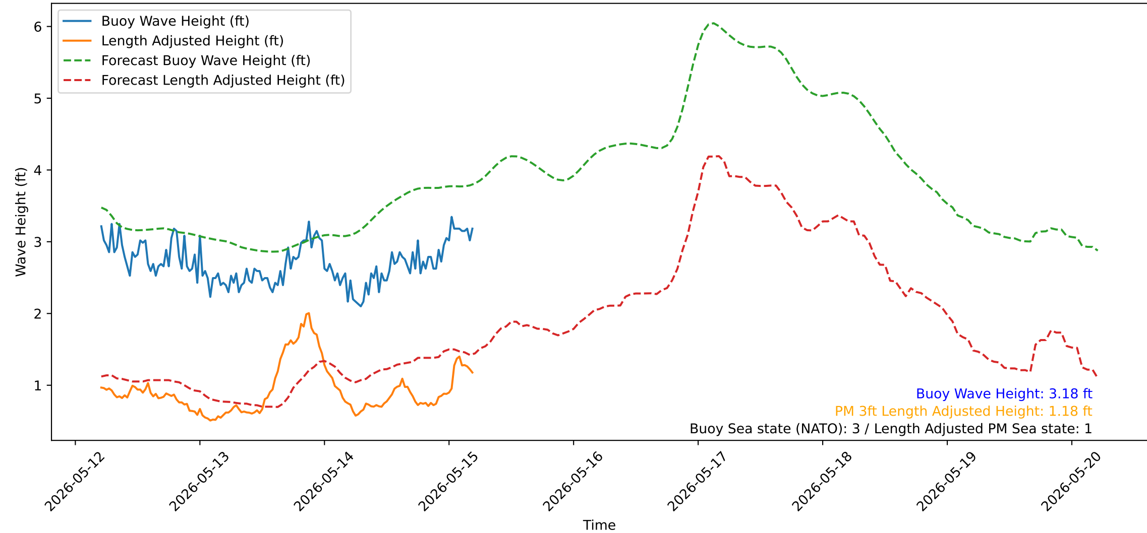
Wave Heights over Time for Green Beach at 2026-05-15 05:11:22
