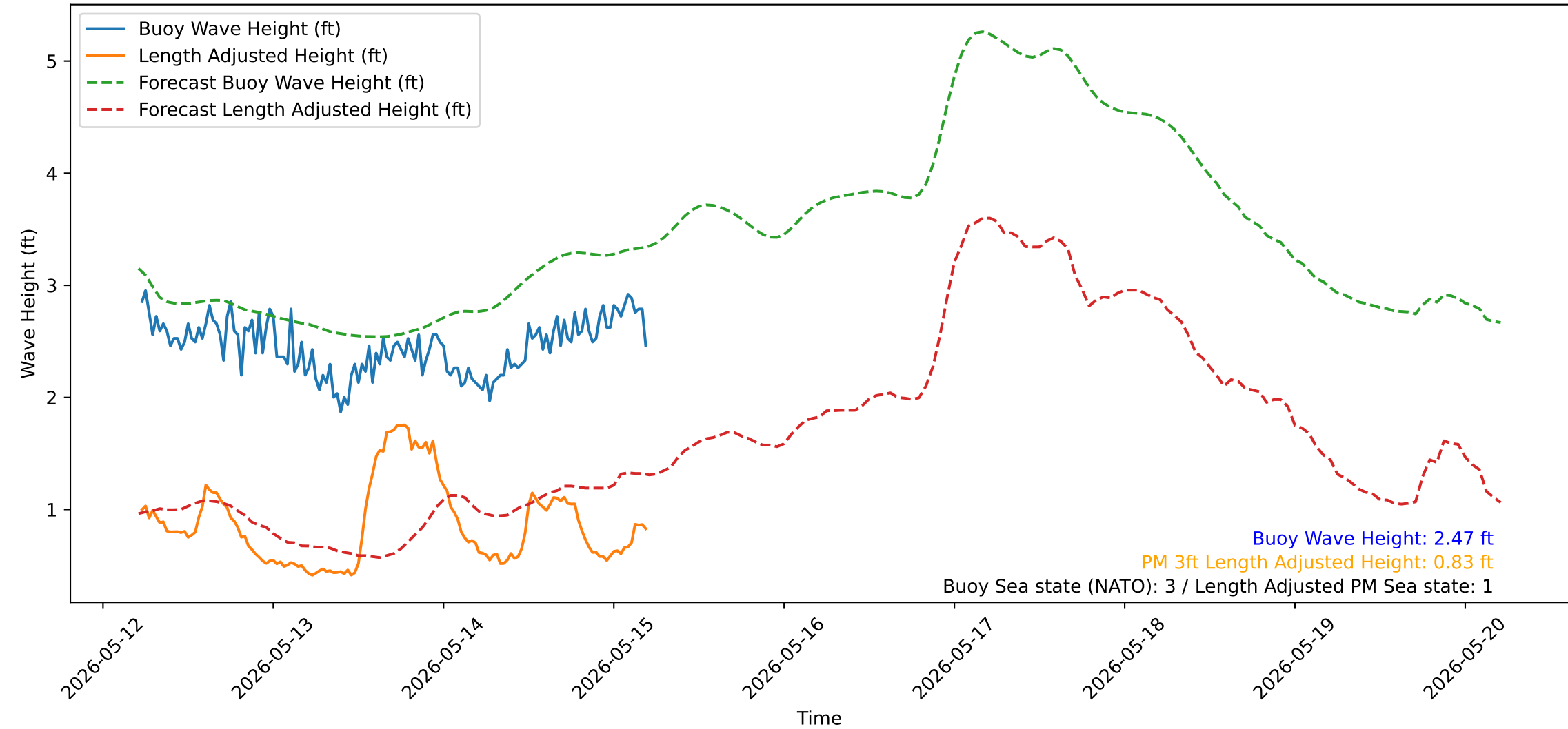
Wave Heights over Time for Red Beach at 2026-05-15 05:10:57
