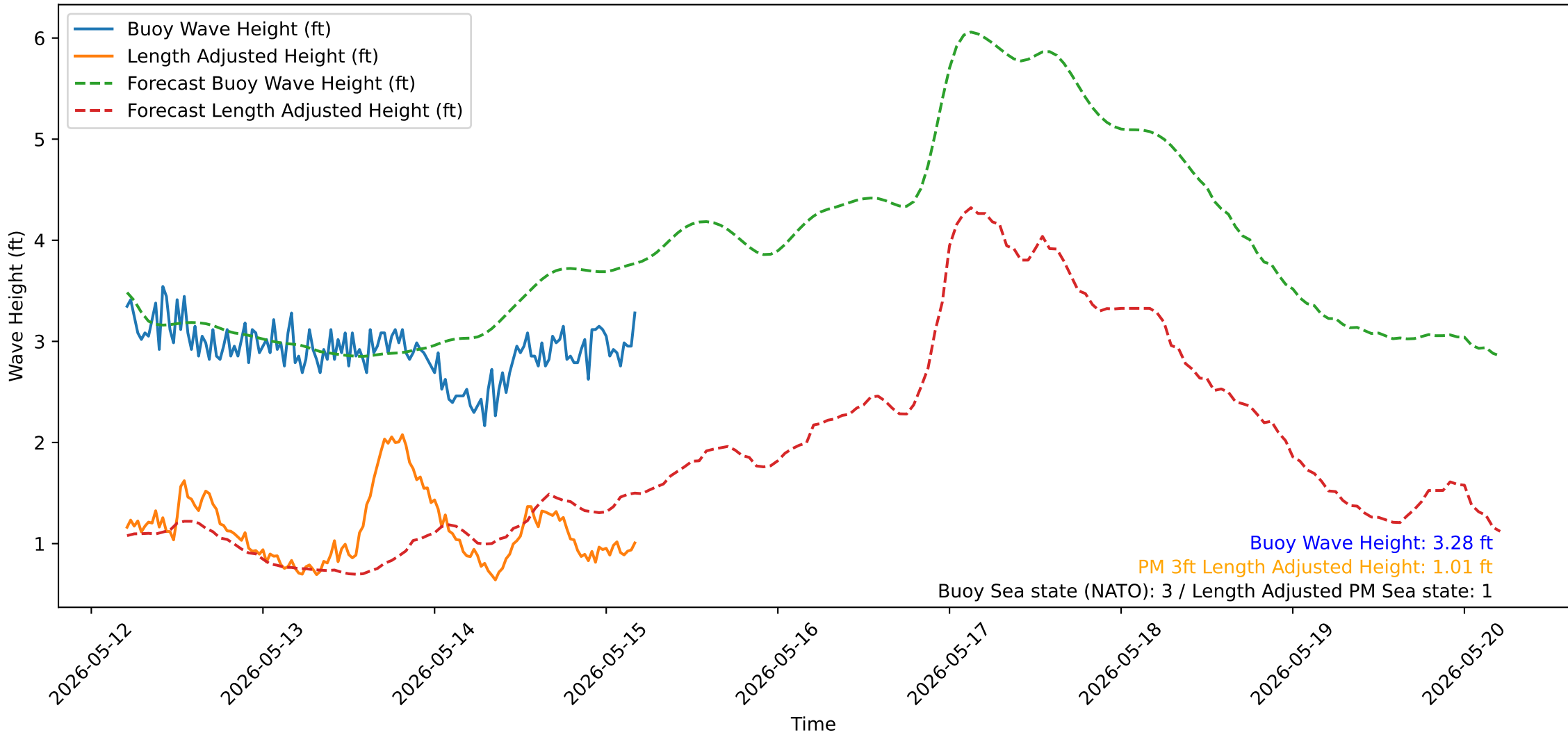
Wave Heights over Time for Oceanside Harbor at 2026-05-15 05:10:35
