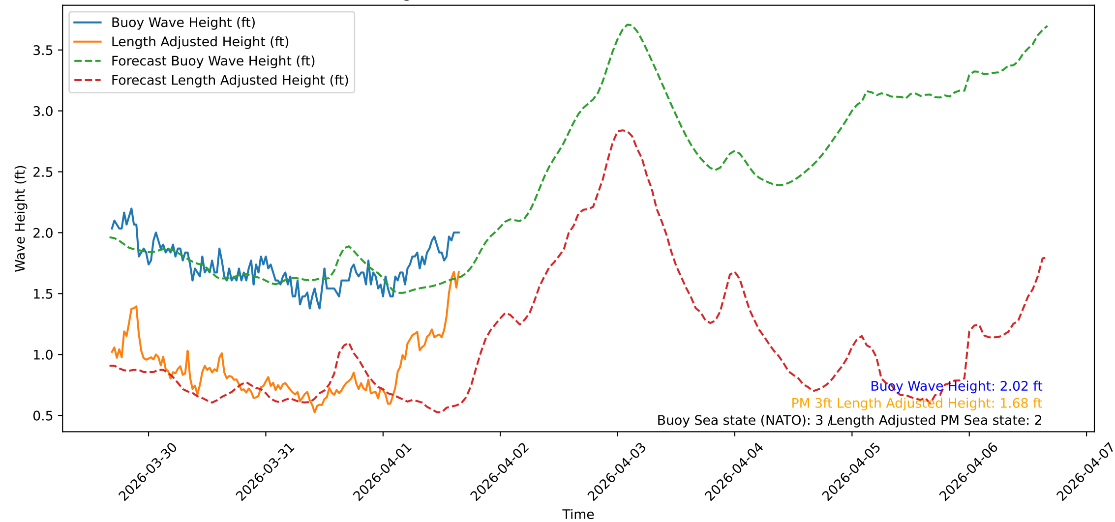
Wave Heights over Time for Red Beach at 2026-04-01 16:10:47
