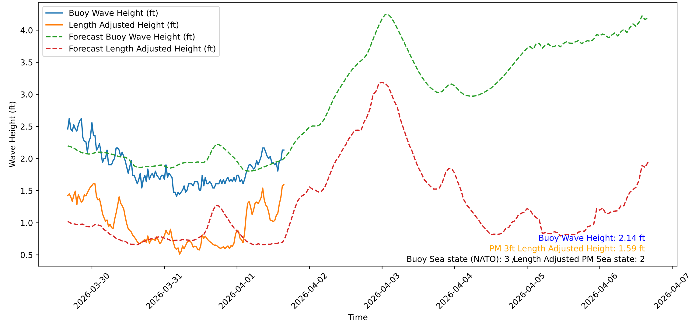
Wave Heights over Time for Green Beach at 2026-04-01 16:11:10
