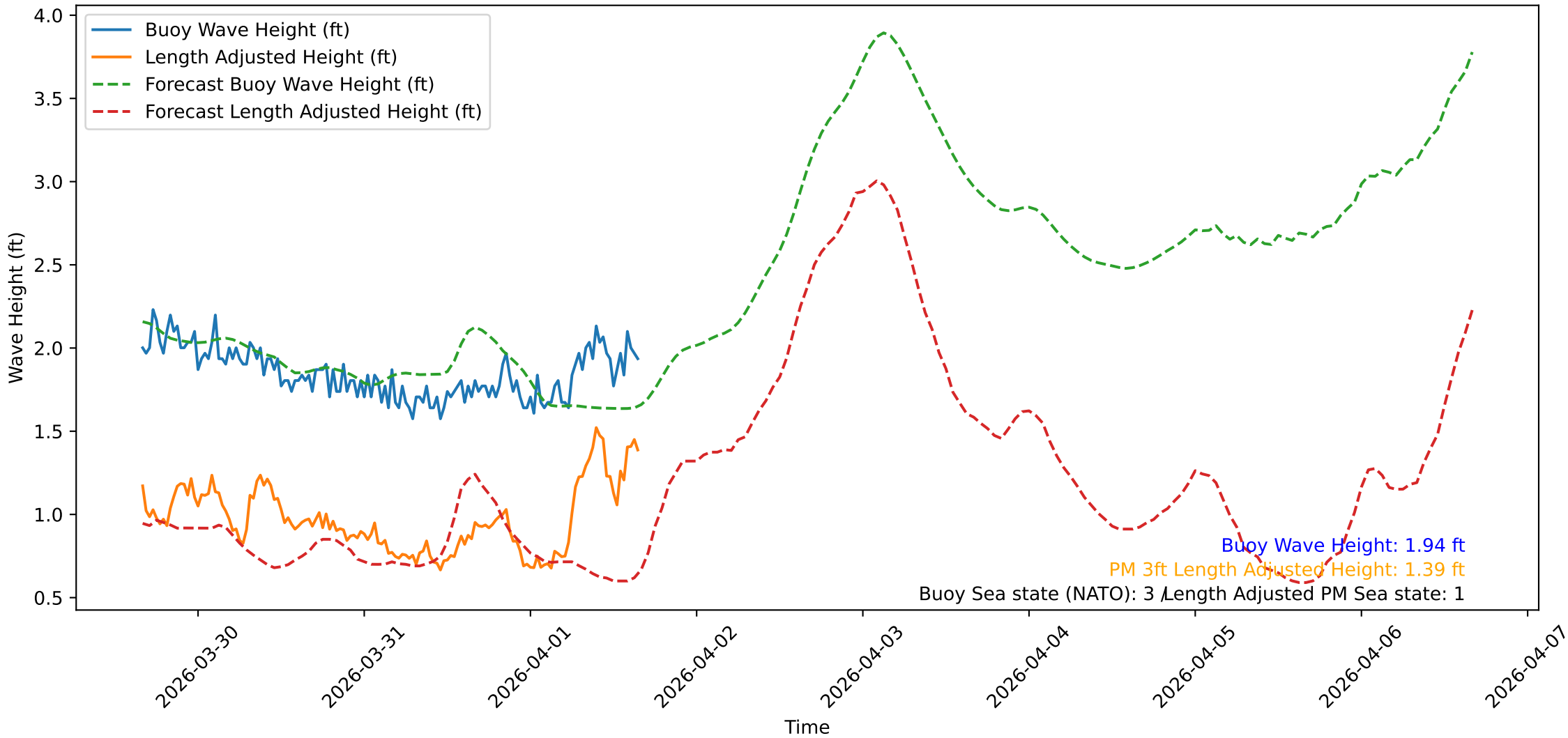
Wave Heights over Time for Oceanside Harbor at 2026-04-01 16:10:31
