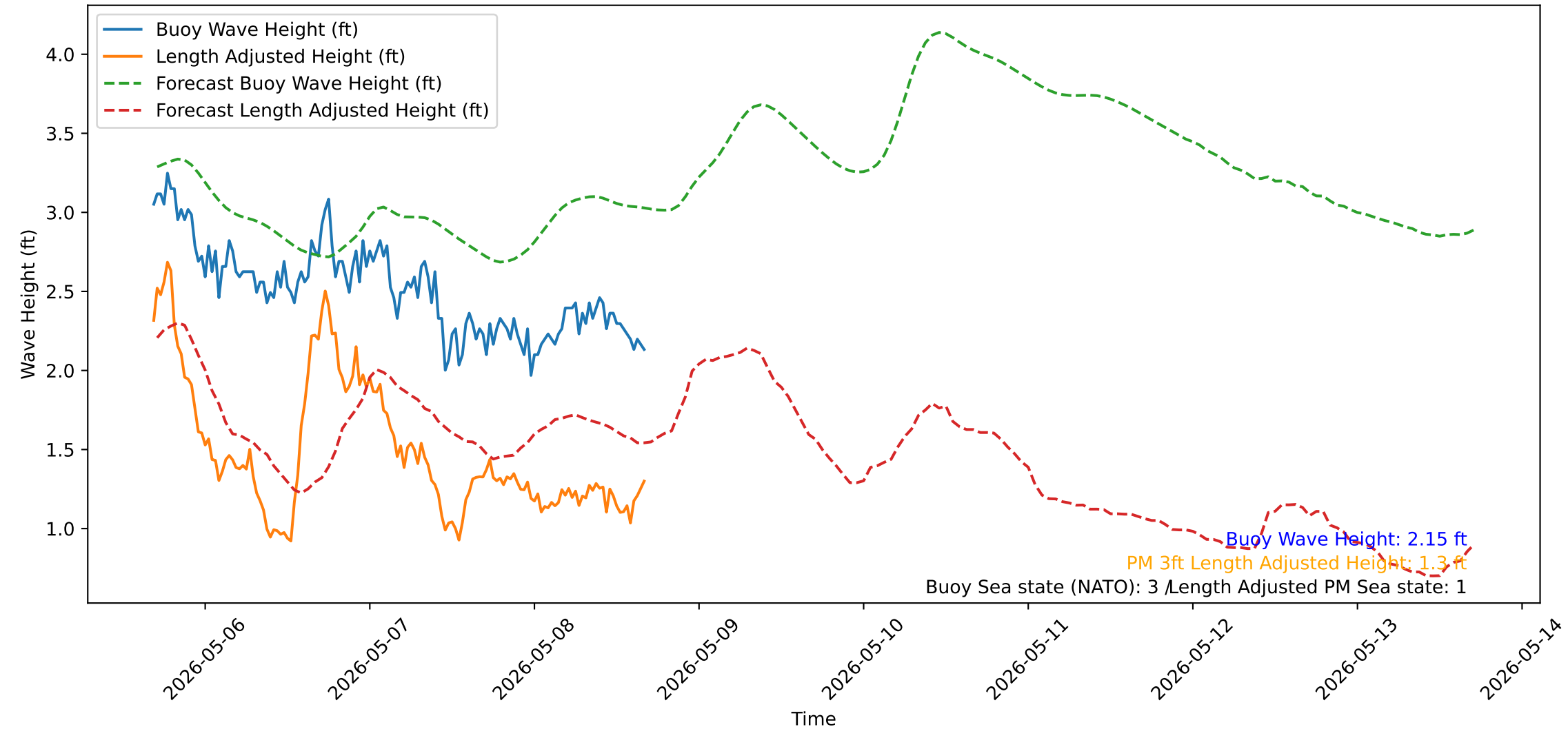
Wave Heights over Time for Oceanside Harbor at 2026-05-08 16:40:31
