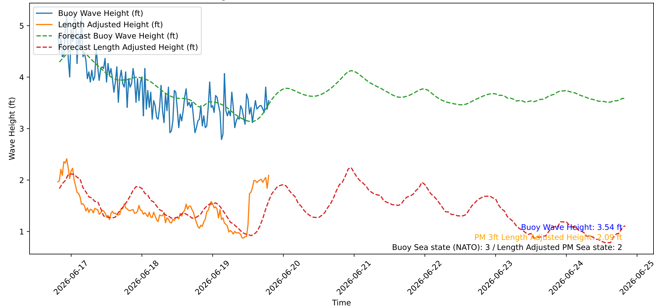
Wave Heights over Time for Oceanside Harbor at 2026-06-19 19:30:26
