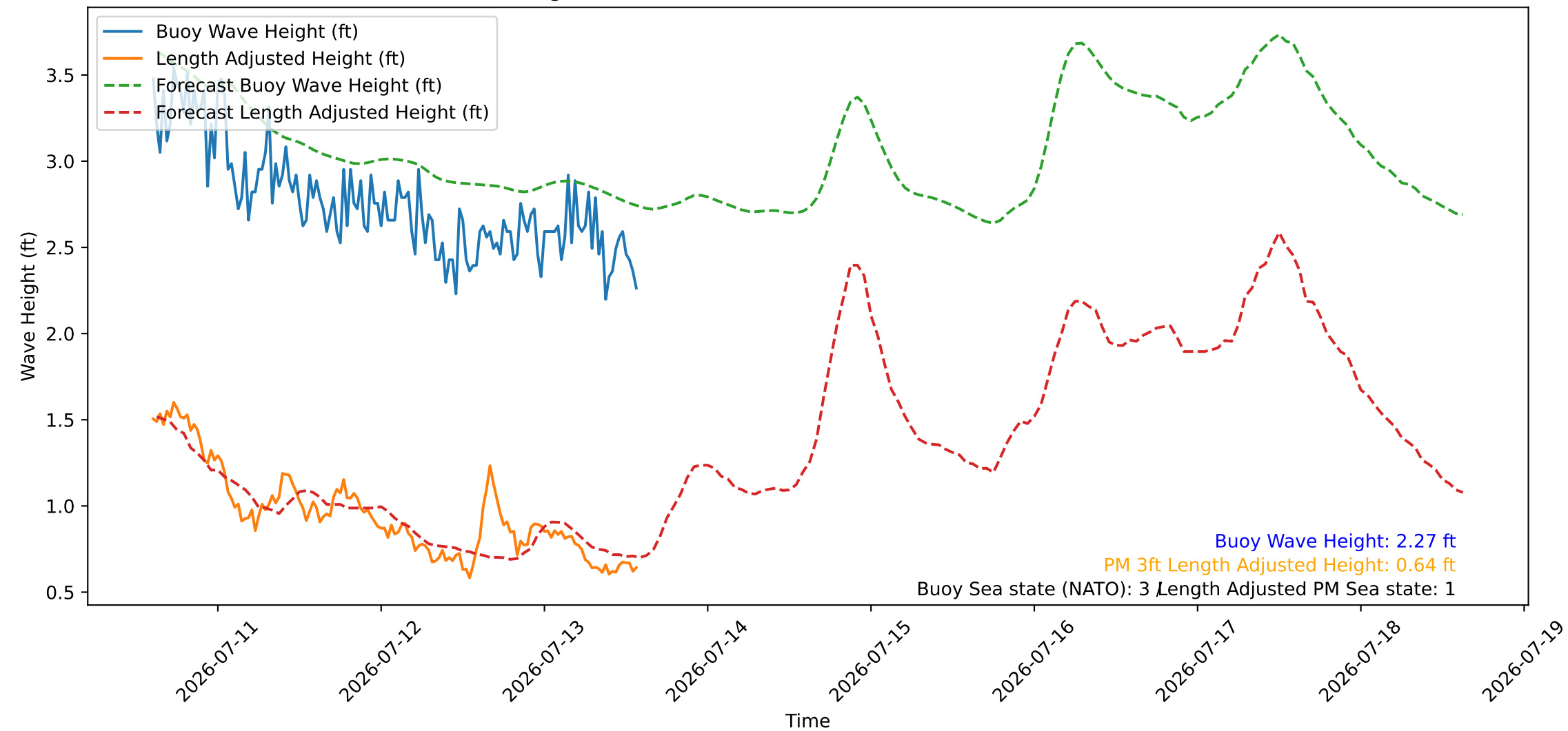
Wave Heights over Time for Green Beach at 2026-07-13 14:31:08
