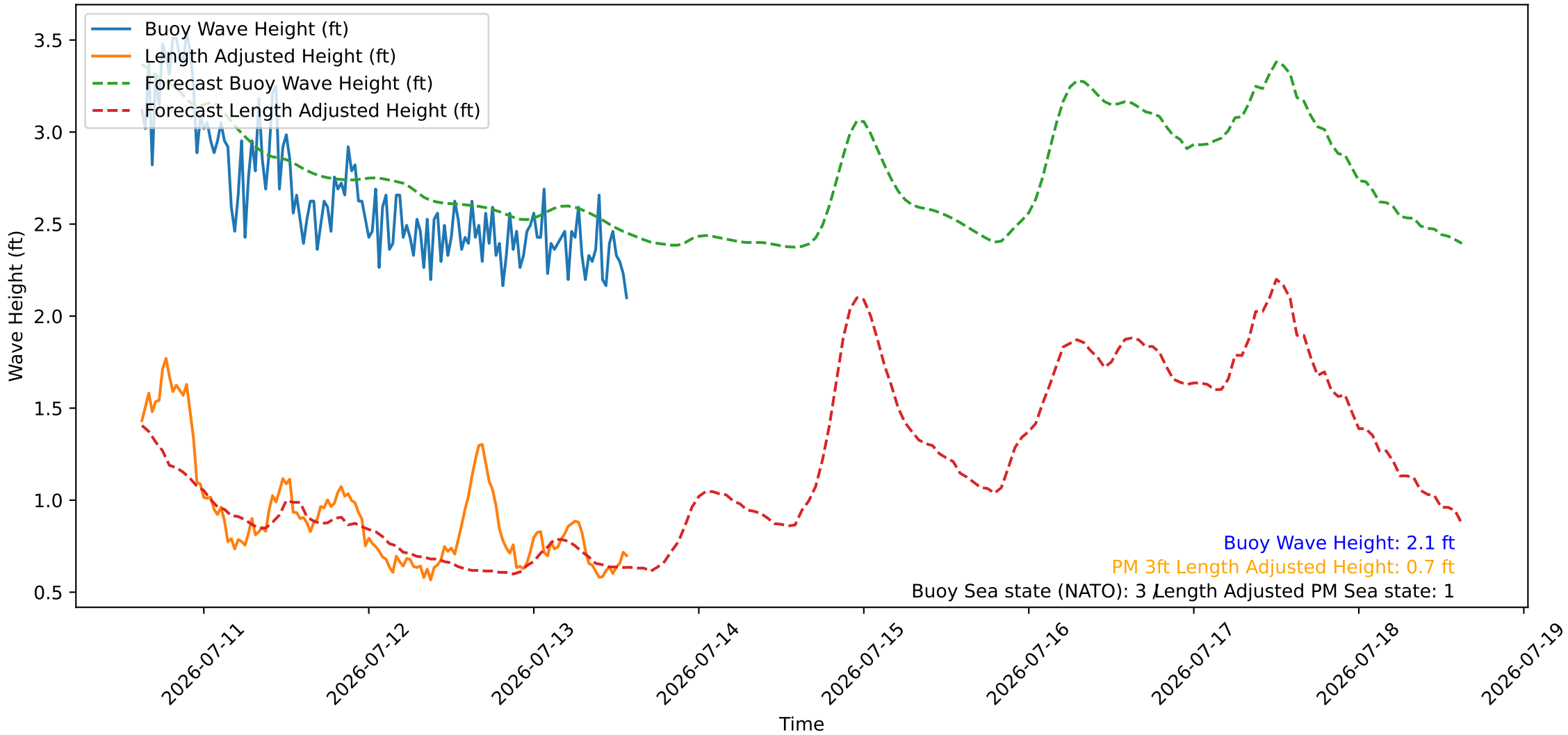
Wave Heights over Time for Red Beach at 2026-07-13 14:30:46
