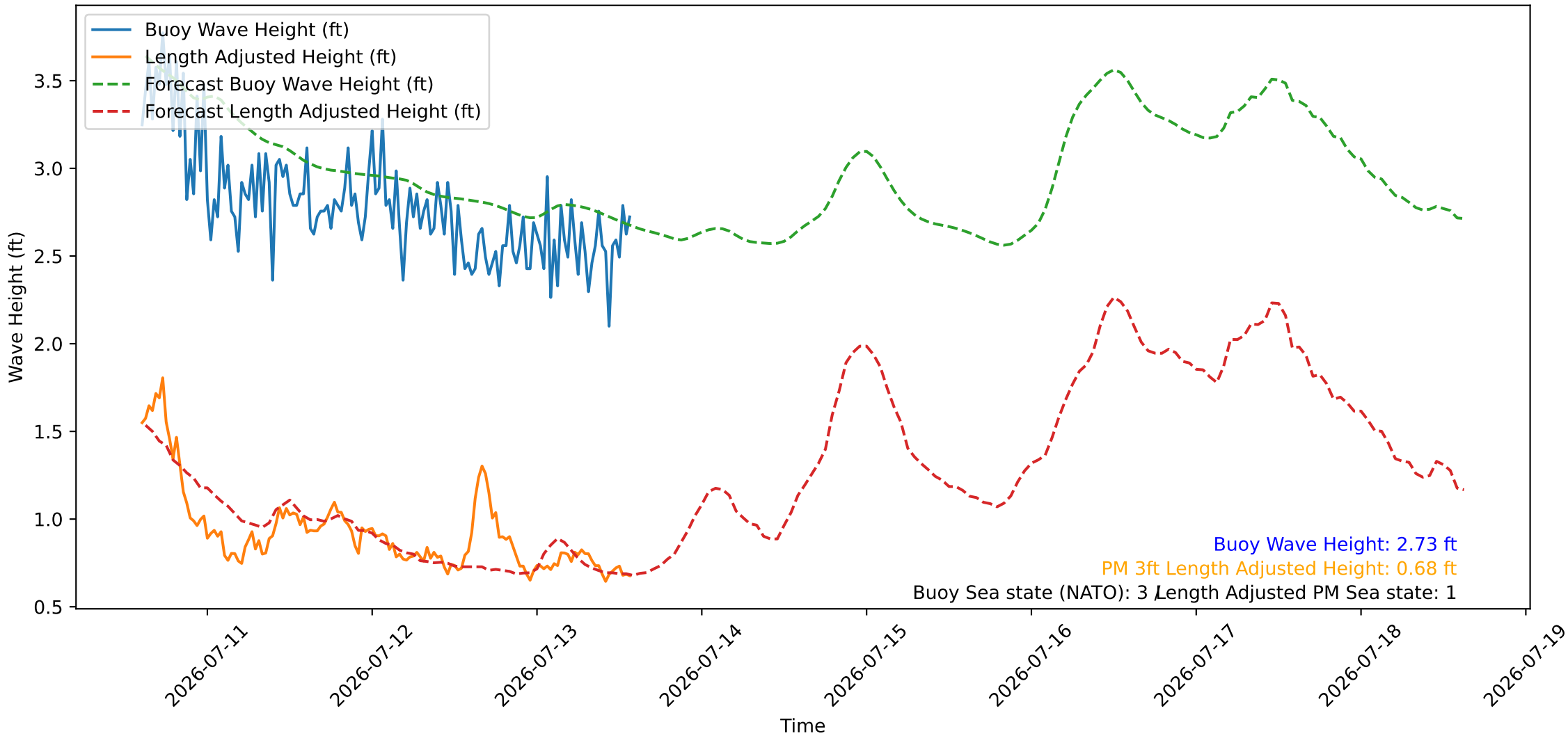
Wave Heights over Time for Oceanside Harbor at 2026-07-13 14:30:26
