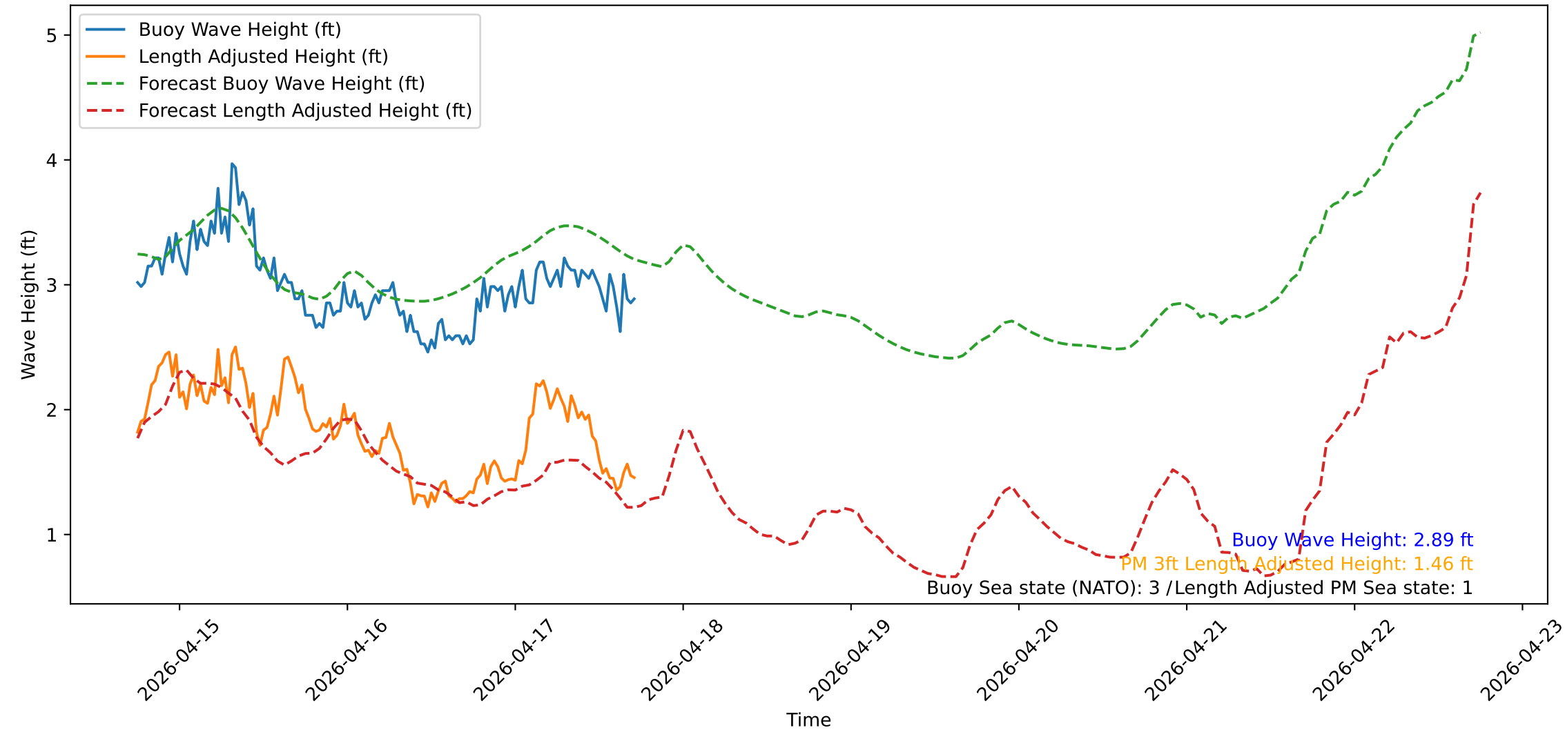
Wave Heights over Time for Green Beach at 2026-04-17 17:51:15
