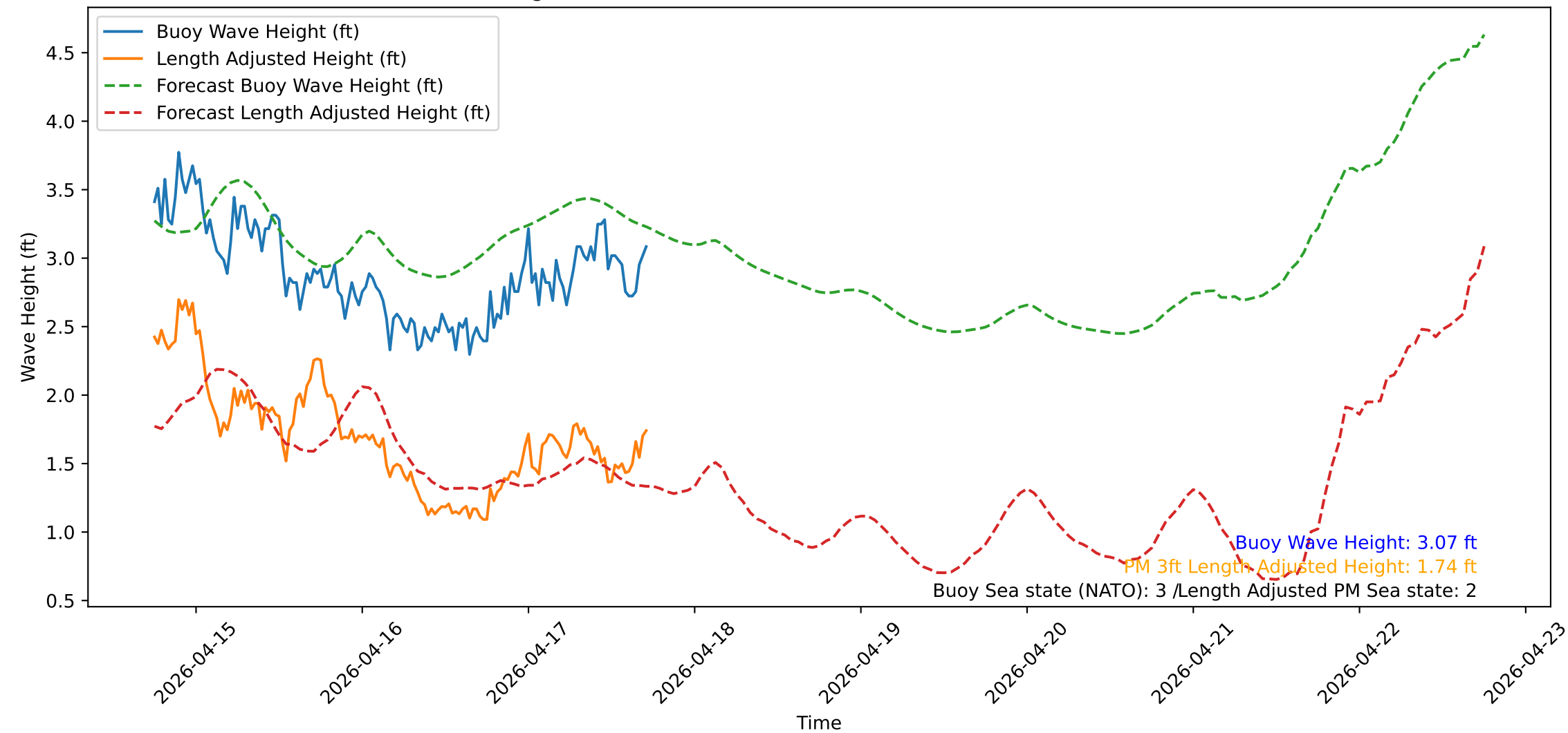
Wave Heights over Time for Oceanside Harbor at 2026-04-17 17:50:32
