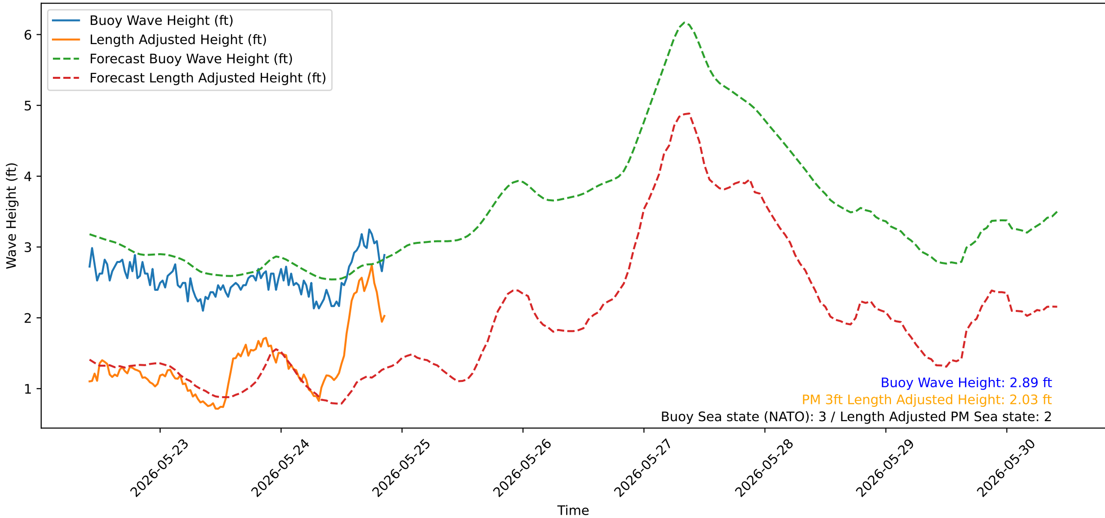
Wave Heights over Time for Oceanside Harbor at 2026-05-25 10:10:30
