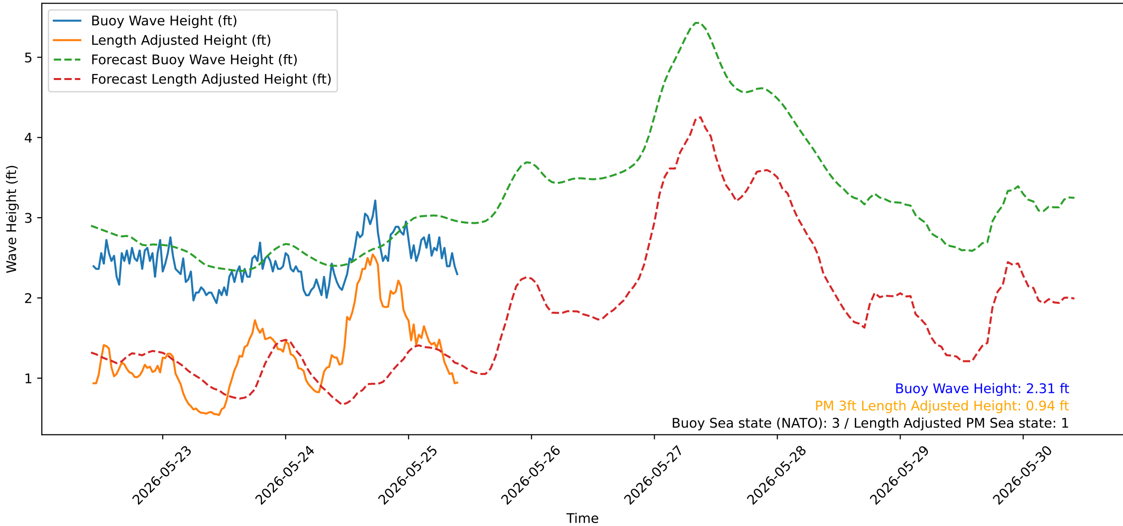
Wave Heights over Time for Red Beach at 2026-05-25 10:10:49
