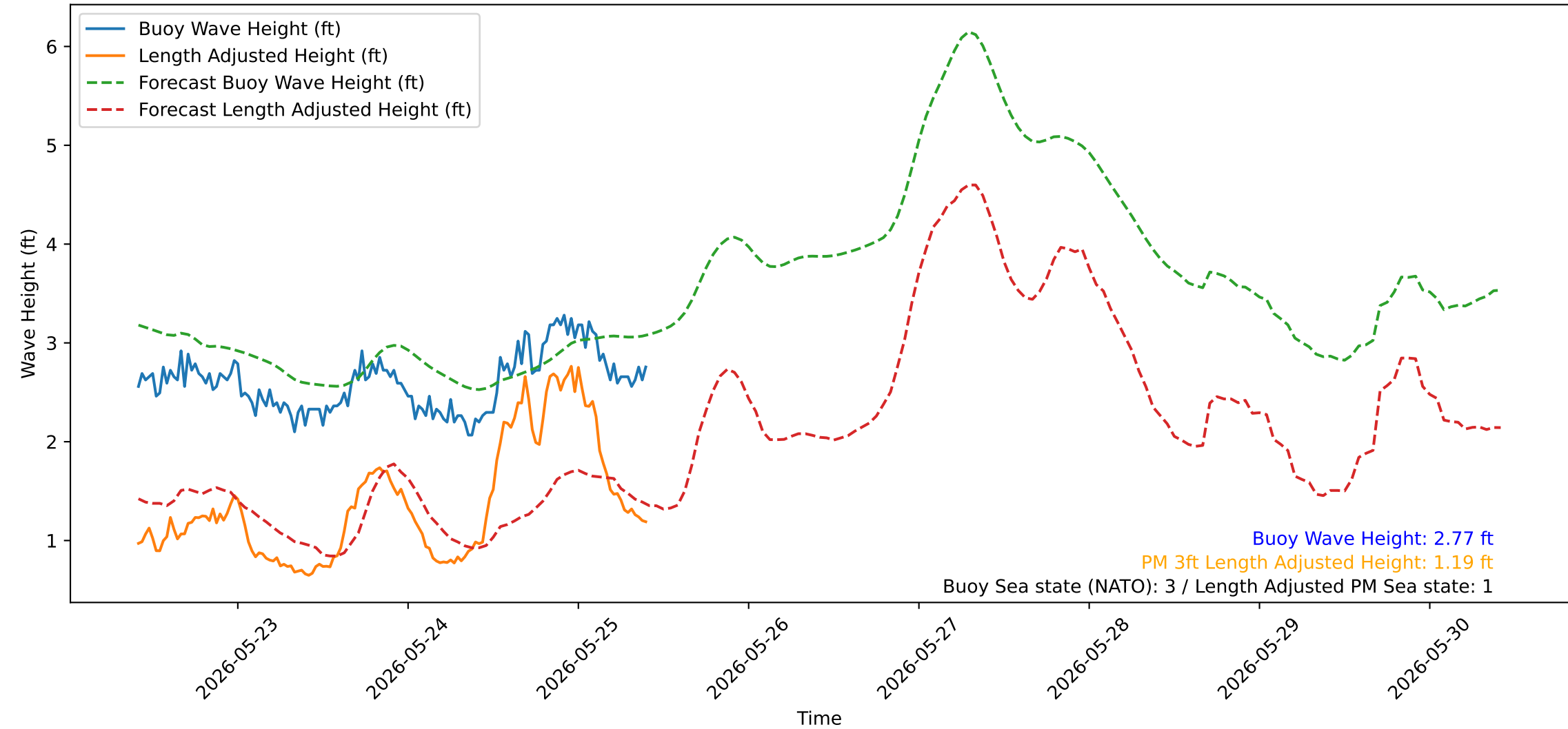
Wave Heights over Time for Green Beach at 2026-05-25 10:11:12
