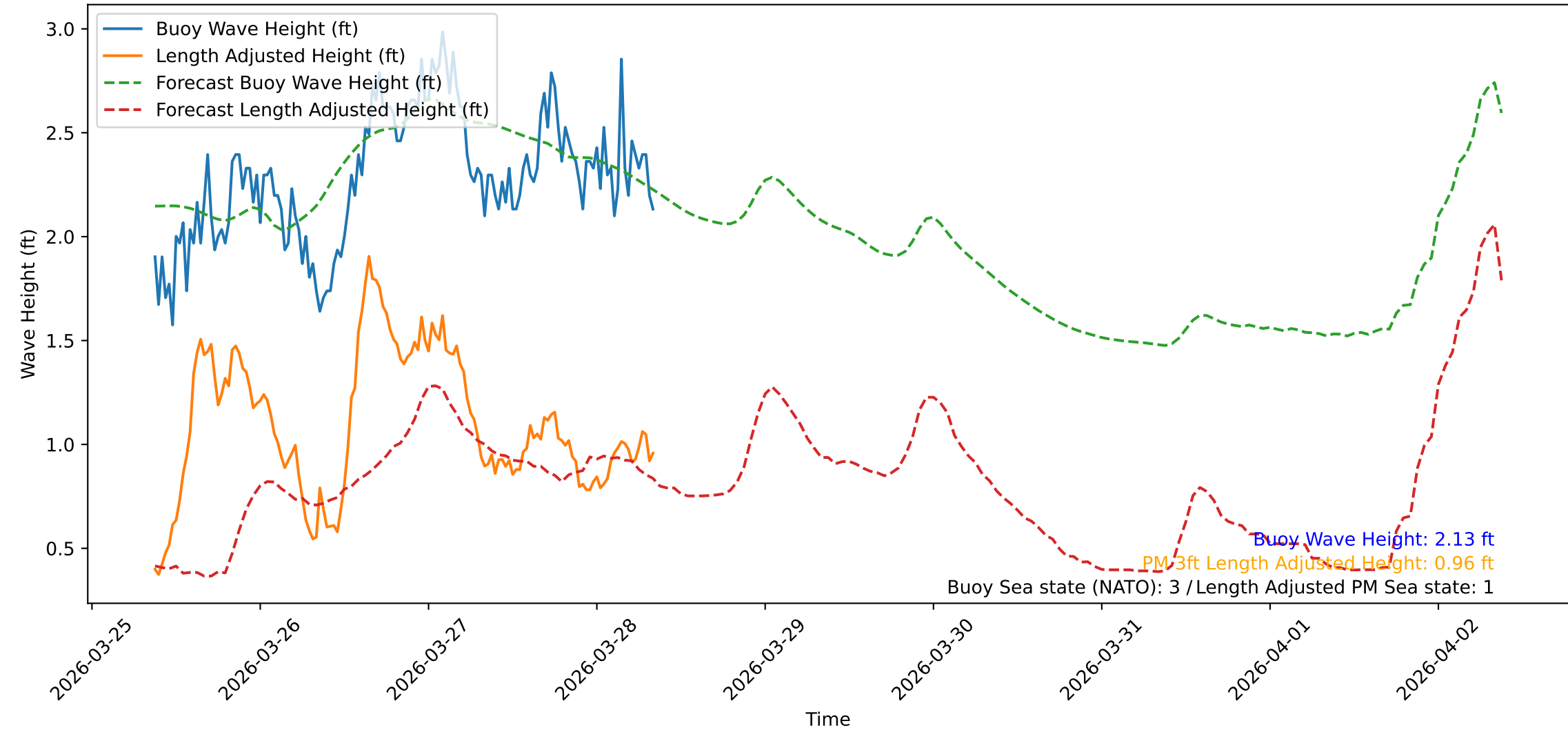
Wave Heights over Time for Red Beach at 2026-03-28 08:50:47
