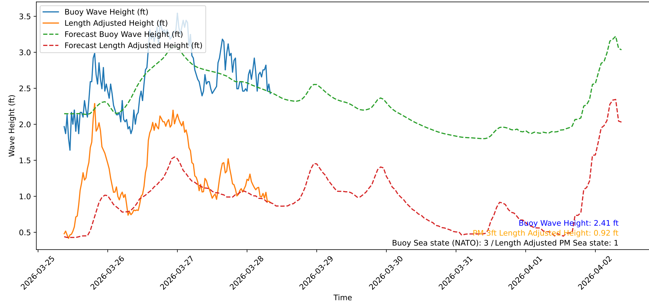
Wave Heights over Time for Green Beach at 2026-03-28 08:51:09
