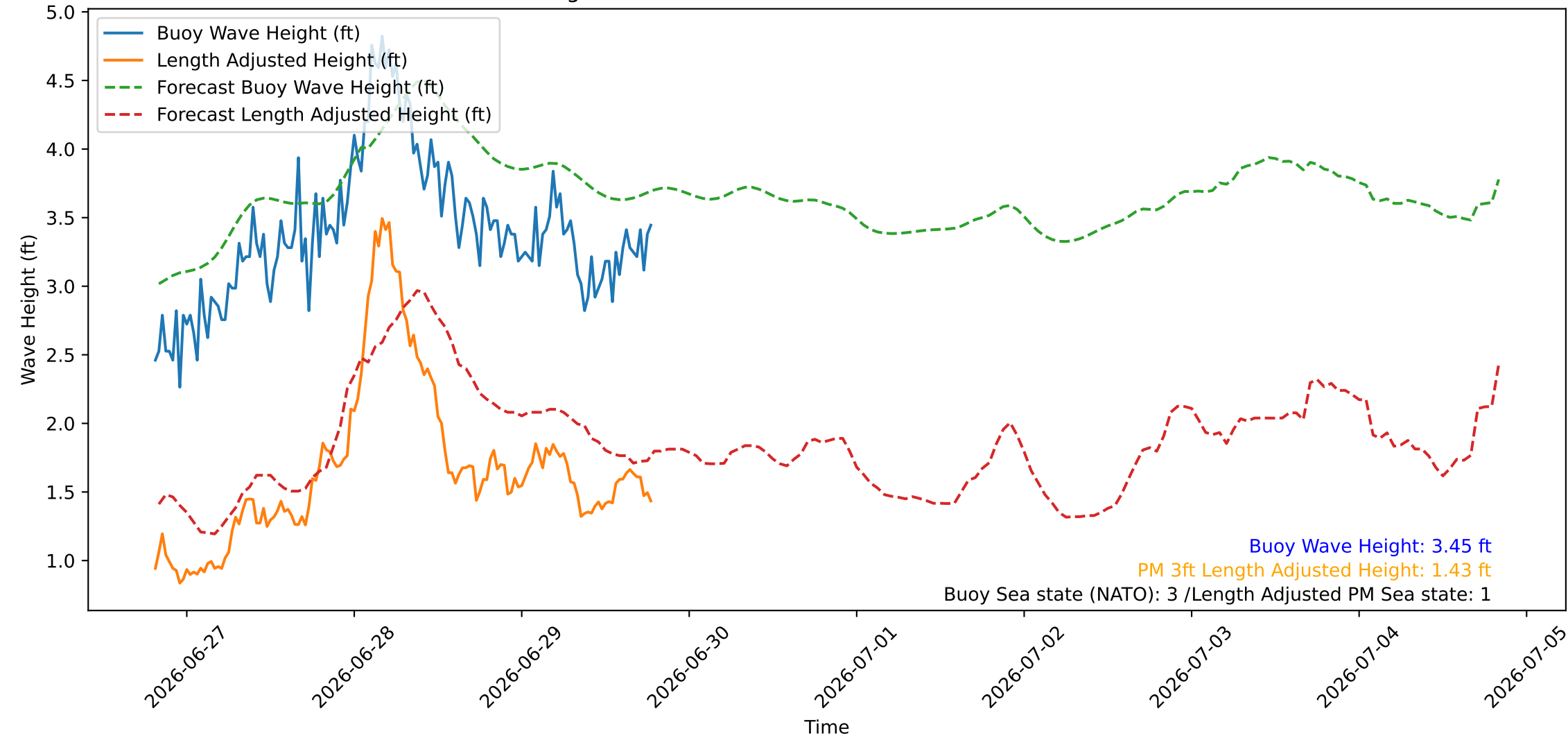
Wave Heights over Time for Green Beach at 2026-06-29 19:31:07
