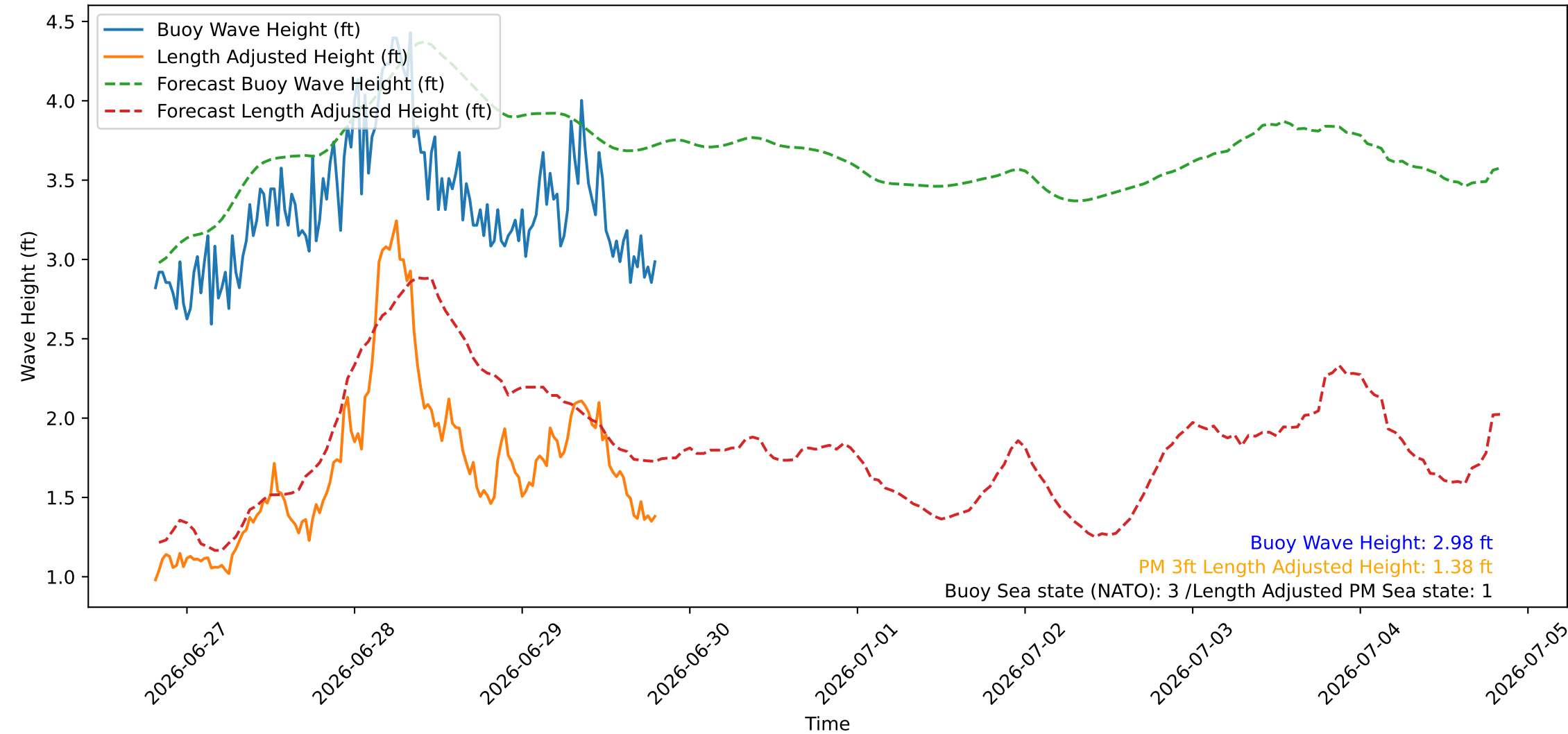
Wave Heights over Time for Oceanside Harbor at 2026-06-29 19:30:26
