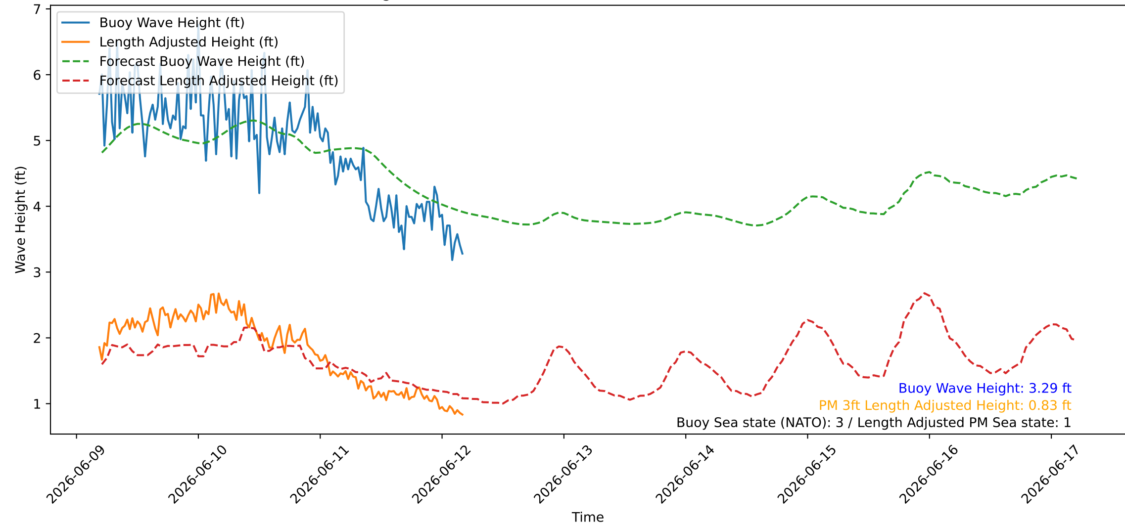
Wave Heights over Time for Oceanside Harbor at 2026-06-12 04:40:26
