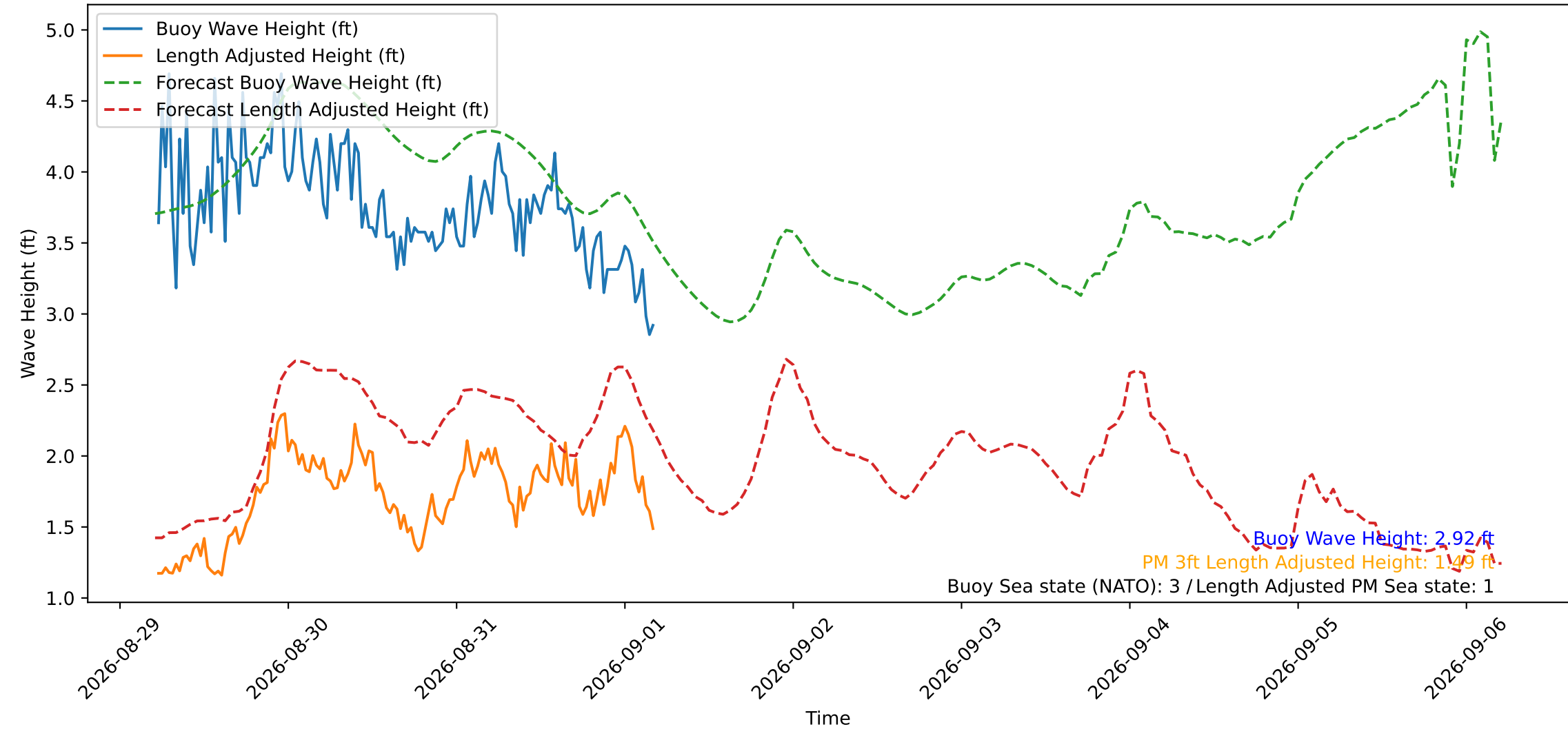
Wave Heights over Time for Red Beach at 2026-09-01 05:00:51
