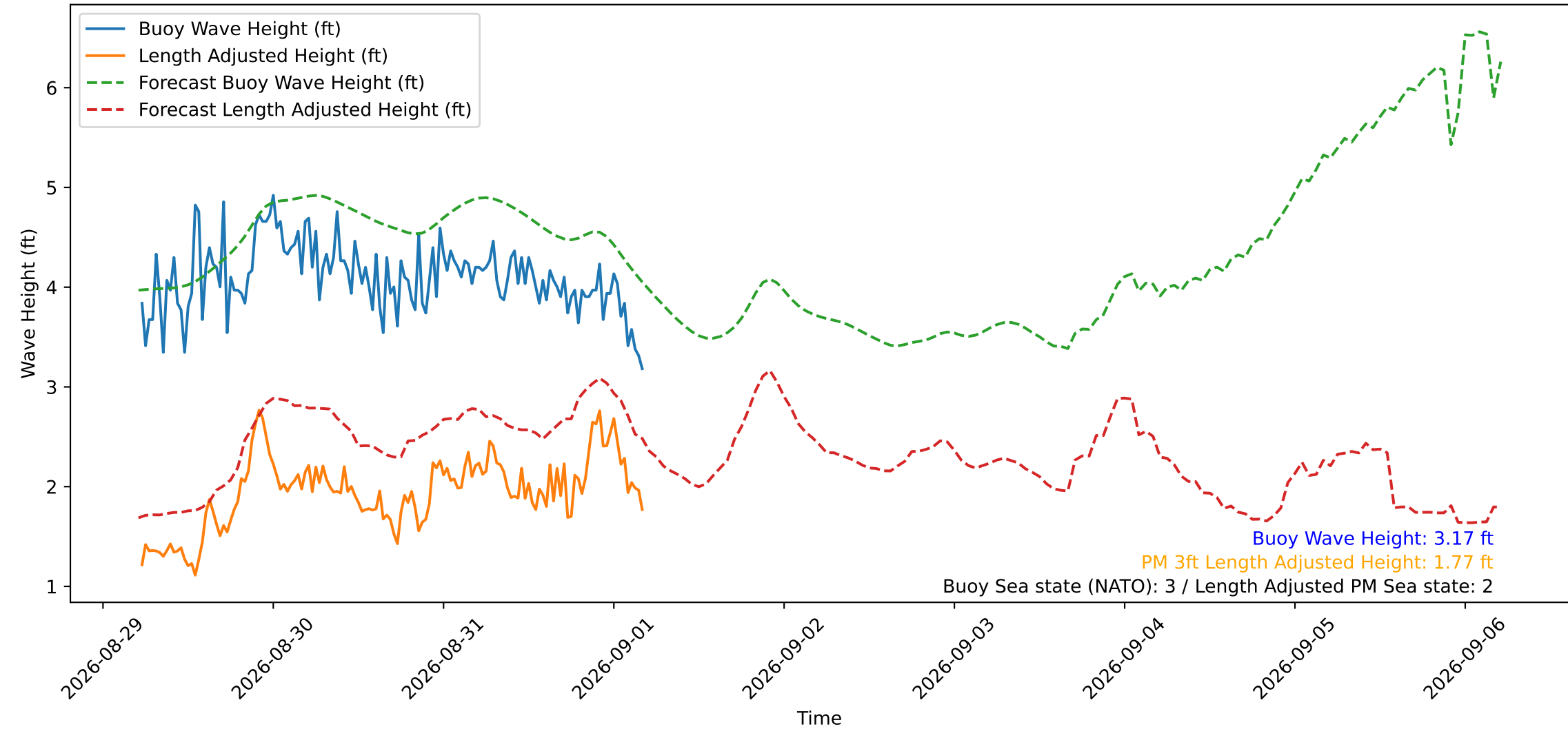
Wave Heights over Time for Green Beach at 2026-09-01 05:01:15
