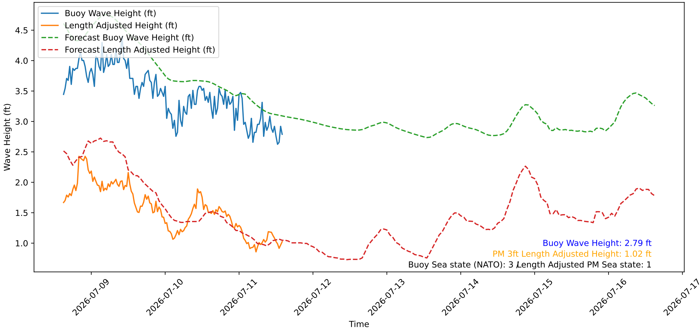
Wave Heights over Time for Green Beach at 2026-07-11 14:51:09
