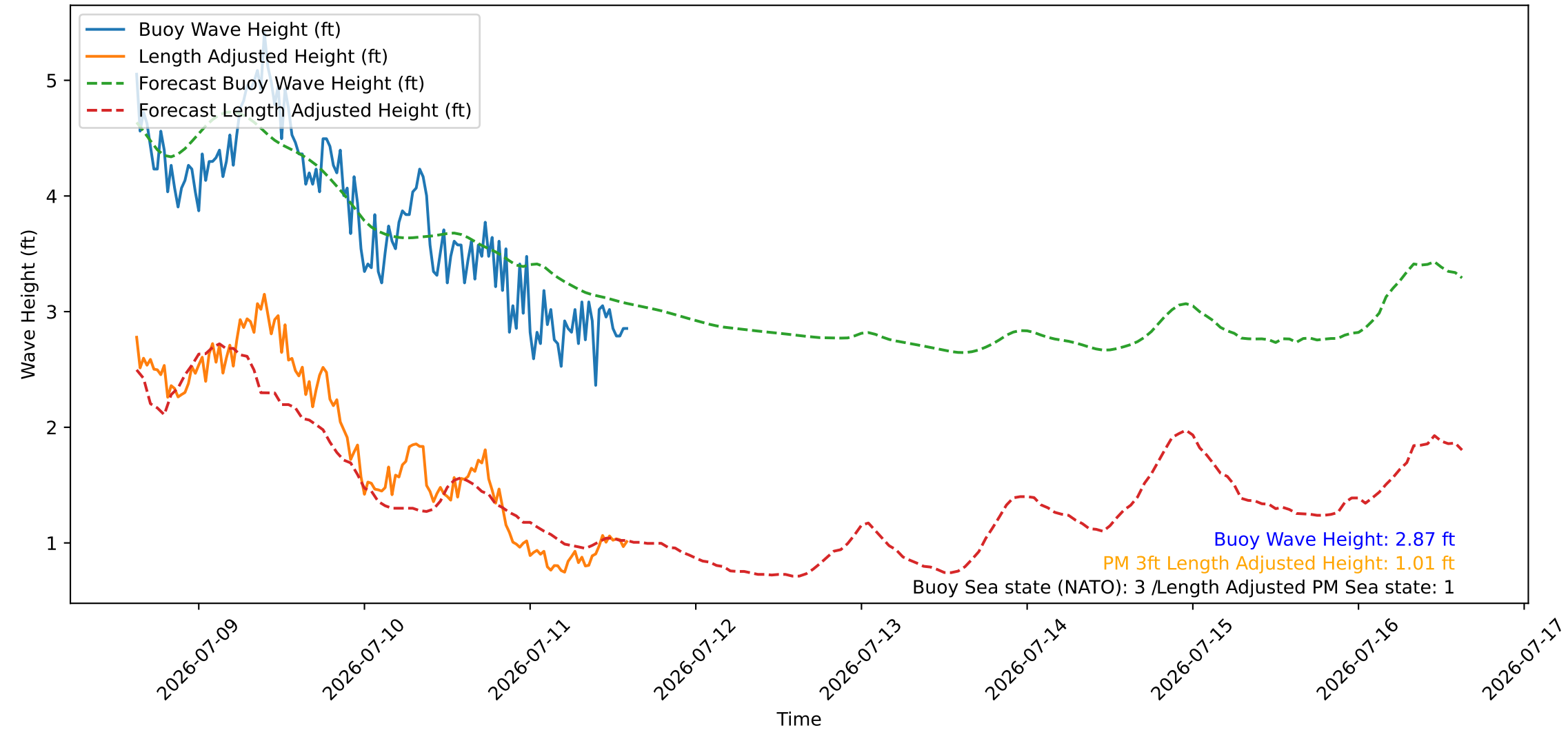
Wave Heights over Time for Oceanside Harbor at 2026-07-11 14:50:26
